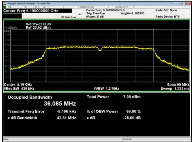
(802.11 ac40) 26dB Bandwidth plot on channel 38
