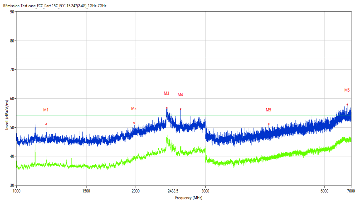
Figure 33: Spurious Emission, 1GHz – 10 th Harmonic, 802.11g, 2437MHz 1GHz-7GHz, Horizontal
