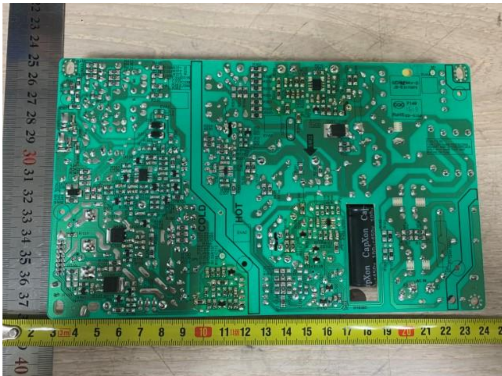
Main board
