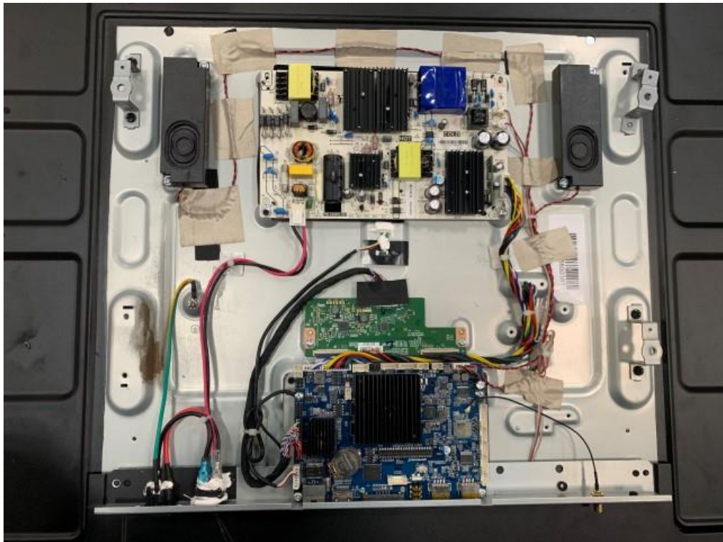
Power board
