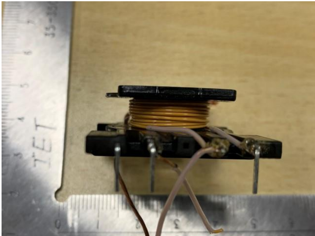
Transformer T101
