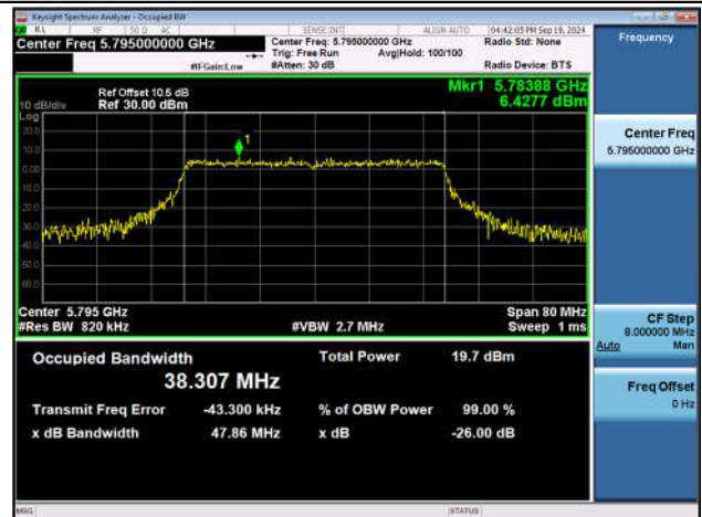
11AX40SISO-Ant1-5795
