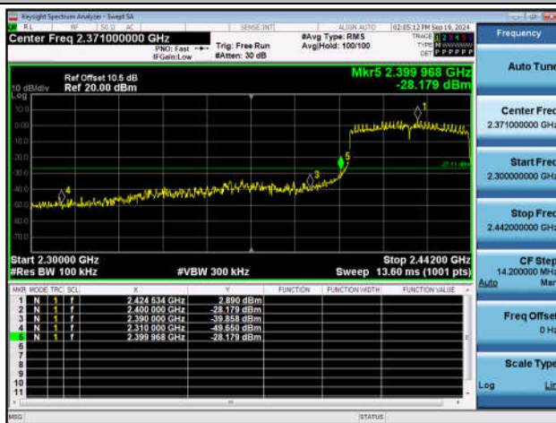
11AX40SISO-Ant1-2422-PASS
