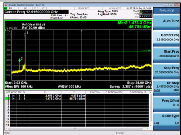
11AX20SISO-Ant1-2462-30~25000-PASS
