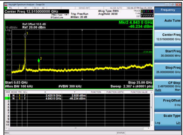
11AX40SISO-Ant1-2437-30~25000-PASS
