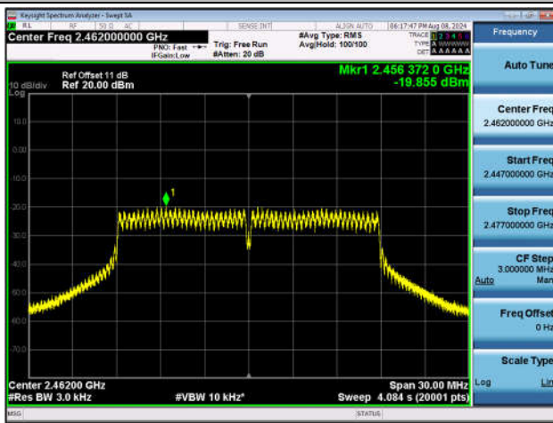
11N20SISO-Ant1-2462-PASS
