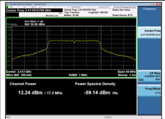
11G-Ant1-2412-PASS
