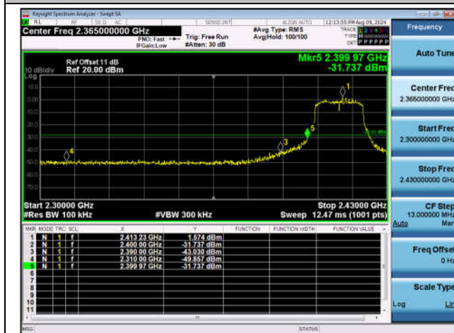
11N20SISO-Ant1-2412-PASS
