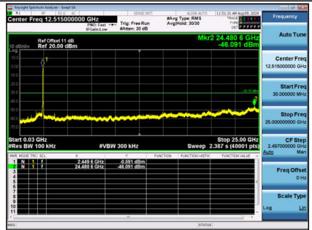
11AX40SISO-Ant1-2452-30~25000-PASS
