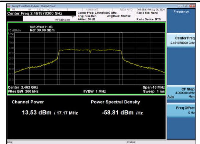
11G-Ant1-2462-PASS
