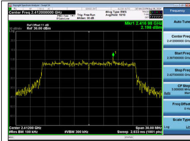
11AX20SISO-Ant1-2412-0~Reference-PASS
