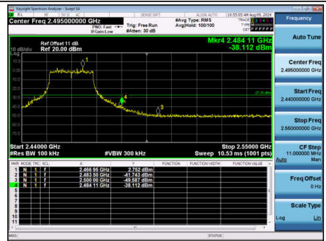
11AX20SISO-Ant1-2462-PASS
