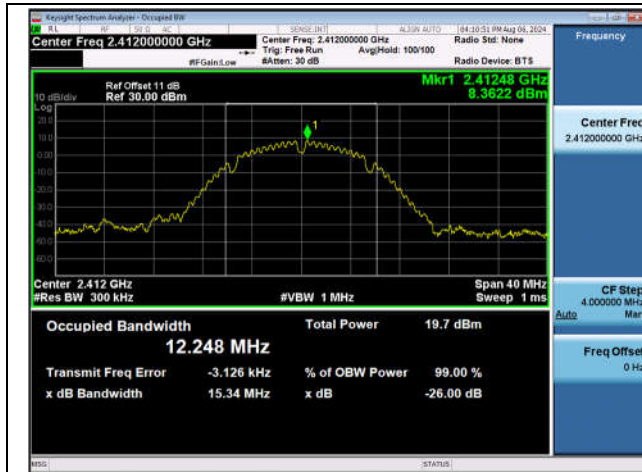
11B-Ant1-2412
