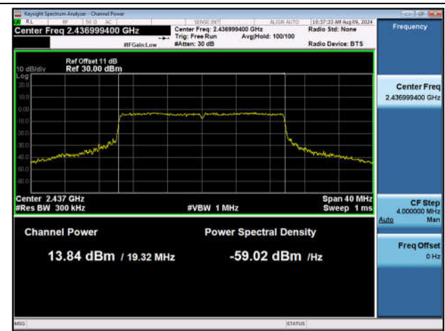
11AX20SISO-Ant1-2437-PASS
