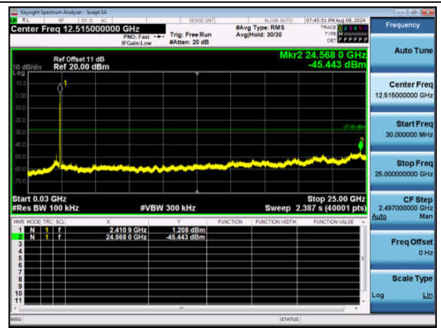
11AX20SISO-Ant1-2412-30~25000-PASS
