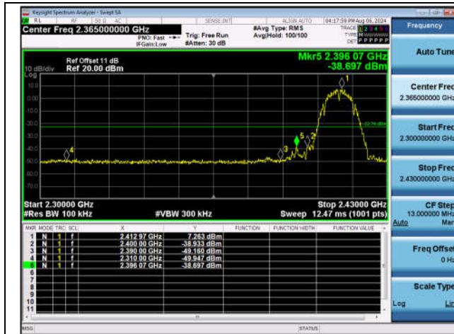
11B-Ant1-2412-PASS
