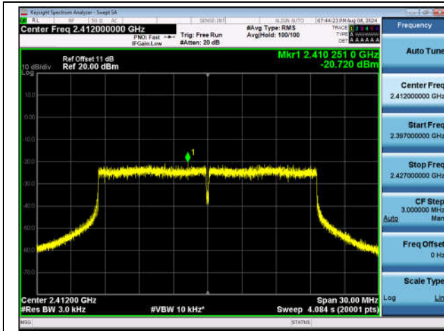
11AX20SISO-Ant1-2412-PASS
