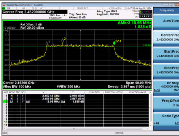
11AX20SISO-Ant1-2462-PASS
