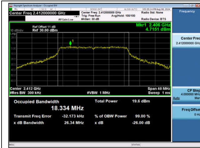
11N20SISO-Ant1-2412
