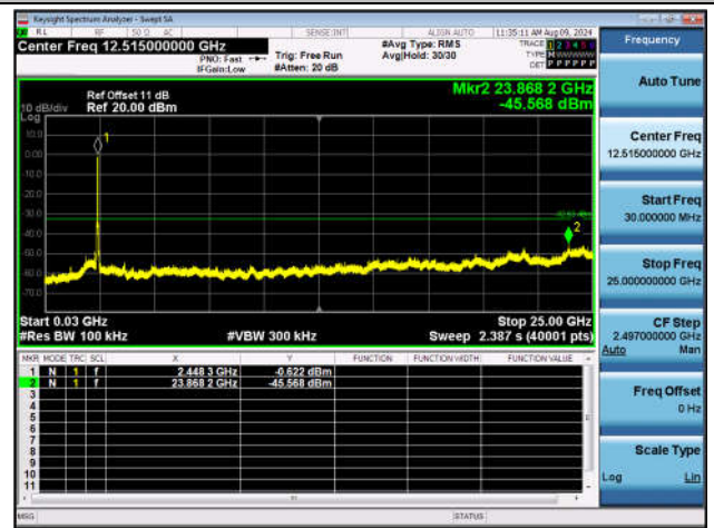
11AX40SISO-Ant1-2437-30~25000-PASS
