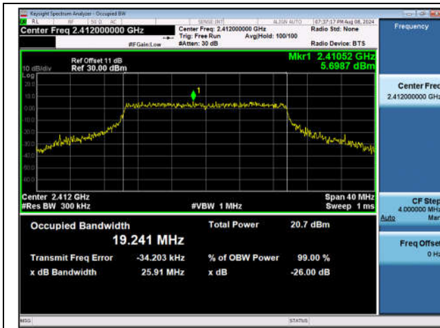
11AX20SISO-Ant1-2412
