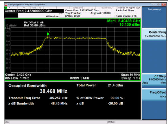
11AX40SISO-Ant1-2422
