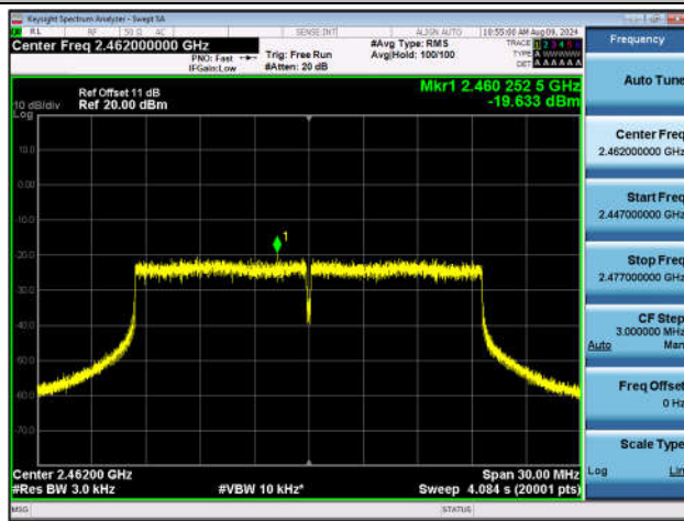
11AX20SISO-Ant1-2462-PASS
