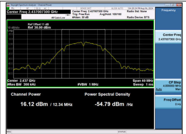
11B-Ant1-2437-PASS
