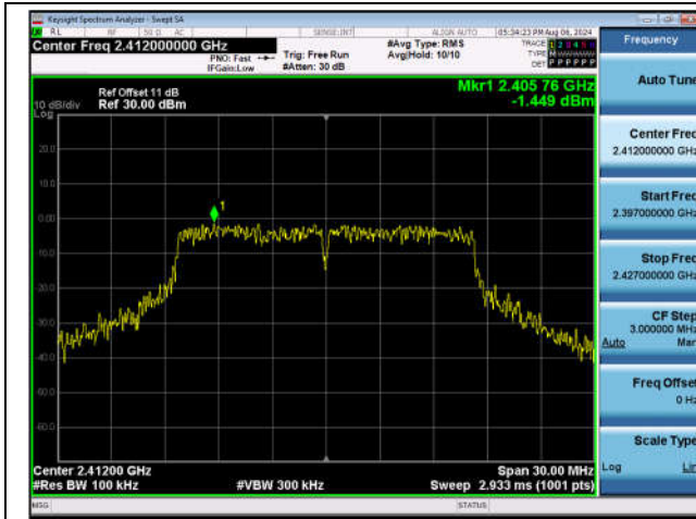
11G-Ant1-2412-0~Reference-PASS
