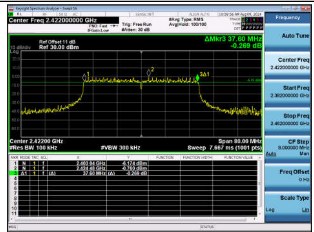
11AX40SISO-Ant1-2422-PASS
