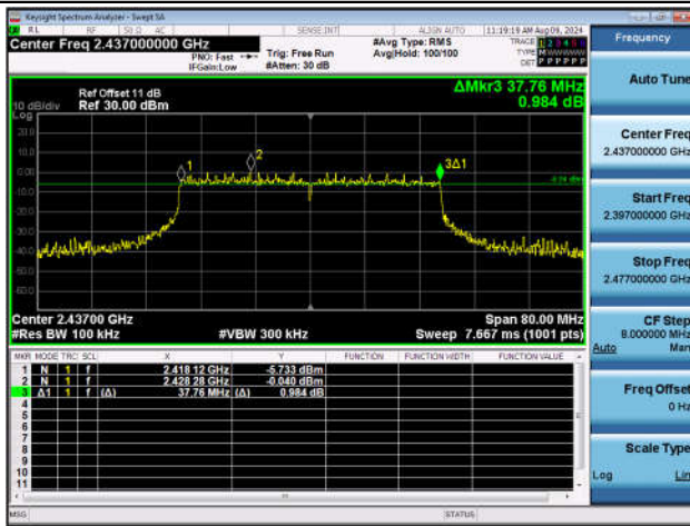
11AX40SISO-Ant1-2437-PASS
