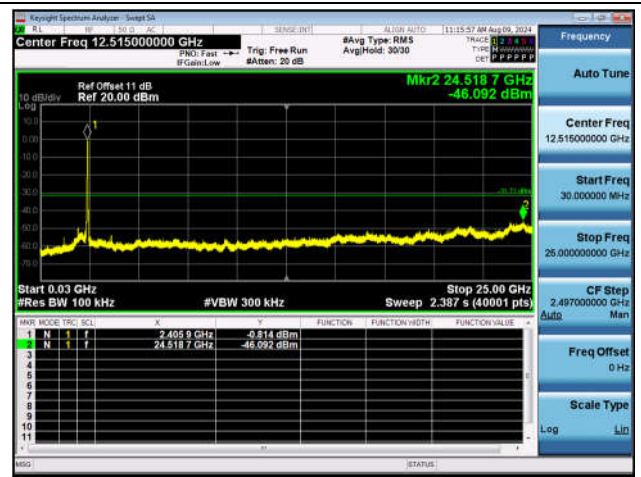
11AX40SISO-Ant1-2422-30~25000-PASS
