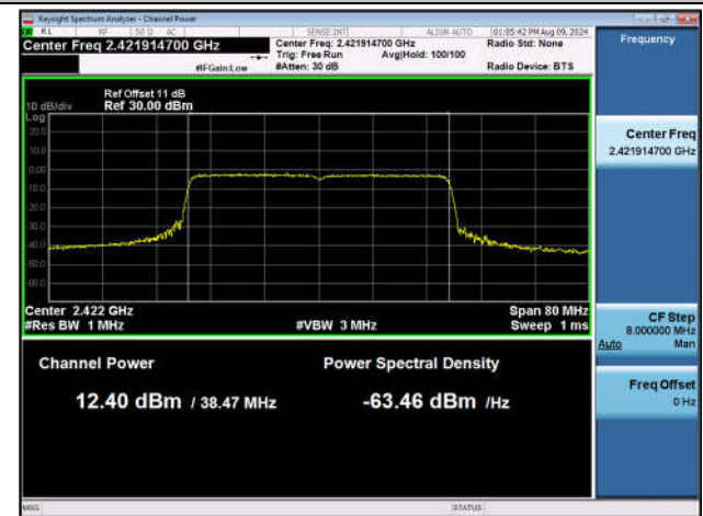
11AX40SISO-Ant1-2422-PASS
