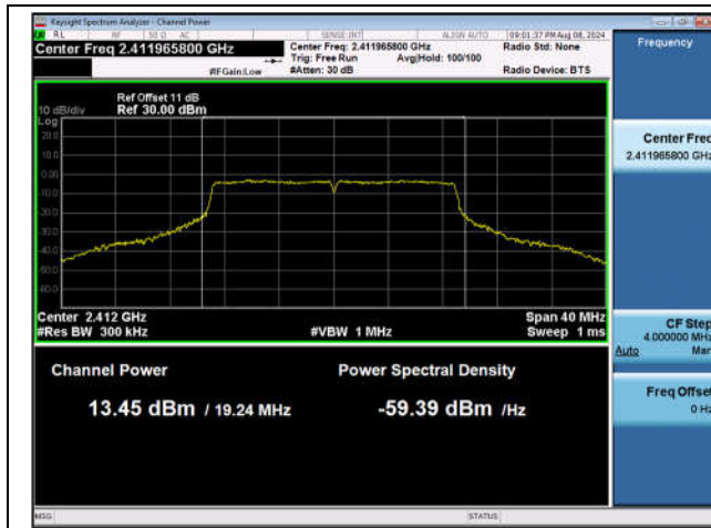
11AX20SISO-Ant1-2412-PASS
