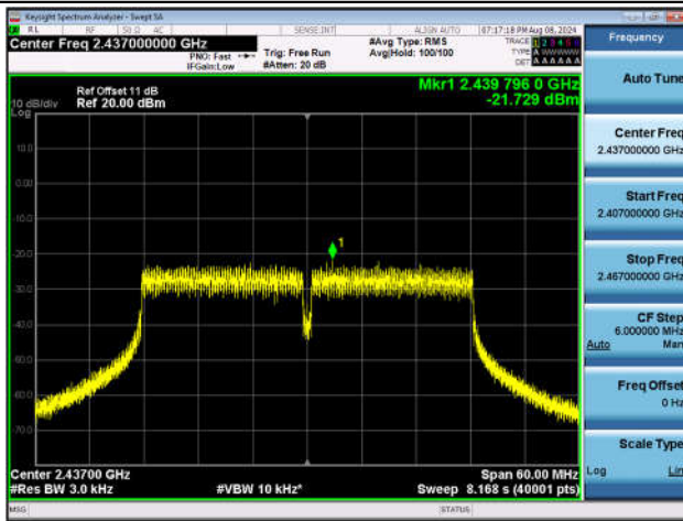
11N40SISO-Ant1-2437-PASS
