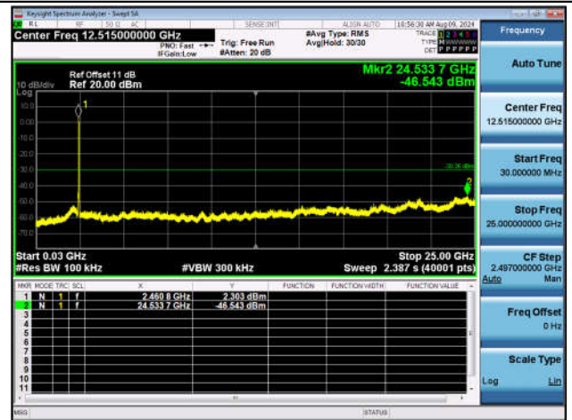
11AX20SISO-Ant1-2462-30~25000-PASS
