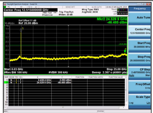
11AX20SISO-Ant1-2437-30~25000-PASS
