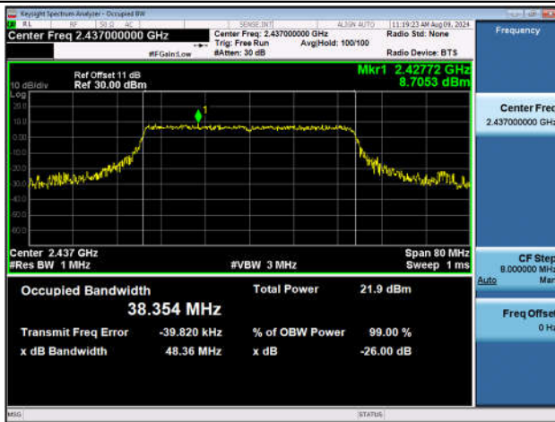
11AX40SISO-Ant1-2437
