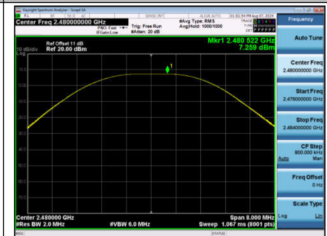
BLE_2M-Ant1-2480-PASS
