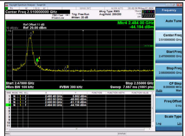
BLE_2M-Ant1-2480-PASS
