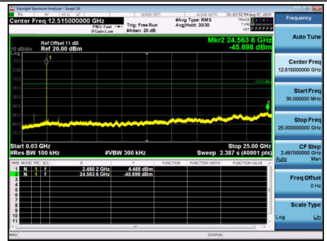
BLE_2M-Ant1-2480-30~25000-PASS
