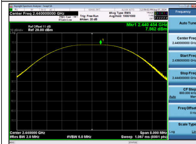
BLE_2M-Ant1-2440-PASS
