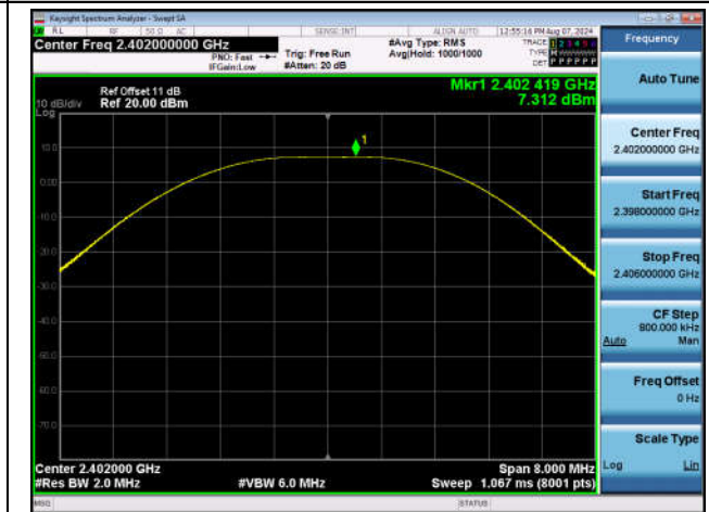
BLE_2M-Ant1-2402-PASS
