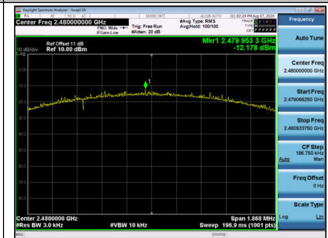
BLE_2M-Ant1-2480-PASS
