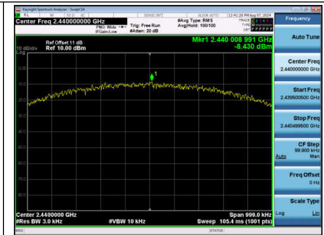
BLE_1M-Ant1-2440-PASS
