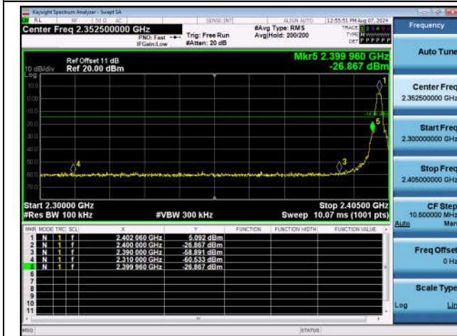
BLE_2M-Ant1-2402-PASS
