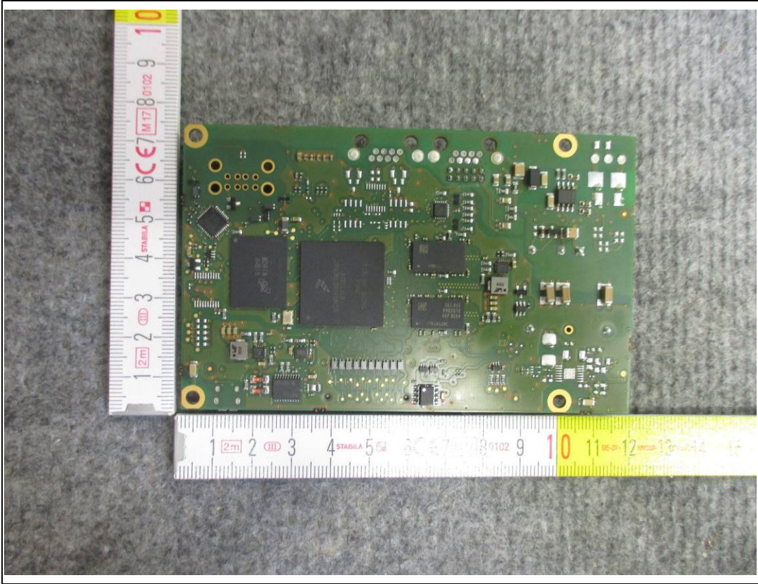
Figure 3: Rear view of Main board of Touch-it CE OEM glass 7
