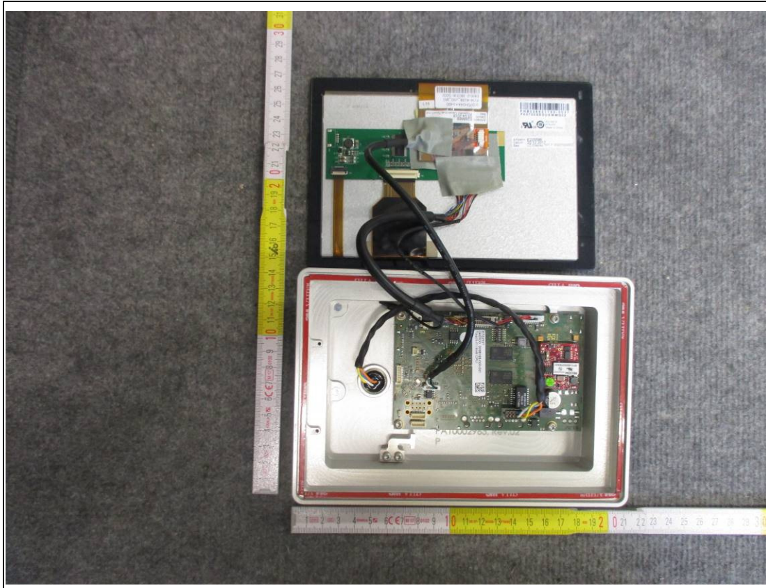
Figure 1: Internal picture of Touch-it CE OEM glass 7
