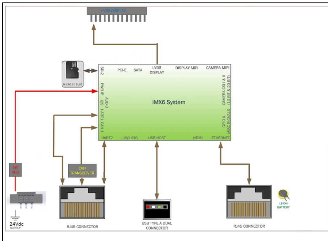
Figure 4-3: Block diagram of function
