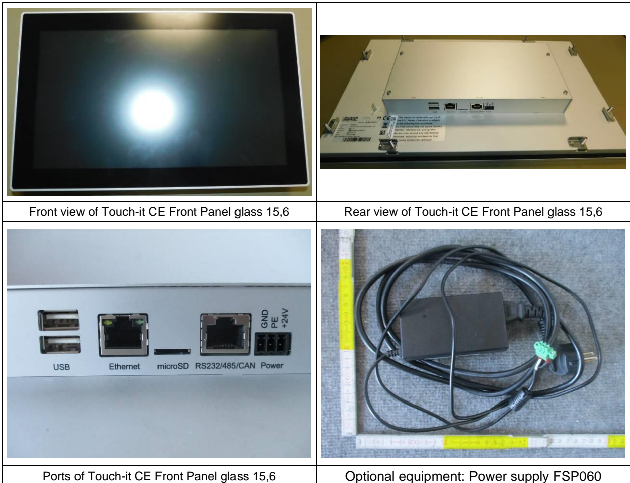
Figure 4-1: Touch-it CE Front Panel glass 15,6 with Power supply
