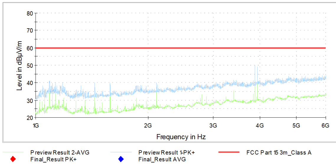
Figure 6-7: Graphical presentation Radiated disturbances 1 GHz to 6 GHz
