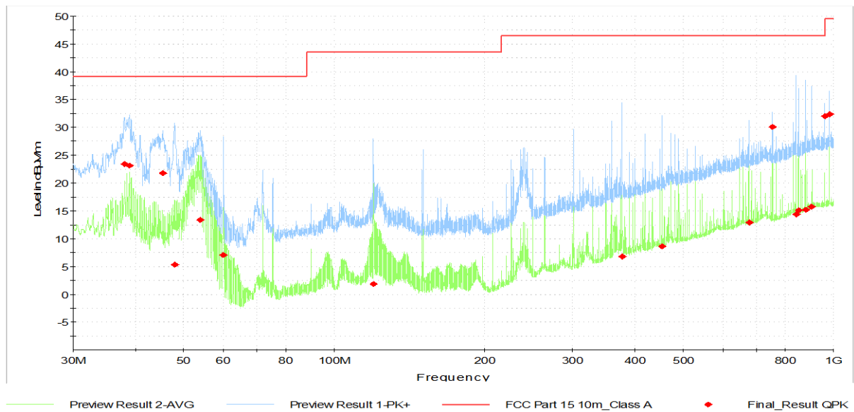
Figure 6-5: Graphical presentation Radiated disturbances 30 MHz to 1000 MHz
