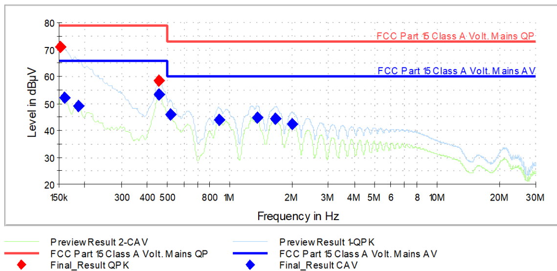
Figure 6-2: Graphical presentation Low voltage AC mains continuous disturbance, Neutral line
