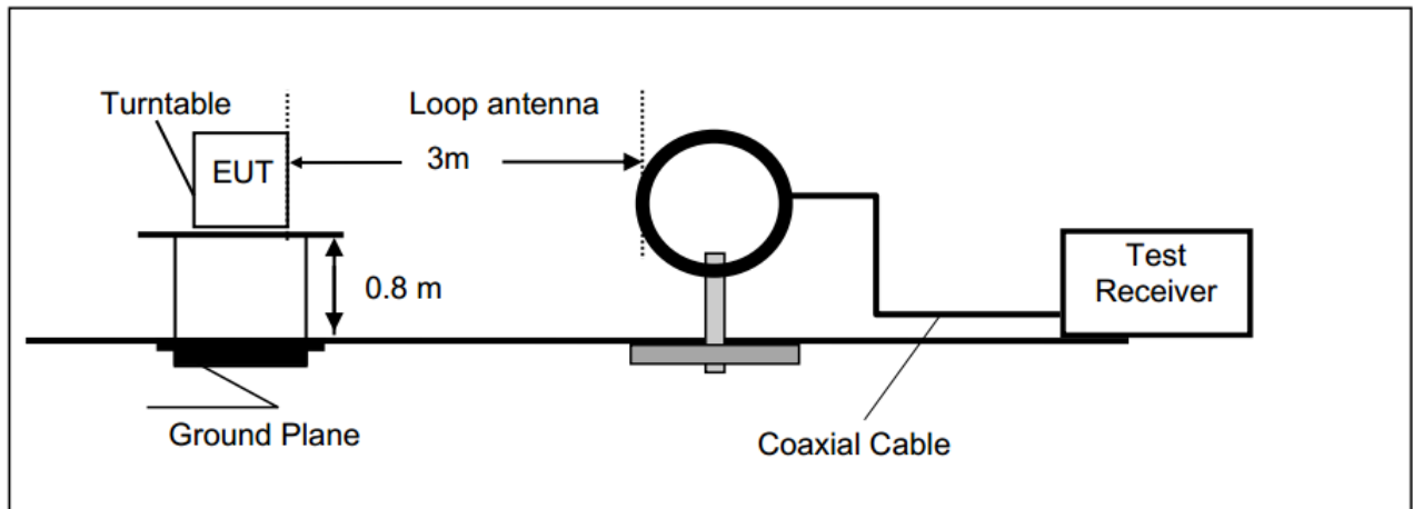
Radiated Emission Test Set-Up, Frequency below 1000MHz
