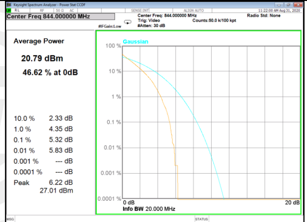
Band5_50_Q16_High
