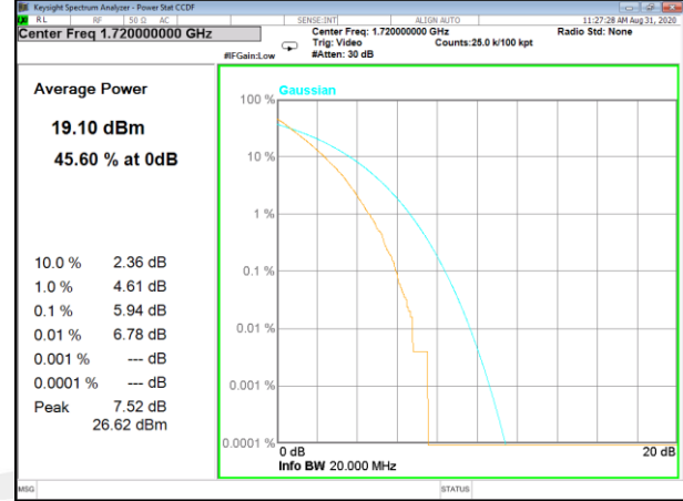
Band4_100_Q16_Low
