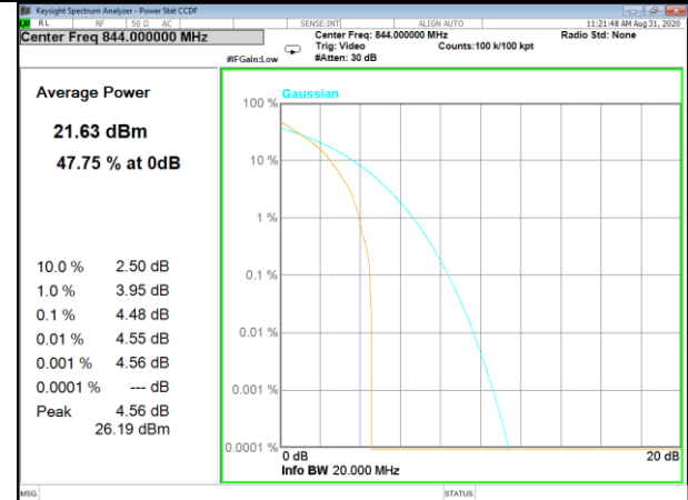
Band5_1_Q16_High
