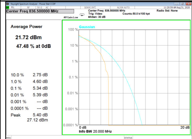
Band5_1_QPSK_Middle
