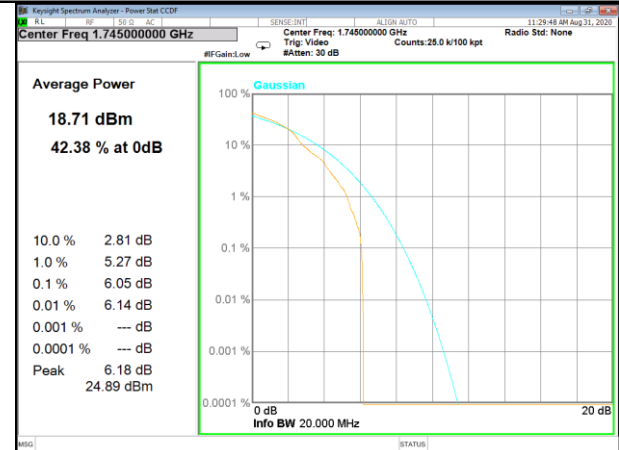
Band4_1_Q16_High
