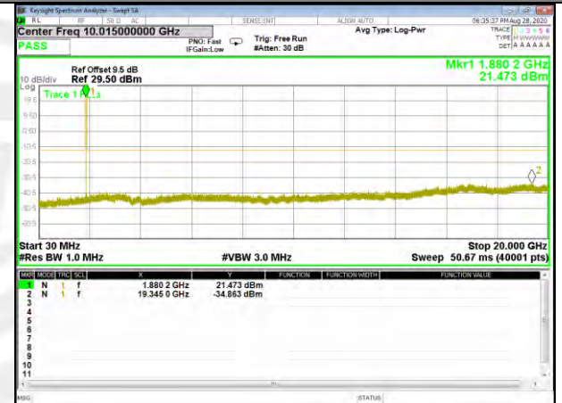
Band2_1.4M_16QAM_High
