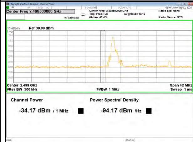
Band7_15M_16QAM_Low_1-RB
