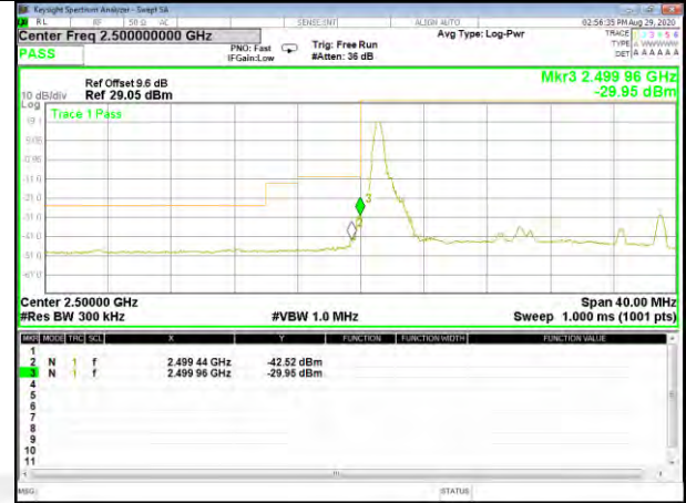
Band7_20M_QPSK_Low_Full-RB
