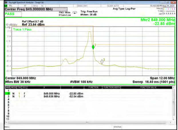
Band5_1.4M_16QAM_High_Full-RB
