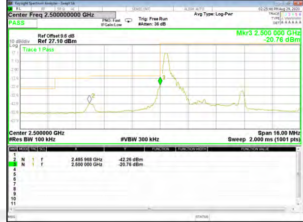
Band7_5M_QPSK_Low_Full-RB
