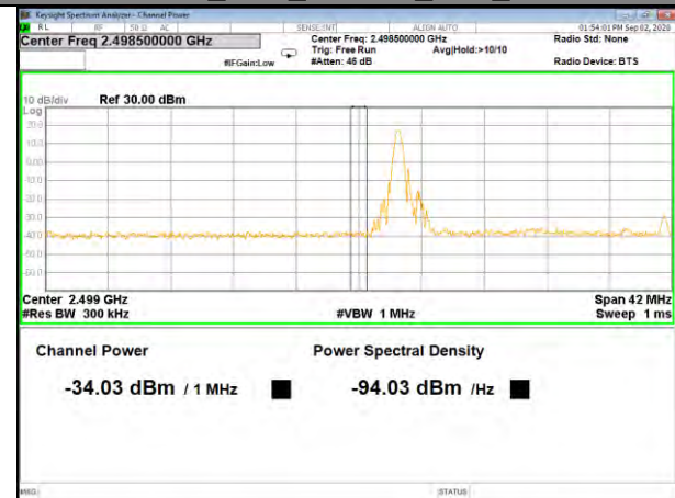
Band7_20M_16QAM_Low_Full-RB
