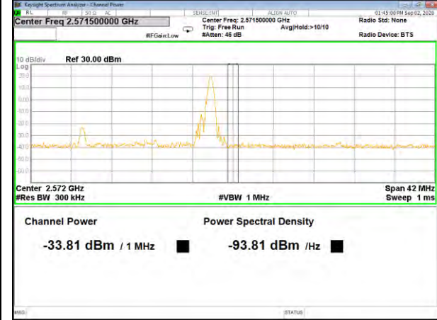
Band7_15M_QPSK_High_Full-RB
