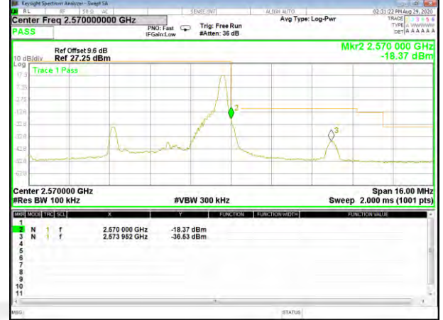
Band7_5M_16QAM_High_Full-RB
