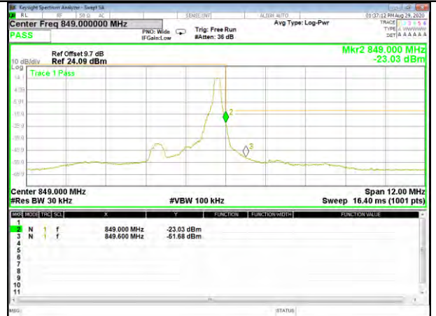
Band5_1.4M_QPSK_High_1-RB
