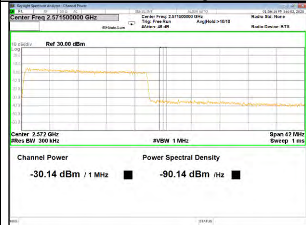
Band7_20M_16QAM_High_Full-RB
