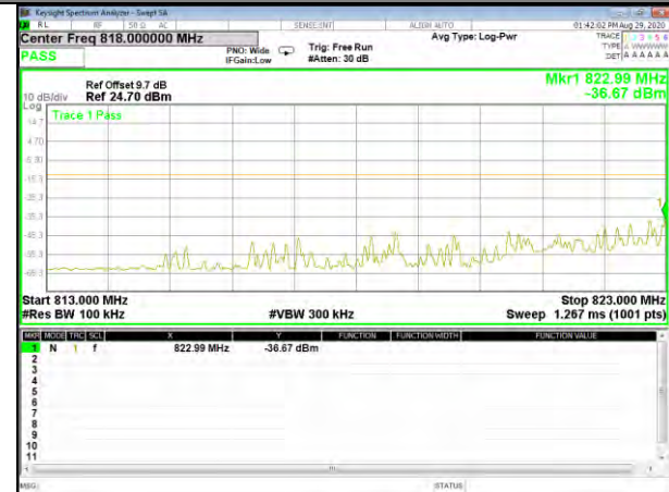
Band5_1.4M_16QAM_Low_Full-RB
