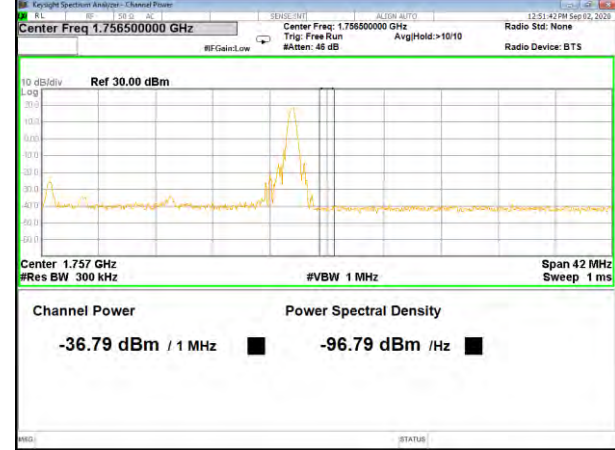
Band4_20M_QPSK_High_Full-RB
