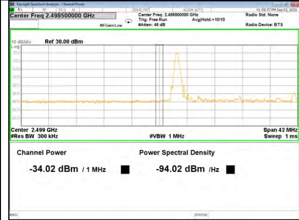
Band7_20M_QPSK_Low_Full-RB
