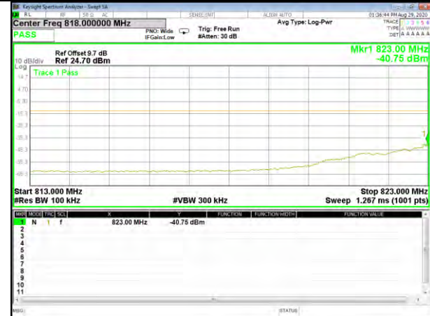
Band5_1.4M_QPSK_High_1-RB
