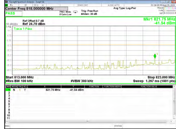
Band5_1.4M_QPSK_Low_Full-RB
