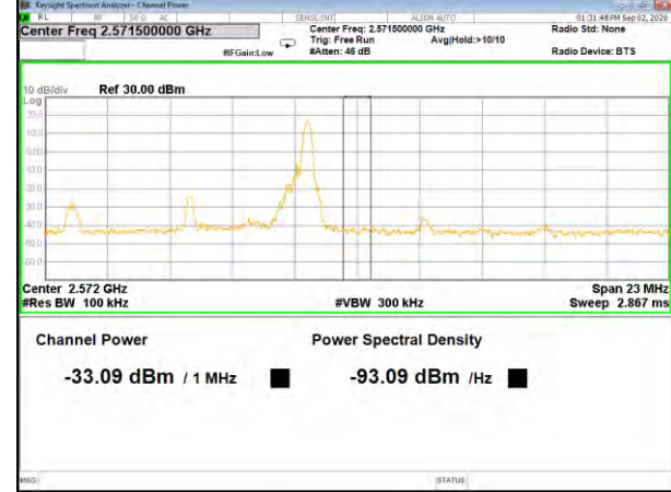
Band7_5M_16QAM_High_Full-RB
