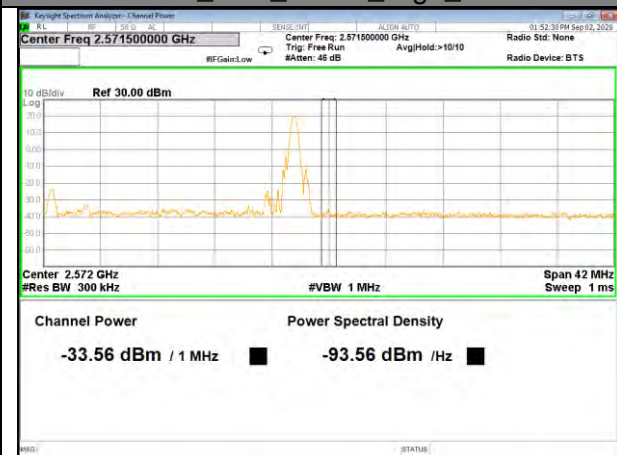
Band7_20M_QPSK_High_1-RB
