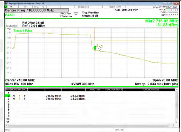
Band17_10M_16QAM_High_Full-RB
