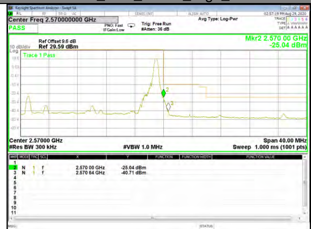
Band7_20M_QPSK_High_1-RB
