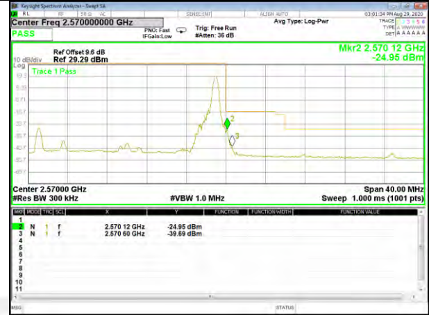
Band7_20M_16QAM_High_Full-RB
