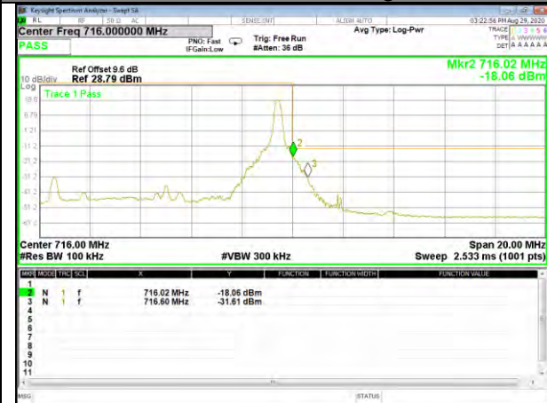
Band17_10M_16QAM_High_1-RB
