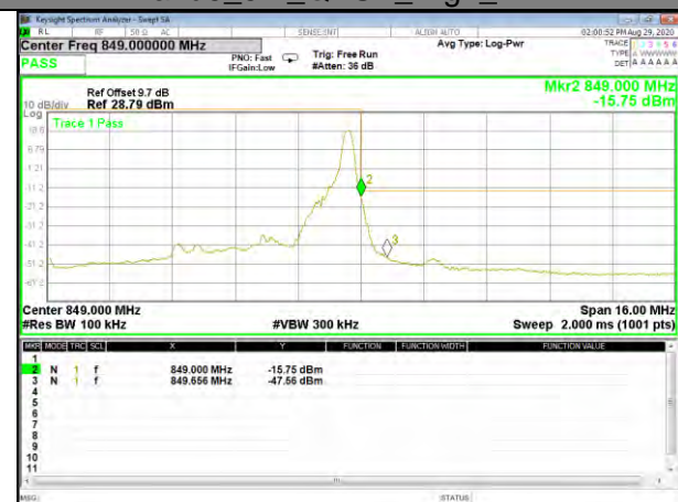
Band5_5M_QPSK_High_1-RB
