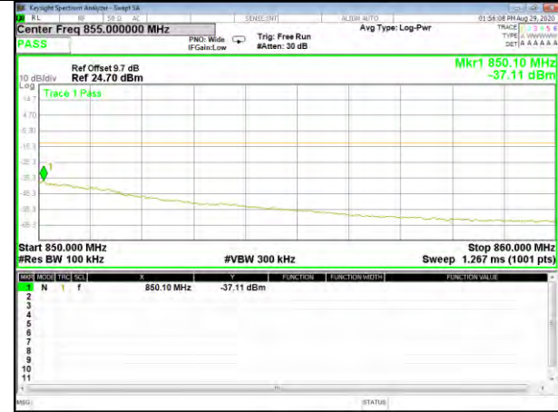
Band5_5M_QPSK_Low_1-RB
