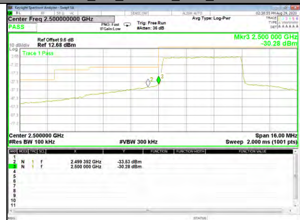
Band7_5M_16QAM_Low_Full-RB
