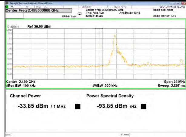
Band7_10M_QPSK_Low_1-RB
