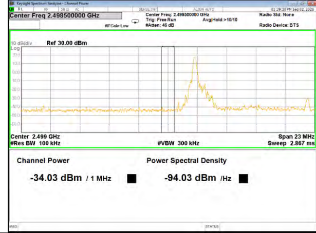
Band7_10M_16QAM_Low_Full-RB
