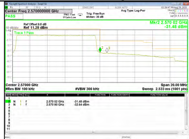
Band7_10M_QPSK_High_Full-RB
