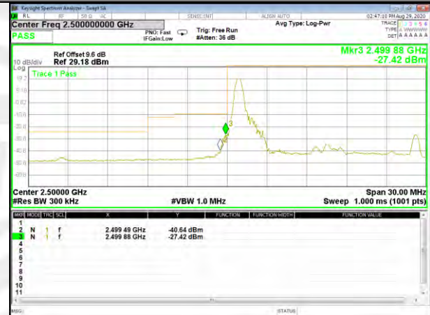
Band7_15M_QPSK_Low_Full-RB
