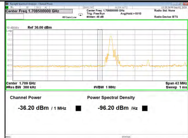
Band4_20M_16QAM_Low_1-RB
