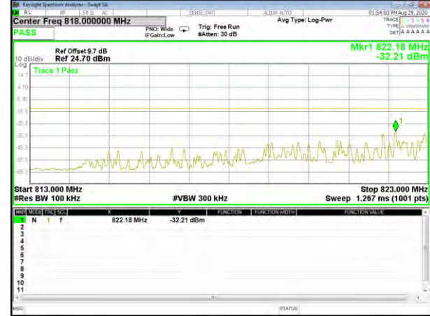
Band5_3M_16QAM_Low_Full-RB
