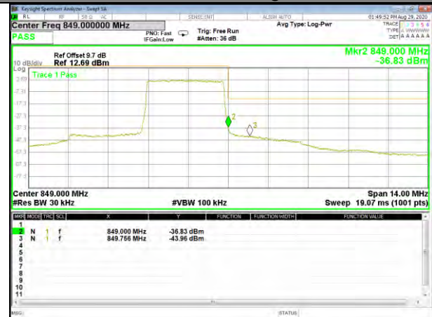
Band5_3M_QPSK_High_Full-RB
