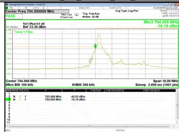
Band17_5M_16QAM_Low_1-RB
