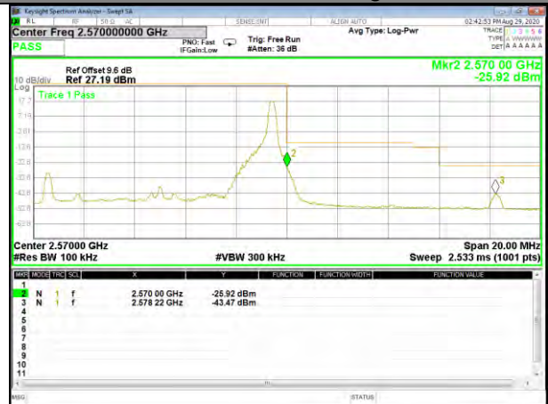
Band7_10M_16QAM_High_1-RB
