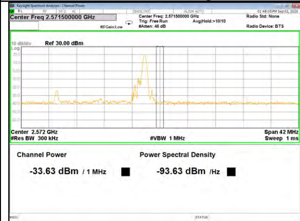
Band7_15M_16QAM_High_Full-RB
