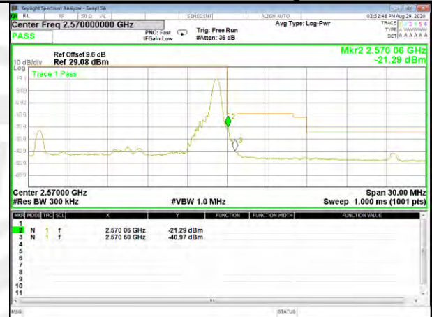
Band7_15M_16QAM_High_Full-RB
