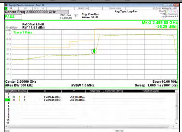
Band7_20M_16QAM_Low_Full-RB
