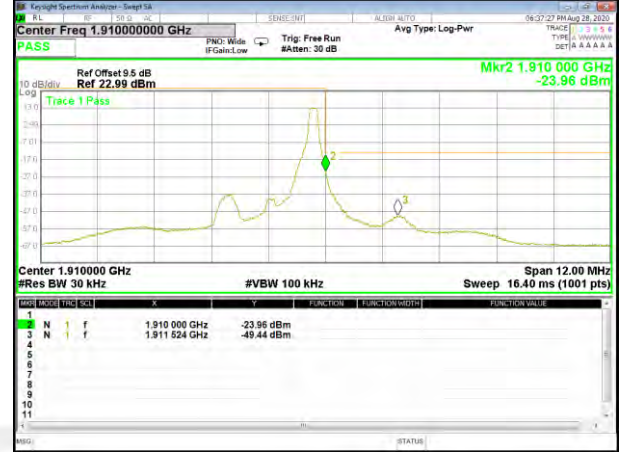
Band2_1.4M_16QAM_High_Full-RB
