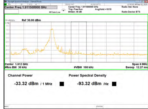
Band2_1.4M_16QAM_High_Full-RB
