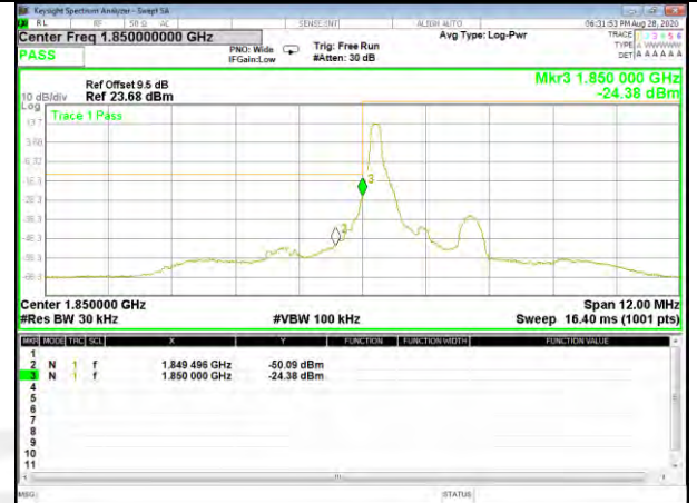
Band2_1.4M_QPSK_Low_Full-RB
