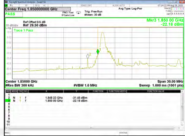
Band2_15M_16QAM_Low_Full-RB
