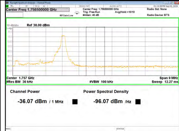
Band4_3M_QPSK_High_Full-RB
