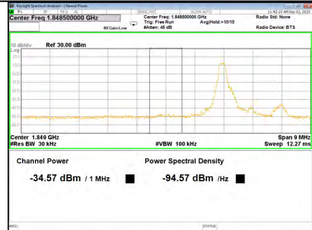
Band2_1.4M_16QAM_Low_Full-RB
