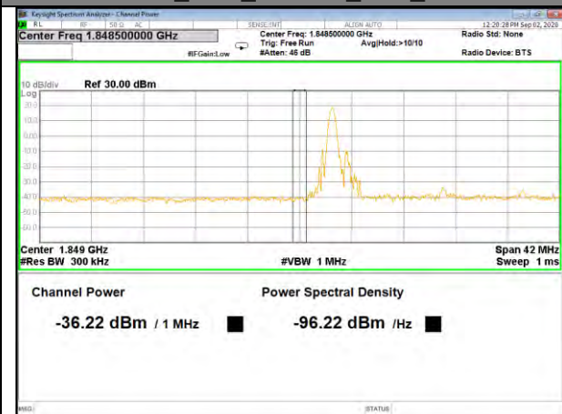
Band2_20M_16QAM_Low_1-RB
