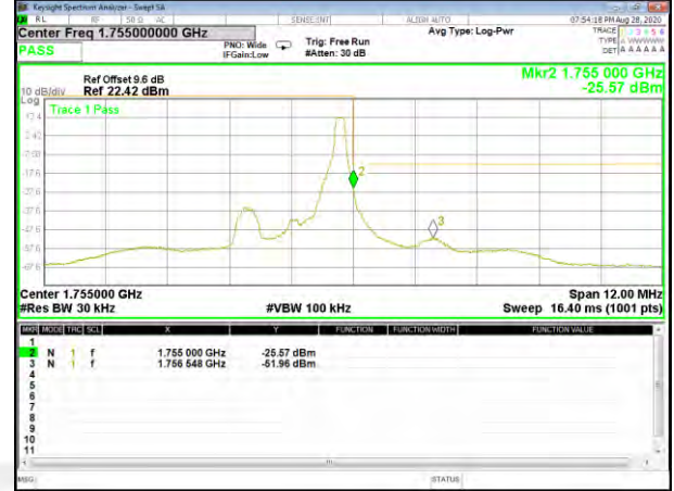
Band4_1.4M_16QAM_High_Full-RB
