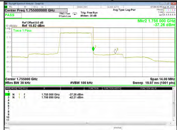
Band4_3M_QPSK_High_Full-RB
