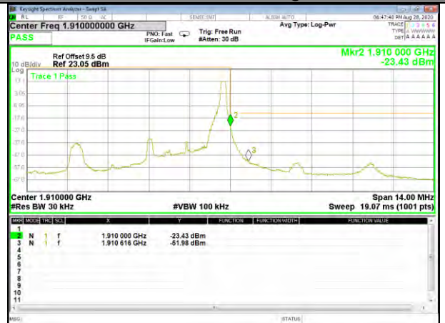
Band2_3M_16QAM_High_1-RB
