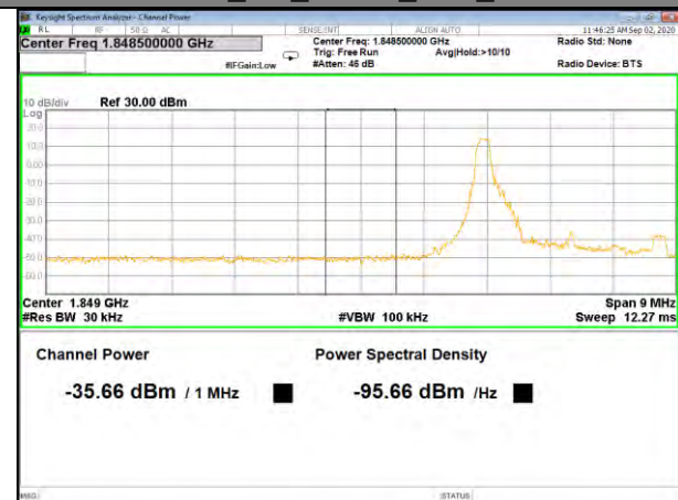
Band2_3M_QPSK_Low_1-RB
