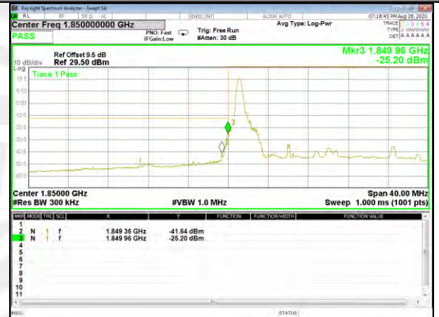
Band2_20M_QPSK_Low_Full-RB
