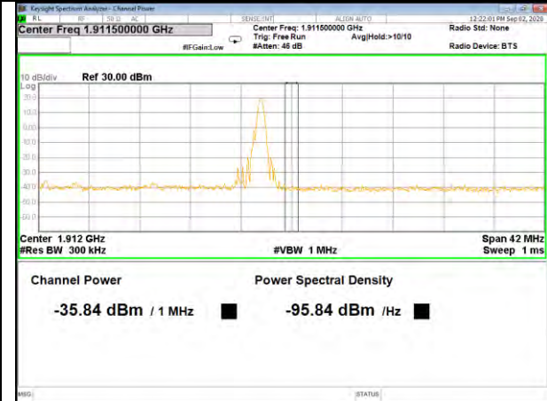
Band2_20M_16QAM_High_Full-RB
