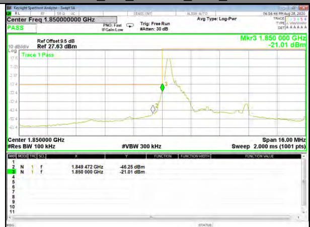
Band2_5M_16QAM_Low_1-RB
