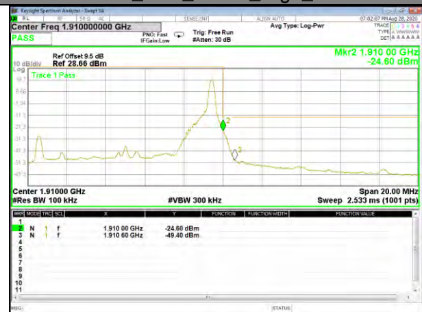
Band2_10M_QPSK_High_1-RB
