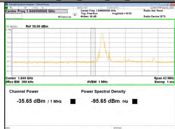
Band2_15M_QPSK_Low_1-RB
