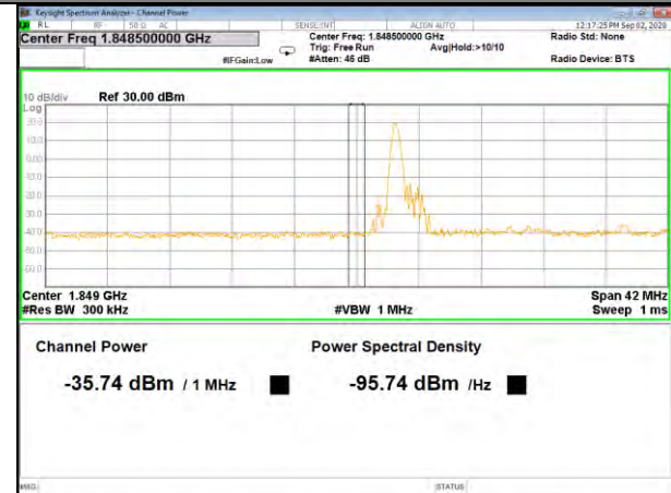
Band2_20M_QPSK_Low_Full-RB
