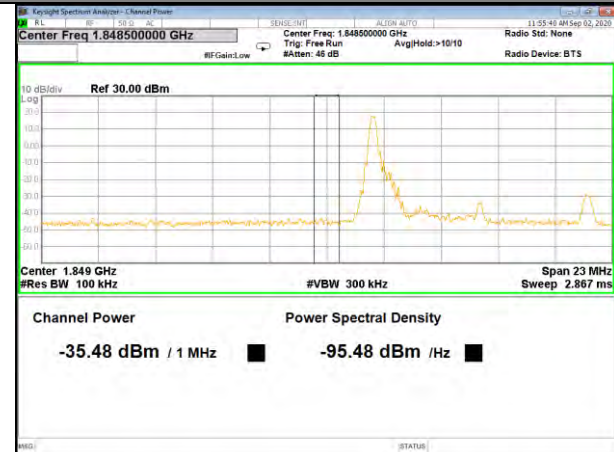
Band2_5M_QPSK_Low_Full-RB
