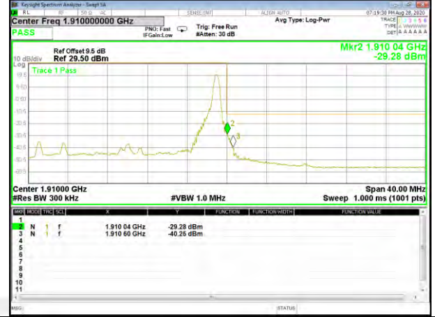
Band2_20M_QPSK_High_Full-RB
