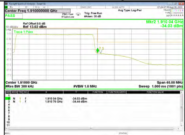
Band2_20M_16QAM_High_Full-RB
