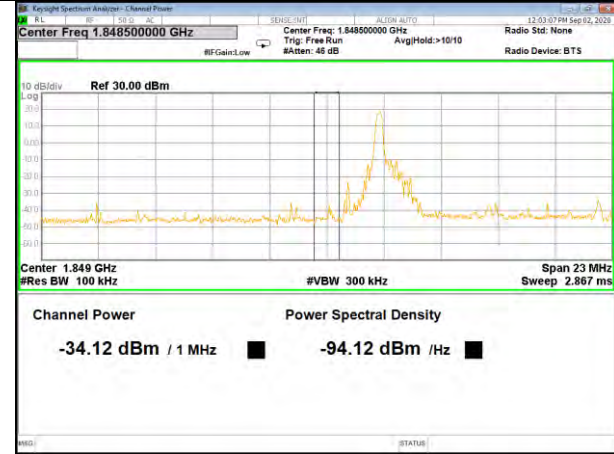
Band2_10M_QPSK_Low_Full-RB
