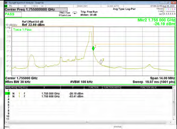
Band4_3M_QPSK_High_Full-RB
