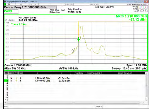
Band4_1.4M_QPSK_Low_Full-RB
