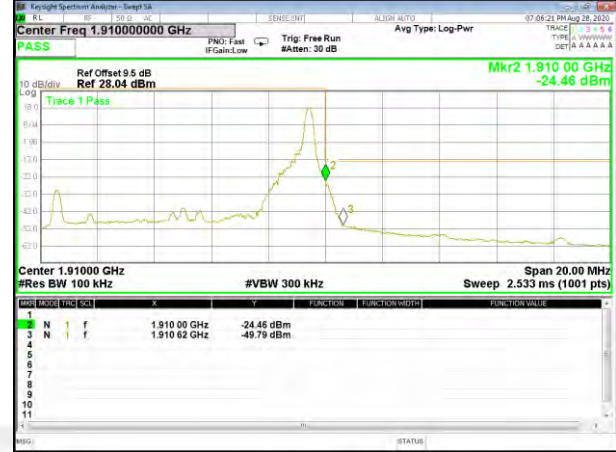
Band2_10M_16QAM_High_Full-RB
