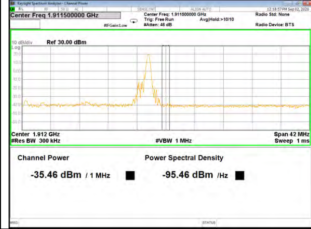
Band2_20M_QPSK_High_Full-RB
