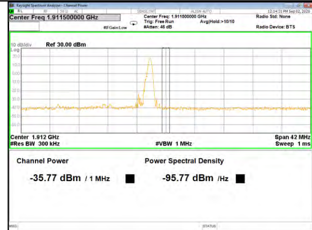
Band2_15M_16QAM_High_1-RB
