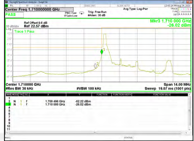
Band4_3M_16QAM_Low_Full-RB
