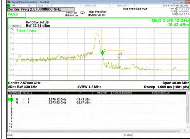
B7_Q16_20M_High_1-RB_Bedge
