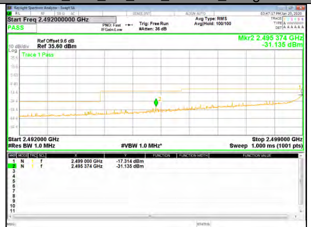
B7_Q16_5M_Low_Full-RB_Bedge
