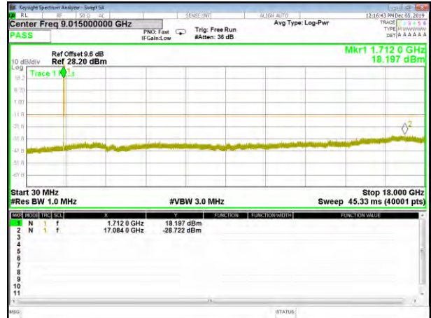
B4 HSDPA Lower Conducted Spurious
