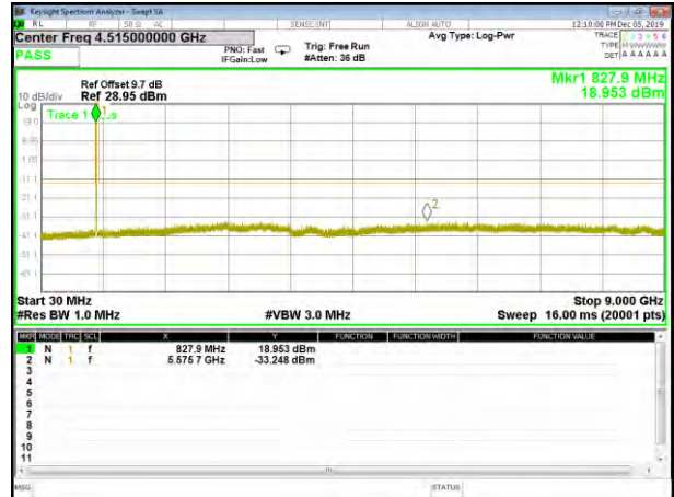
B5 HSDPA Lower Conducted Spurious
