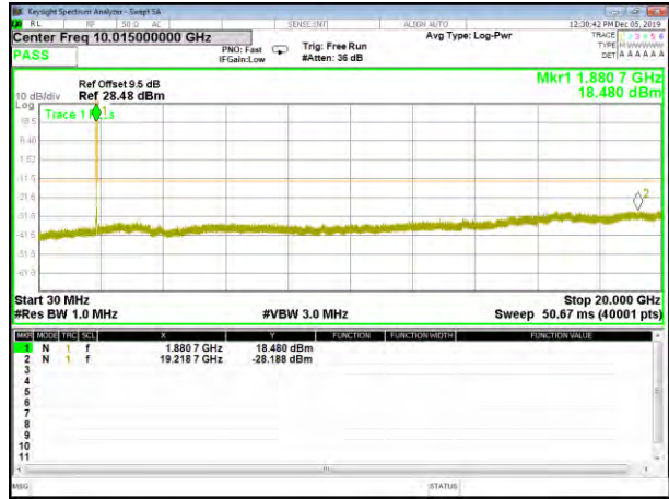
B2_HSUPA_Middle_Conducted_Spurious
