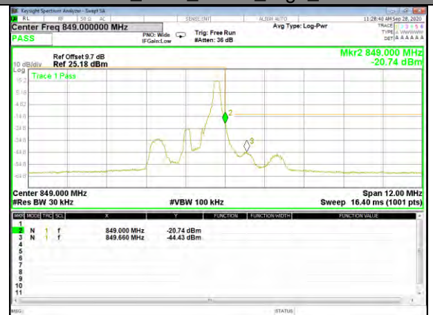
Band5_1.4M_QPSK_High_1-RB
