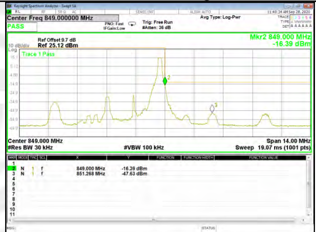
Band5_3M_QPSK_High_Full-RB
