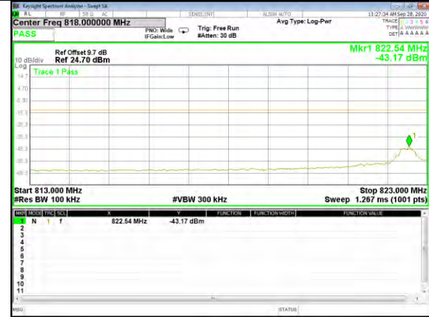
Band5_1.4M_QPSK_Low_Full-RB
