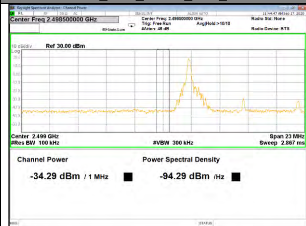
Band7_10M_QPSK_Low_1-RB
