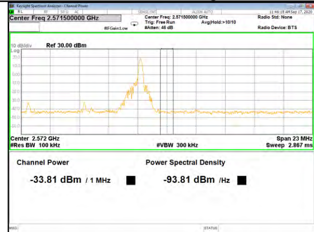
Band7_10M_QPSK_High_Full-RB
