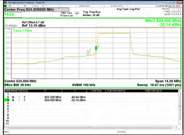
Band5_3M_QPSK_High_1-RB
