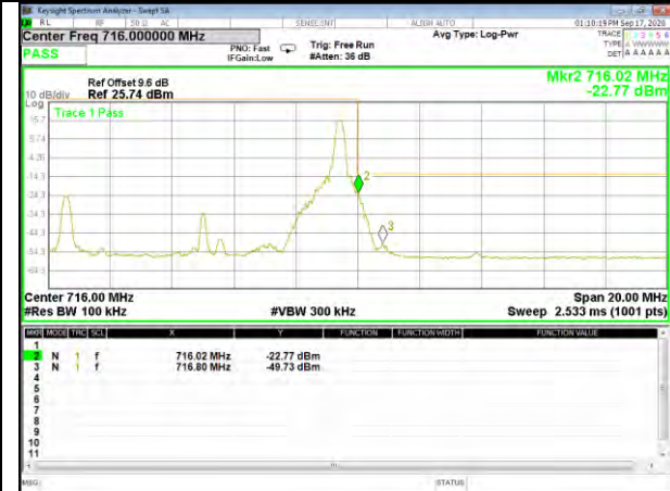
Band17_10M_16QAM_High_1-RB
