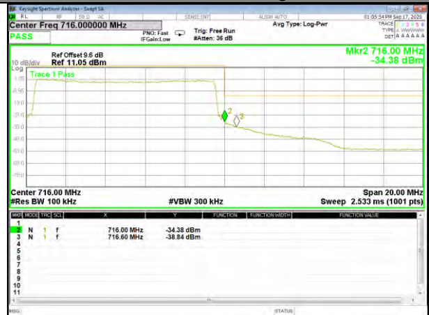
Band17_10M_QPSK_High_Full-RB
