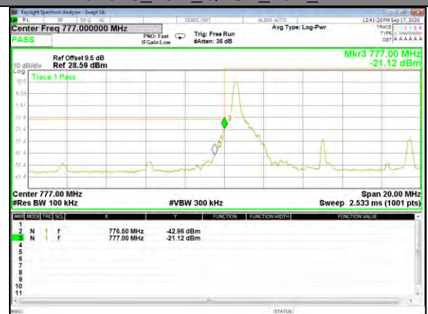
Band13_10M_QPSK_Low_1-RB
