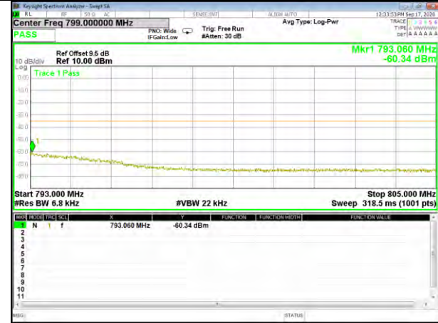
Band13_5M_16QAM_Low_1-RB
