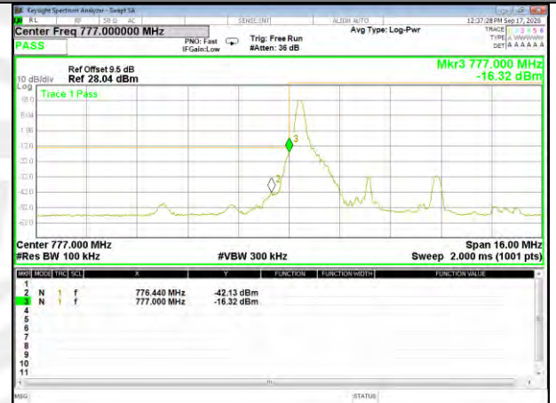
Band13_5M_16QAM_Low_Full-RB
