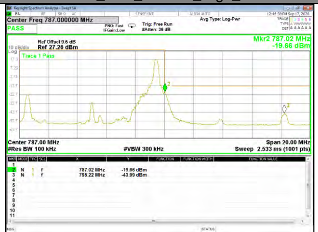
Band13_10M_16QAM_High_1-RB
