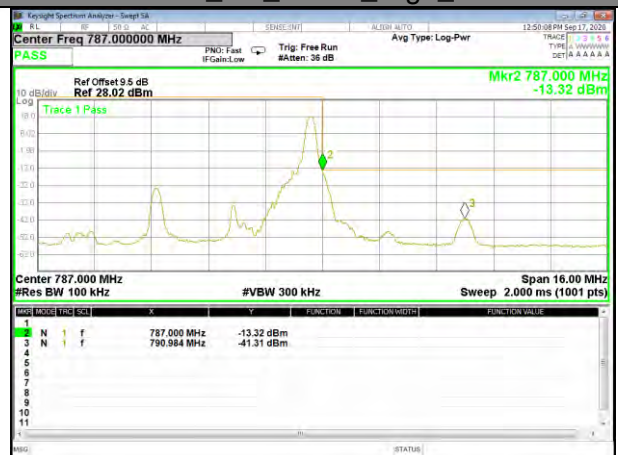
Band13_5M_QPSK_High_1-RB
