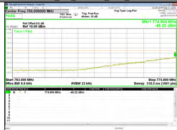
Band13_5M_16QAM_Low_Full-RB
