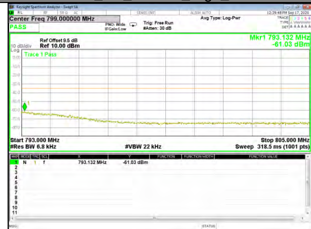
Band13_10M_QPSK_Low_1-RB
