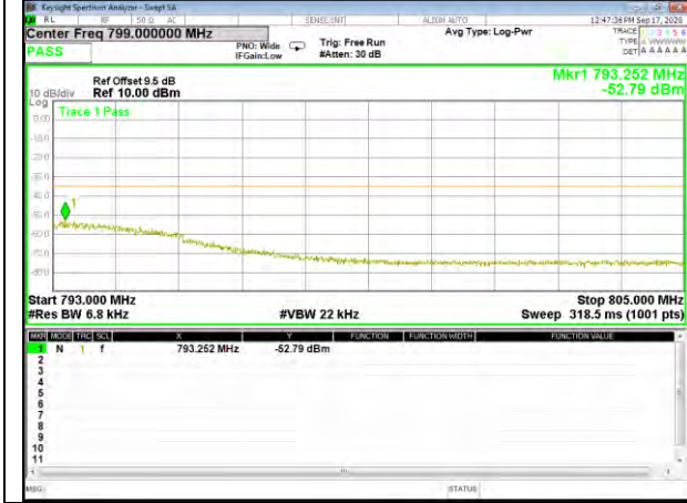
Band13_10M_16QAM_High_Full-RB
