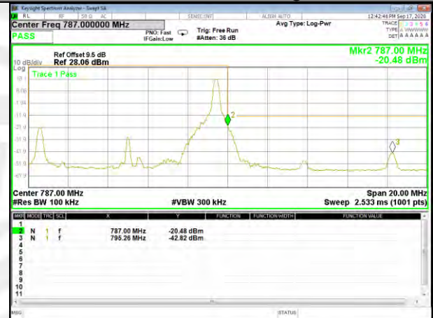
Band13_10M_QPSK_High_Full-RB
