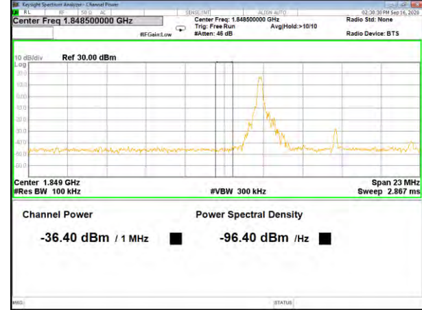
Band2_10M_QPSK_Low_Full-RB
