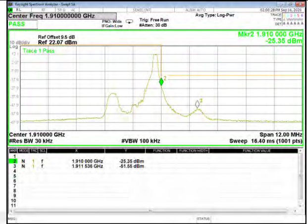
Band2_1.4M_16QAM_High_Full-RB
