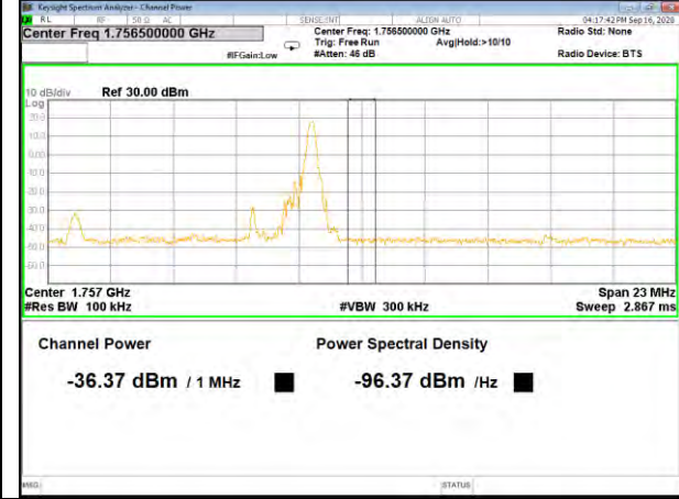
Band4_5M_QPSK_High_Full-RB
