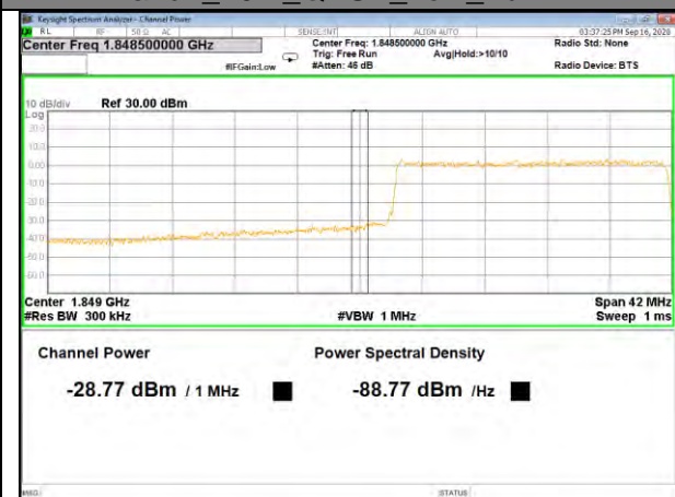
Band2_20M_QPSK_Low_Full-RB
