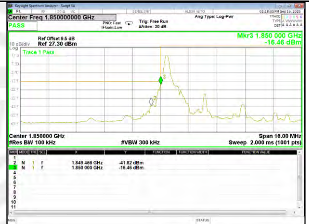
Band2_5M_QPSK_Low_Full-RB
