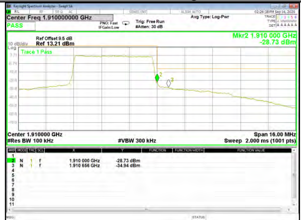
Band2_5M_16QAM_High_Full-RB
