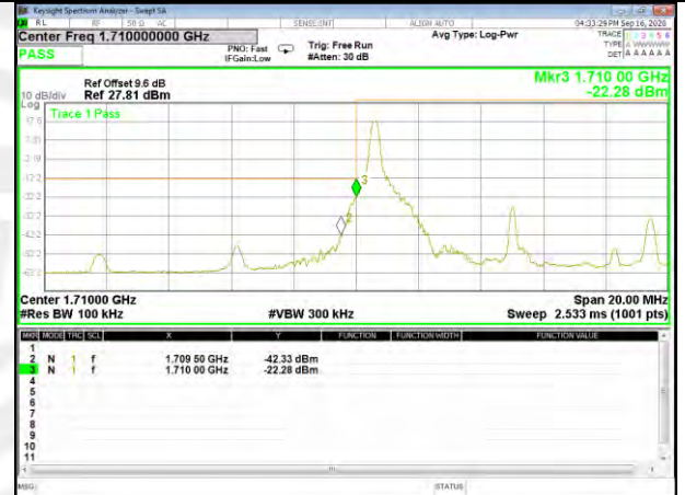
Band4_10M_16QAM_Low_Full-RB
