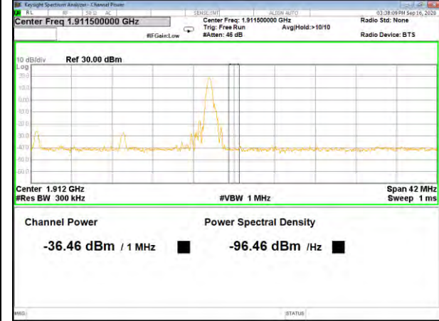
Band2_20M_QPSK_High_Full-RB
