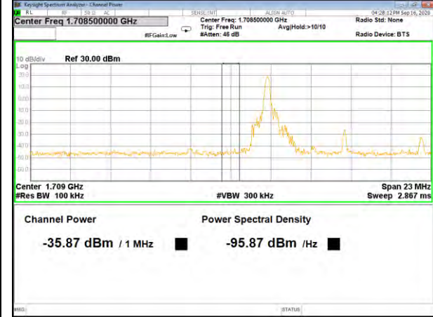
Band4_10M_QPSK_Low_Full-RB
