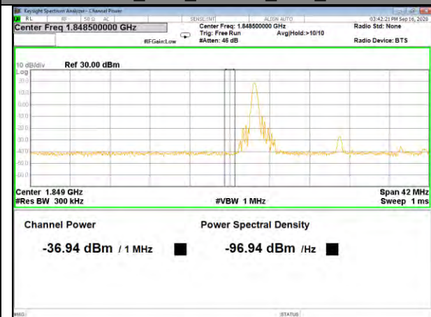
Band2_20M_16QAM_Low_1-RB
