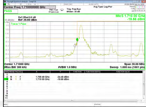
Band4_15M_16QAM_Low_Full-RB
