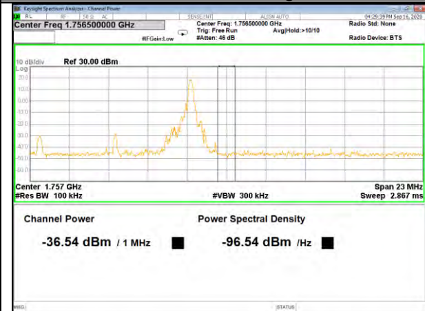
Band4_10M_QPSK_High_1-RB
