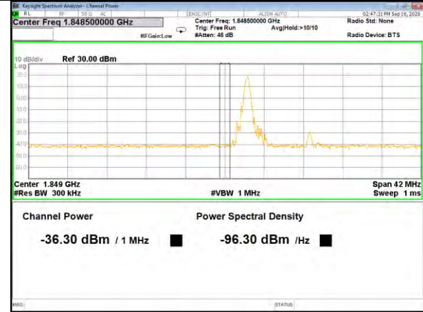
Band2_15M_16QAM_Low_Full-RB
