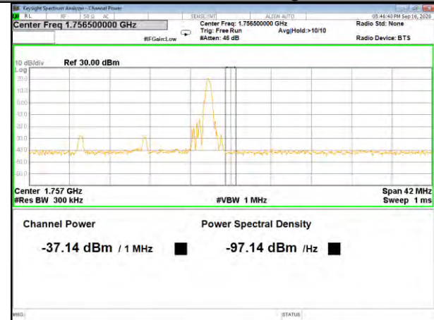
Band4_15M_QPSK_High_Full-RB
