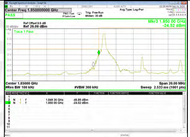
Band2_10M_16QAM_Low_Full-RB
