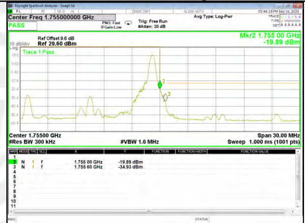
Band4_15M_QPSK_High_Full-RB
