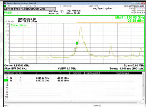
Band2_20M_QPSK_Low_Full-RB
