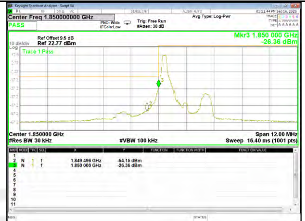
Band2_1.4M_QPSK_Low_Full-RB
