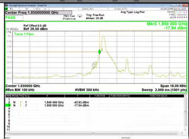
Band2_5M_16QAM_Low_1-RB
