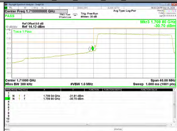
Band4_20M_QPSK_Low_Full-RB
