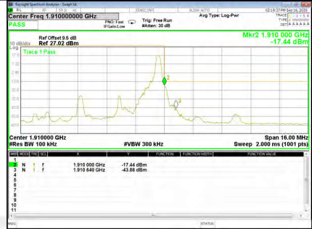
Band2_5M_QPSK_High_Full-RB
