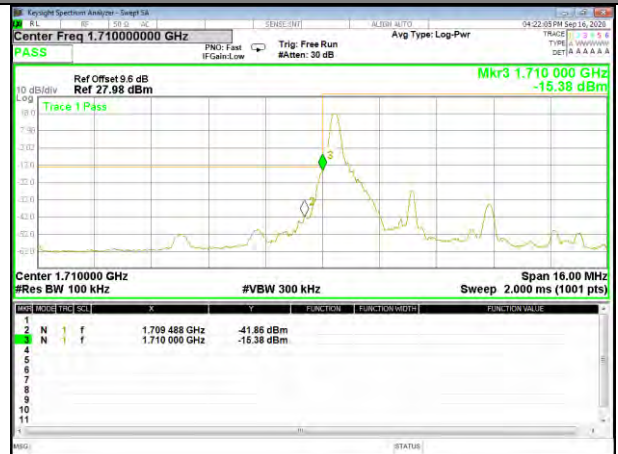
Band4_5M_16QAM_Low_1-RB
