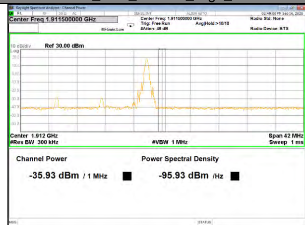
Band2_15M_16QAM_High_1-RB
