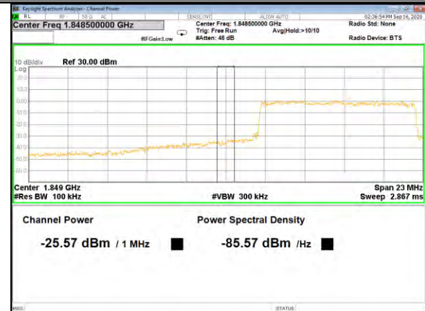
Band2_10M_16QAM_Low_Full-RB
