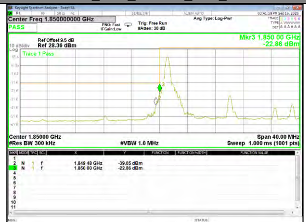
Band2_20M_16QAM_Low_1-RB
