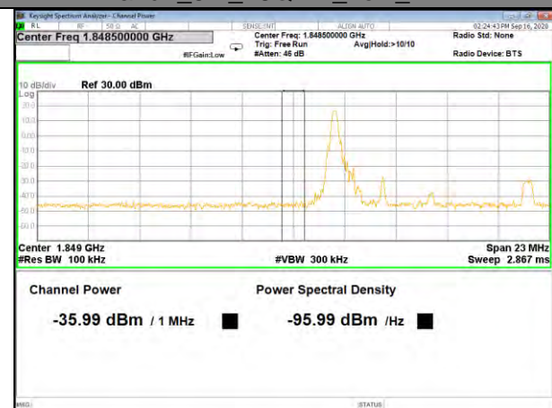
Band2_5M_16QAM_Low_1-RB
