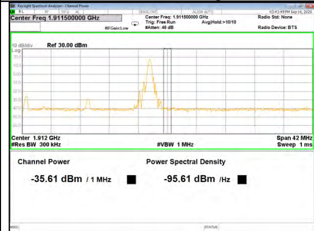
Band2_20M_16QAM_High_Full-RB
