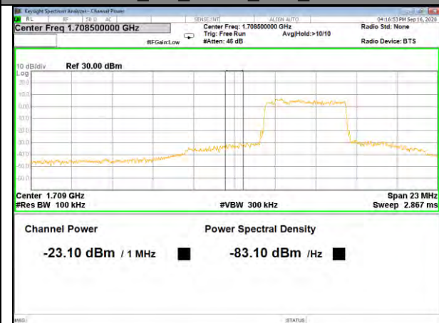
Band4_5M_QPSK_Low_Full-RB
