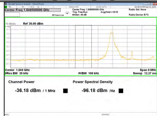
Band2_3M_QPSK_Low_1-RB
