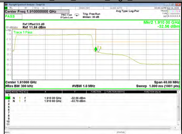
Band2_20M_16QAM_High_Full-RB
