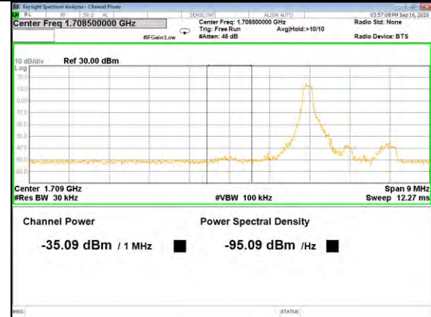
Band4_1.4M_16QAM_Low_Full-RB
