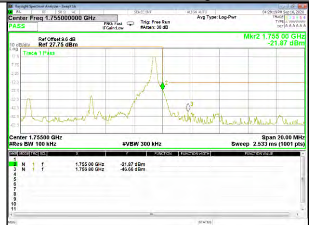
Band4_10M_QPSK_High_1-RB
