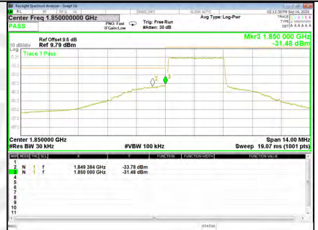
Band2_3M_16QAM_High_1-RB
