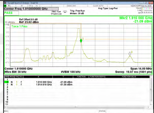
Band2_3M_QPSK_High_Full-RB
