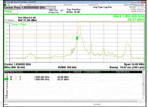
Band2_3M_16QAM_Low_Full-RB
