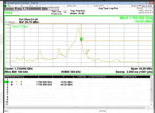
Band4_5M_16QAM_High_Full-RB
