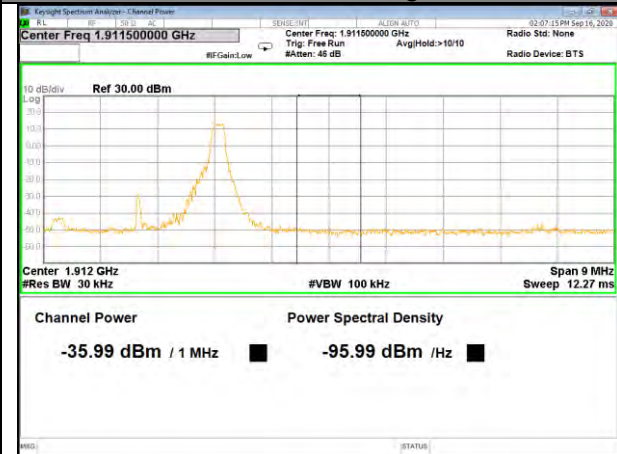
Band2_3M_QPSK_High_Full-RB
