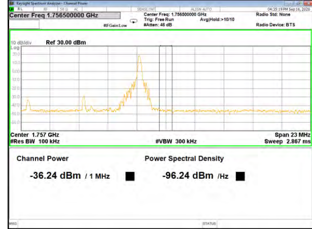
Band4_10M_16QAM_High_Full-RB
