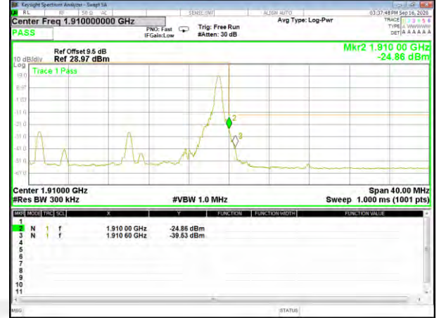
Band2_20M_QPSK_High_Full-RB
