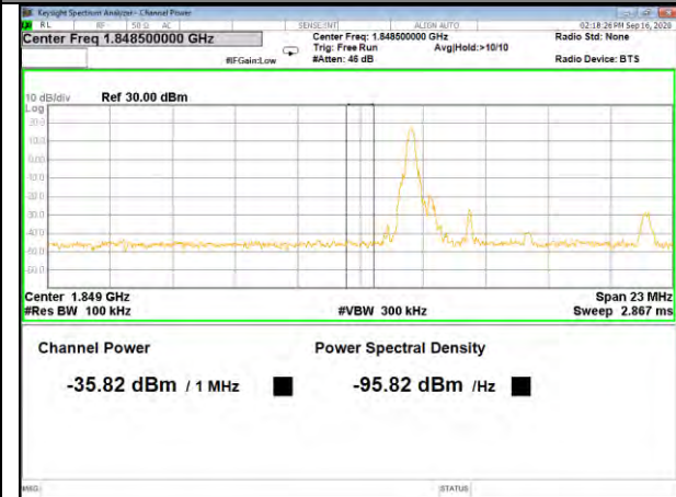
Band2_5M_QPSK_Low_Full-RB
