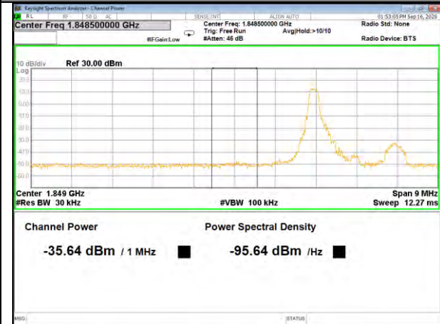
Band2_1.4M_QPSK_Low_Full-RB
