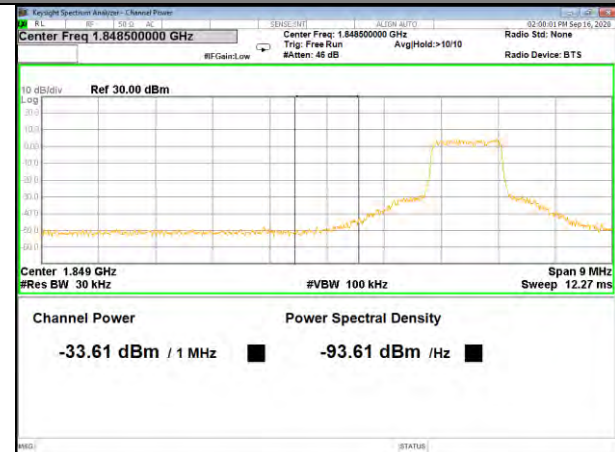
Band2_1.4M_16QAM_Low_Full-RB
