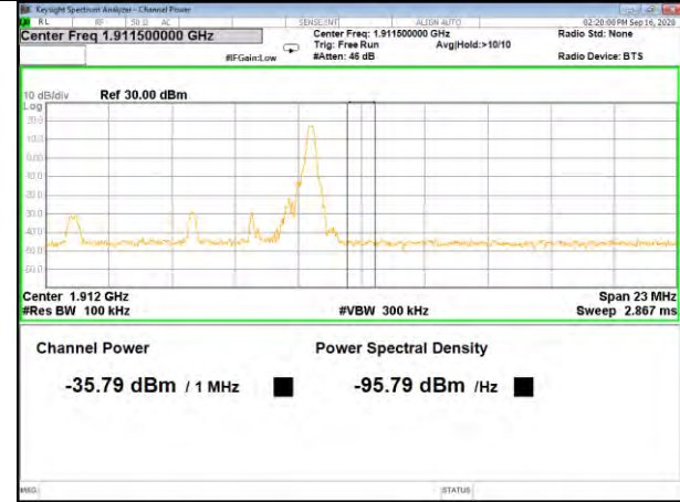
Band2_5M_QPSK_High_Full-RB
