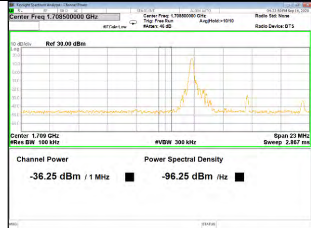
Band4_10M_16QAM_Low_Full-RB
