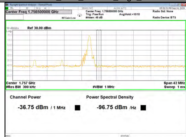
Band4_15M_16QAM_High_1-RB
