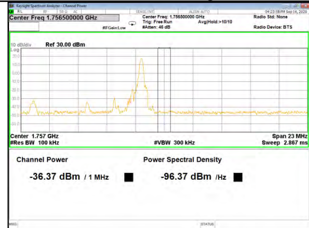
Band4_5M_16QAM_High_Full-RB
