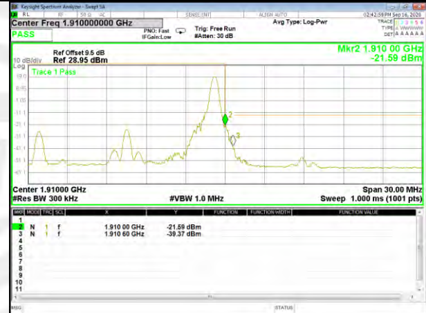
Band2_15M_QPSK_High_Full-RB
