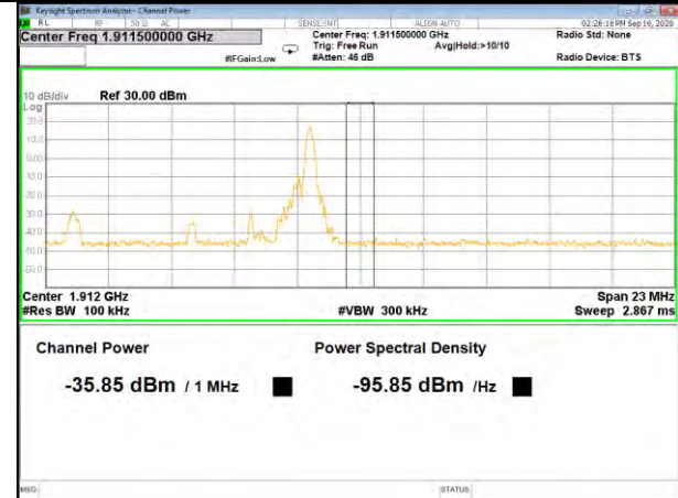
Band2_5M_16QAM_High_Full-RB
