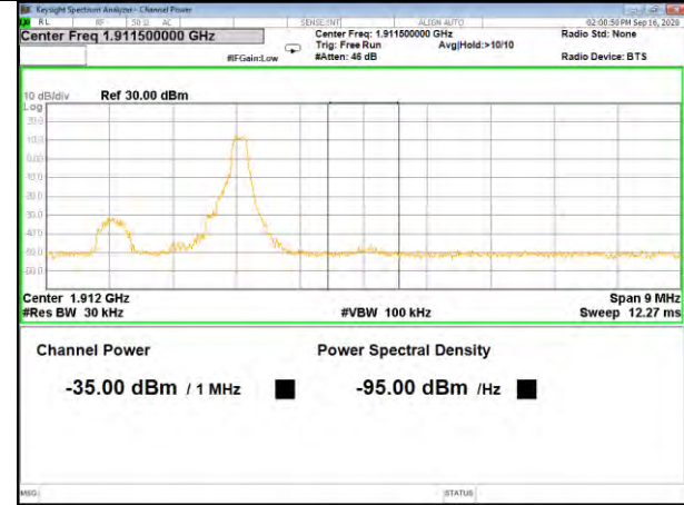
Band2_1.4M_16QAM_High_Full-RB
