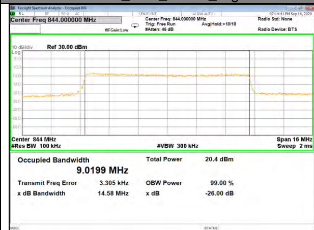
Band5_10M_QPSK_High
