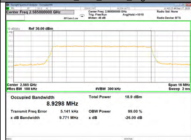
Band7_10M_QPSK_High
