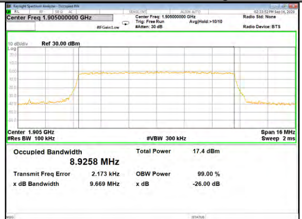
Band2_10M_16QAM_High
