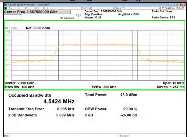
Band7_5M_16QAM_High
