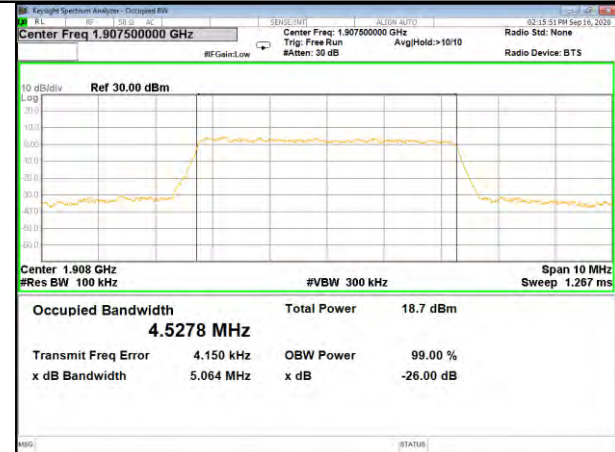
Band2_5M_QPSK_High
