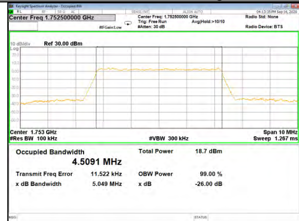
Band4_5M_QPSK_High
