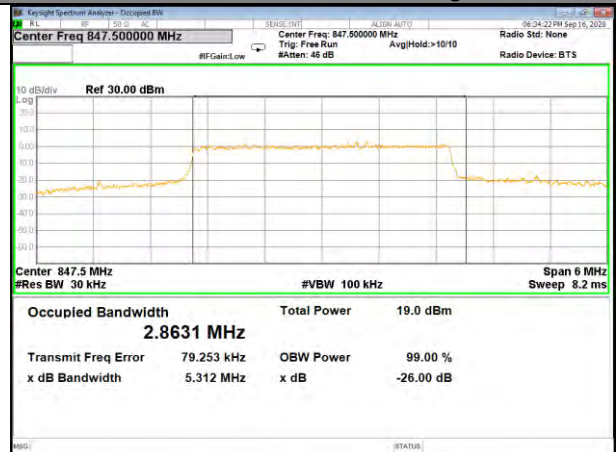
Band5_3M_16QAM_High
