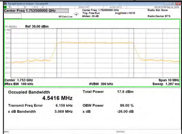
Band4_5M_16QAM_High
