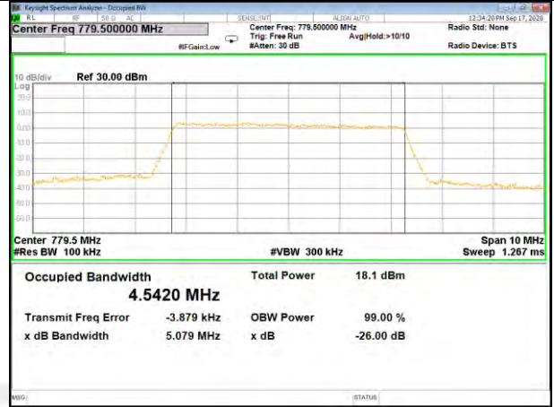
Band13_5M_16QAM_Middle
