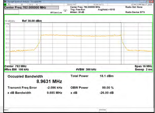
Band13_10M_16QAM_Middle
