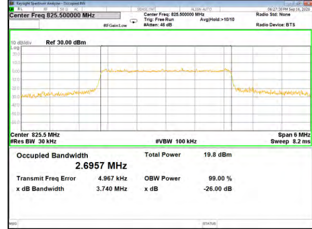
Band5_3M_QPSK_Middle
