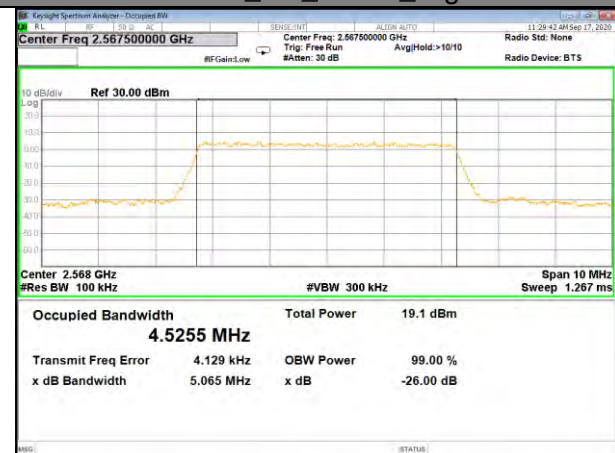
Band7_5M_QPSK_High
