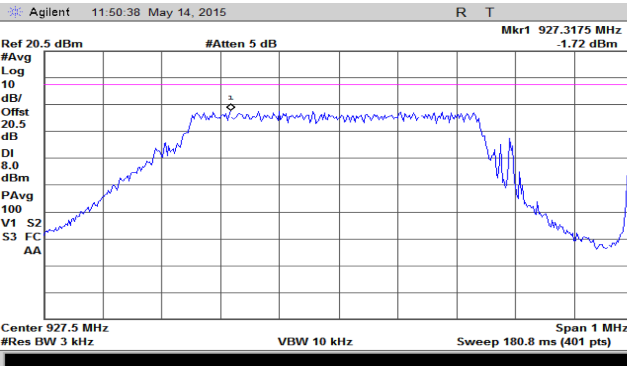
Plot 28 – Power Spectral Density – Highest Channel – DTS Mode
