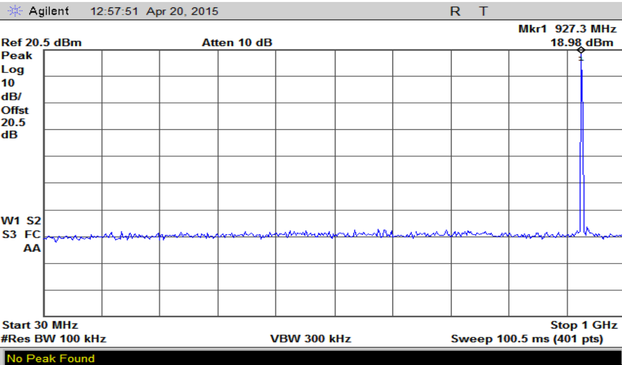
Plot 20 – High Band – 30MHz to 1GHz
