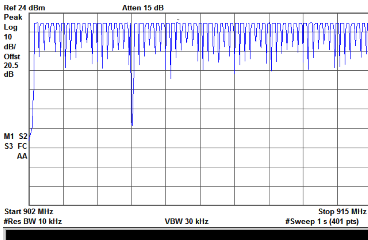
Plot 34 – Time Period – Hybrid Mode (64 Hops)
