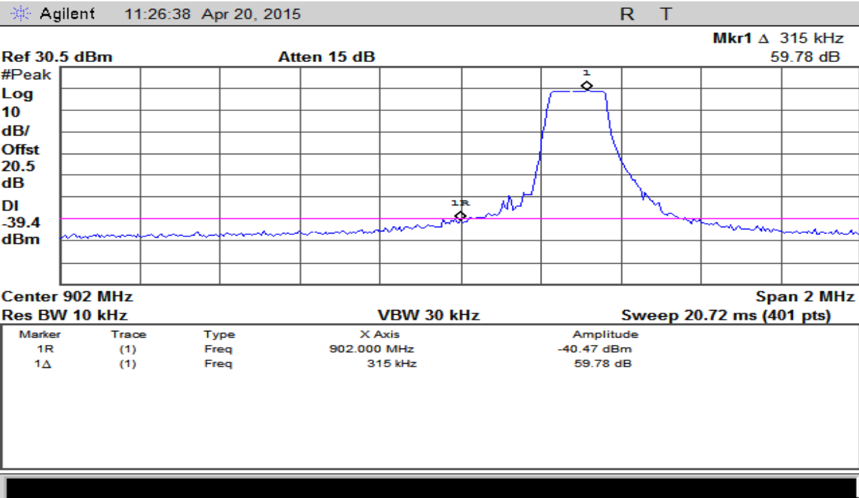
Plot 24 - Band Edge – Low Channel – Hybrid Mode
