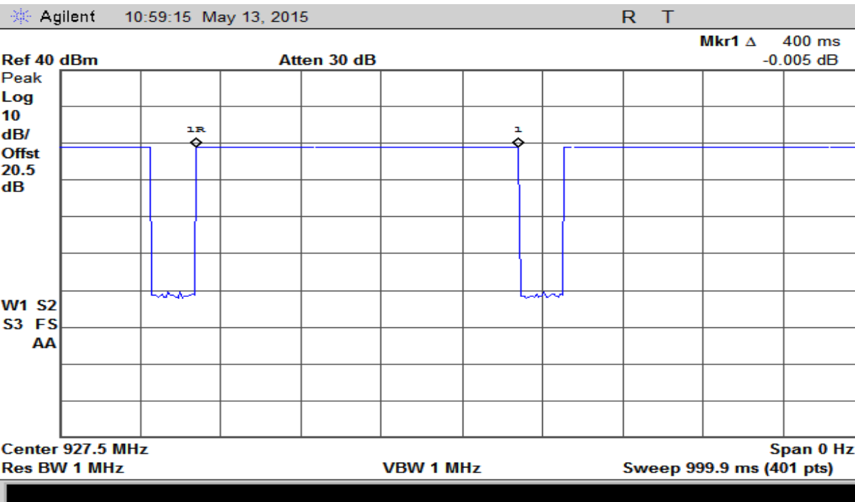
Plot 32 – Dwell Time – Hybrid Mode (SF 8)
