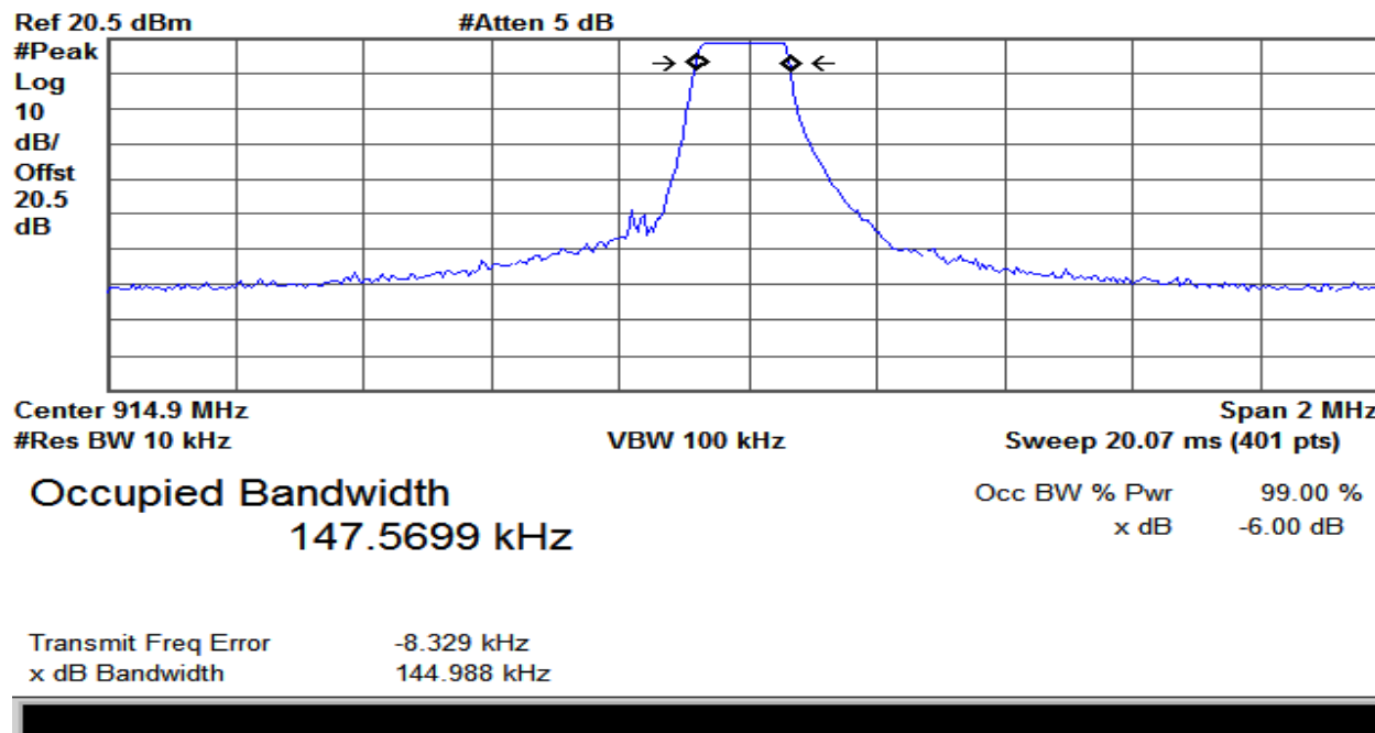
Plot 11 – Middle Channel – 6dB BW – Hybrid Mode
