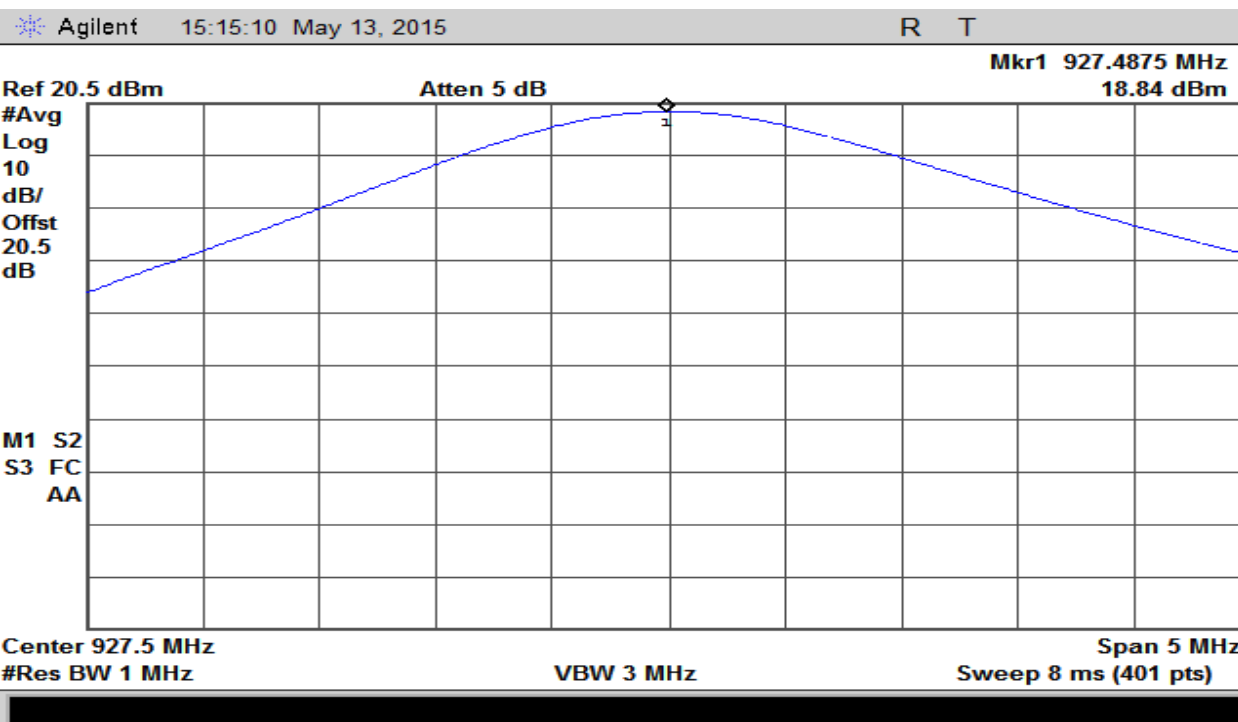
Plot 15 – Output Power – High
