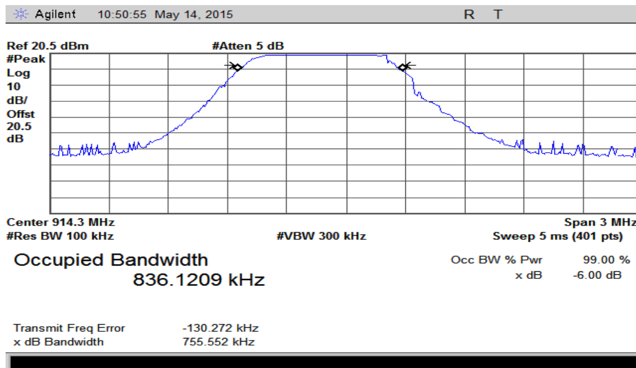
Plot 5 – Middle Channel – 6dB BW – DTS Mode (SF 10)
