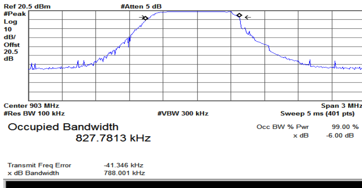
Plot 4 – Lowest Channel – 6dB BW – DTS Mode (SF 10)
