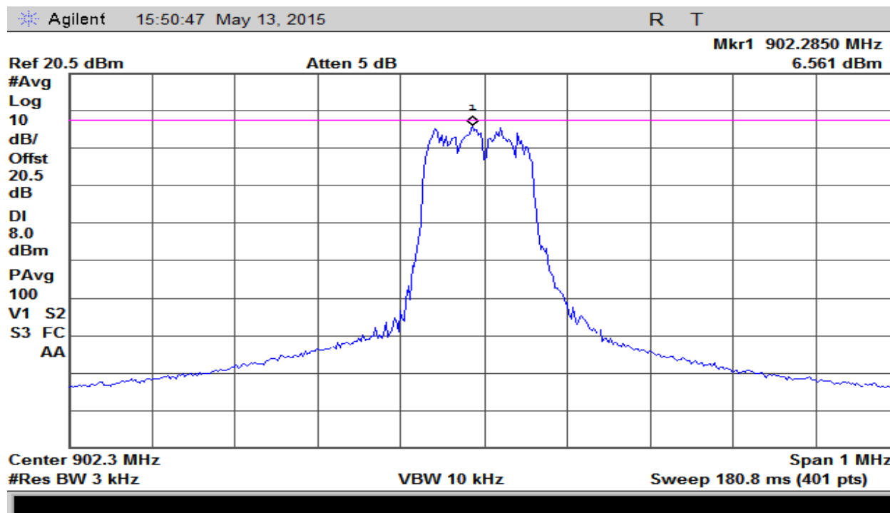
Plot 29 – Power Spectral Density – Lowest Channel – Hybrid Mode (SF10)
