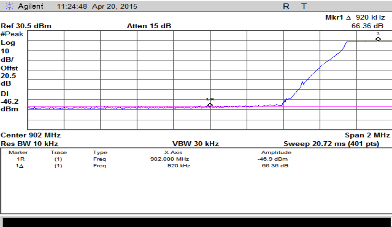
Plot 22 - Band Edge – Low Channel – DTS Mode
