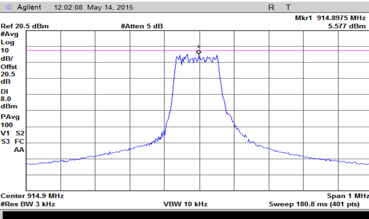
Plot 30 – Power Spectral Density – Middle Channel – Hybrid Mode (SF 10)
