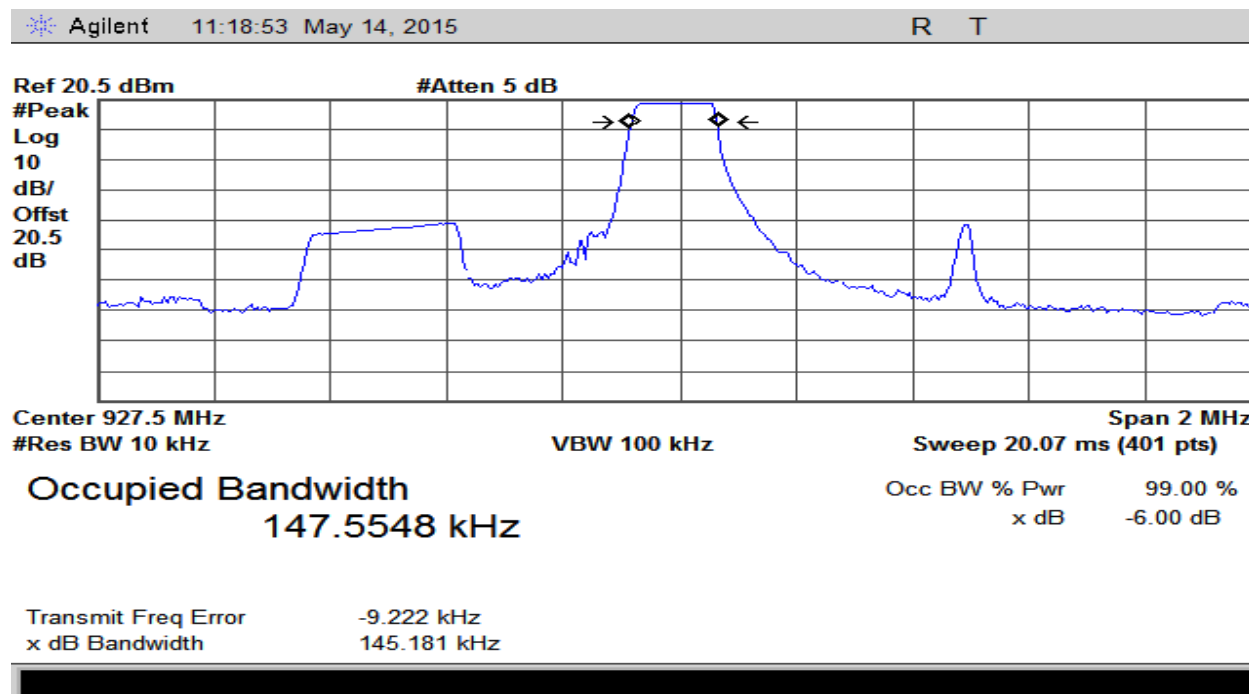
Plot 12 – Highest Channel – 6dB BW – Hybrid Mode
