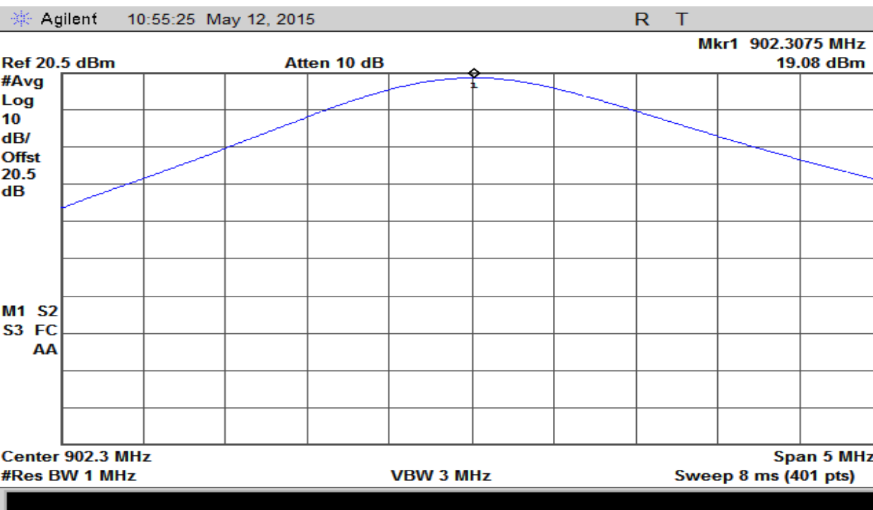
Plot 13 – Output Power – Low
