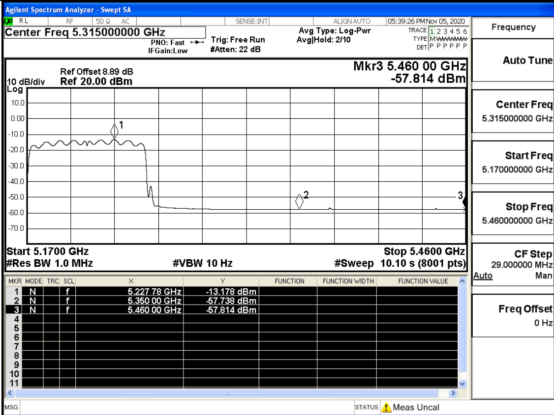
IEEE 802.11ac80 / Channel 42 / 5210MHz / Average
