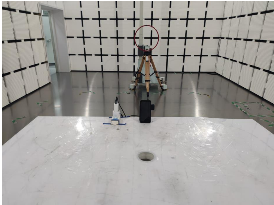
Radiation (9KHz-30MHz)
