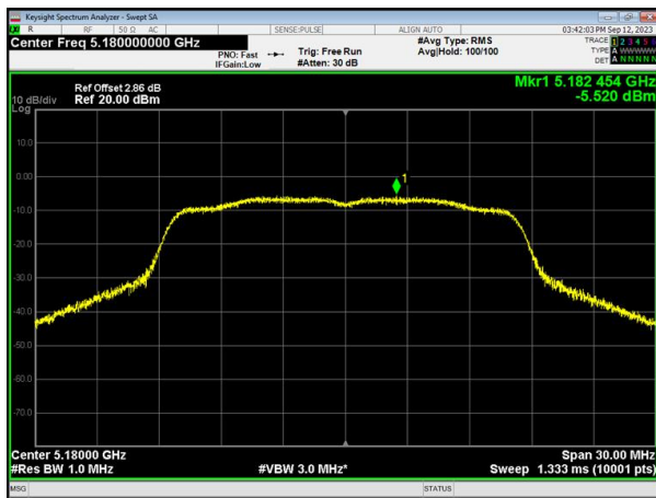
(802.11a) PSD plot on channel 36(RMS)
