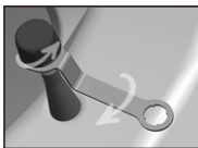
A、用扳手顺时针方向旋转六角螺母, 将其与传感器分离,再逆时针方 向旋转传感器 Screw the nut clockwise to separate it from the sensor by wrench and then screw out the sensor by hand
