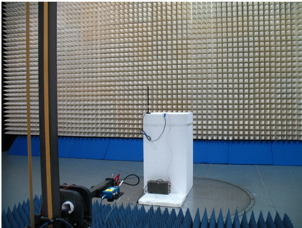
Radiated Spurious Emissions, 1-18GHz, L-Com model HG2408MGUR-RSP antenna
