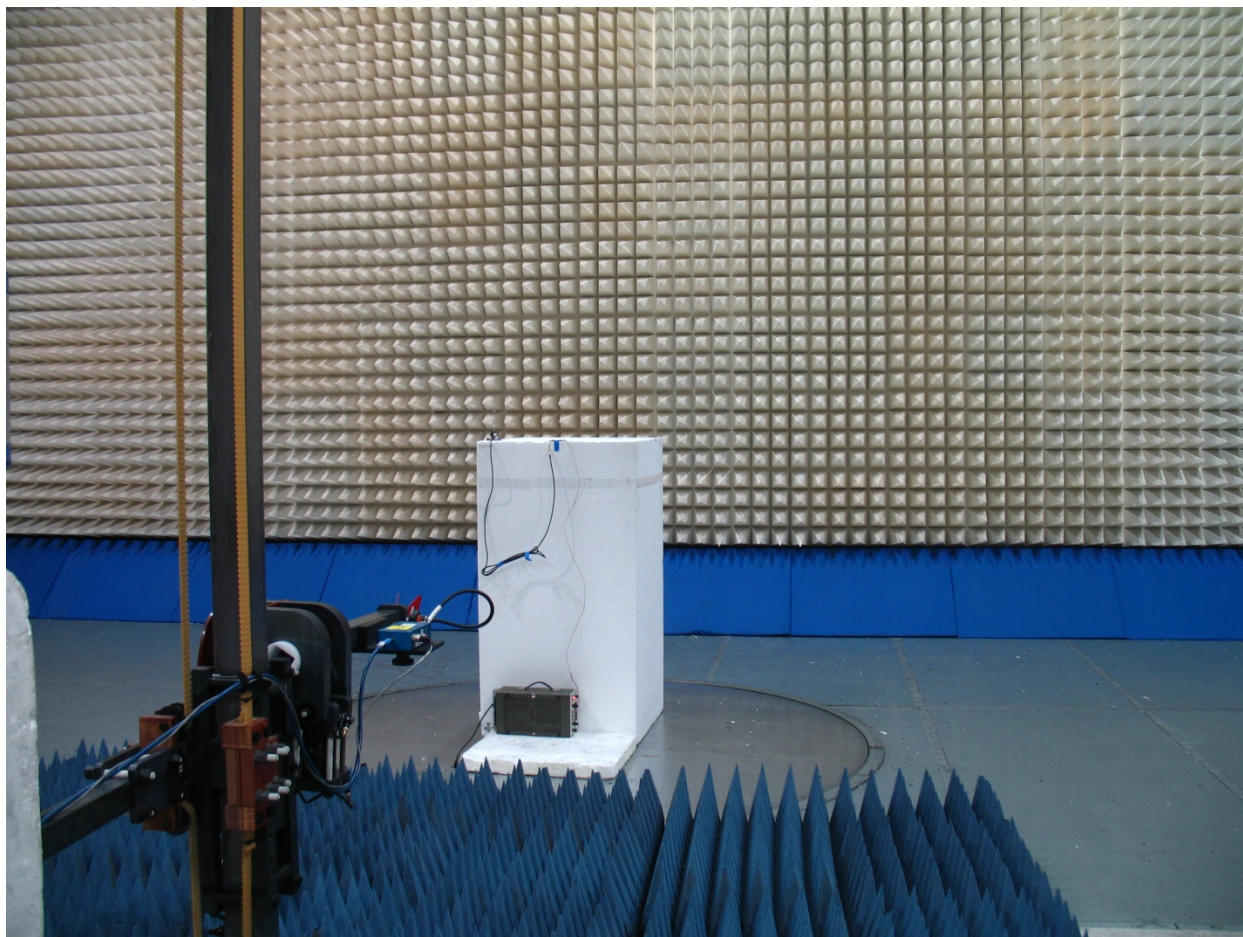
Radiated Spurious Emissions, 1-18GHz, L-Com model HG2405MGU antenna
