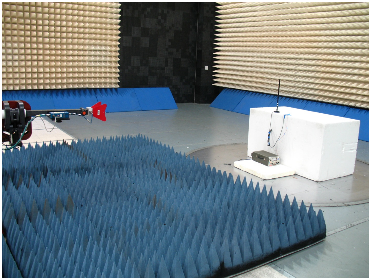
Unintentional Radiated Emissions, 1-18GHz, L-Com model HG2408MGUR-RSP antenna
