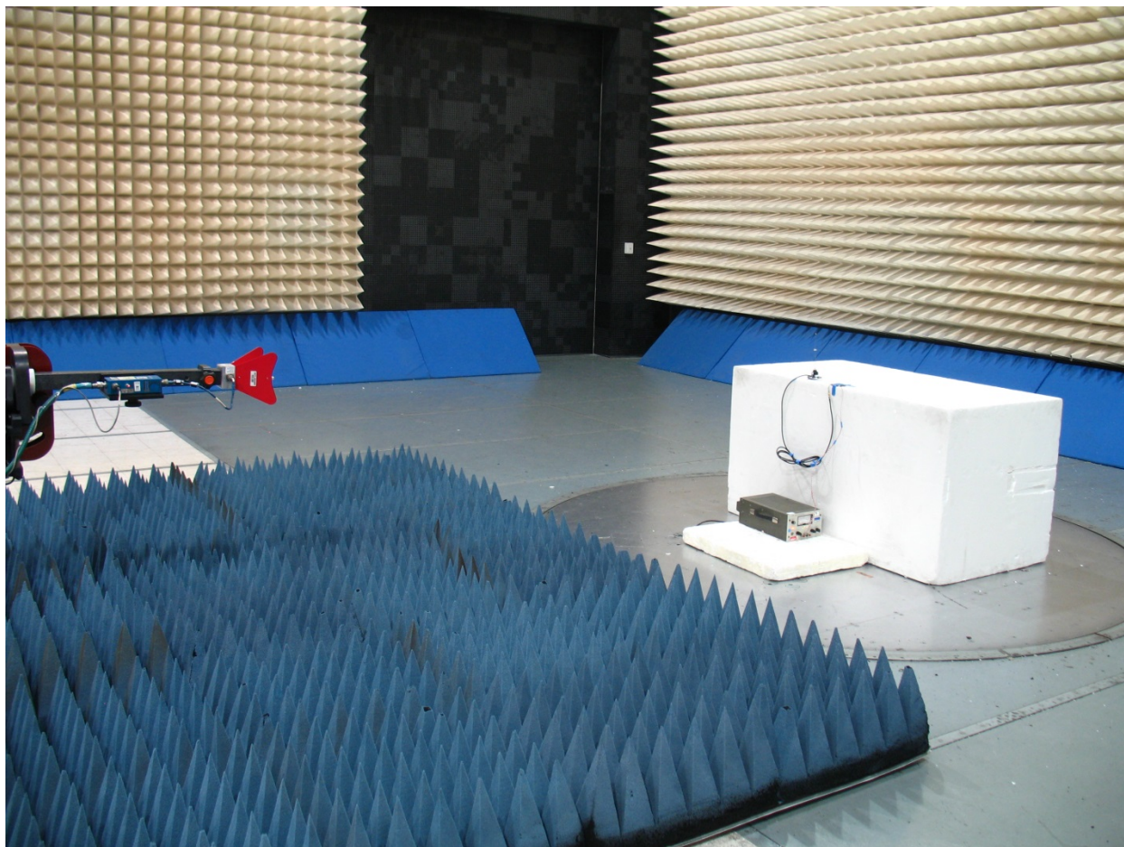
Unintentional Radiated Emissions, 1-18GHz, L-Com model HG2405MGU antenna
