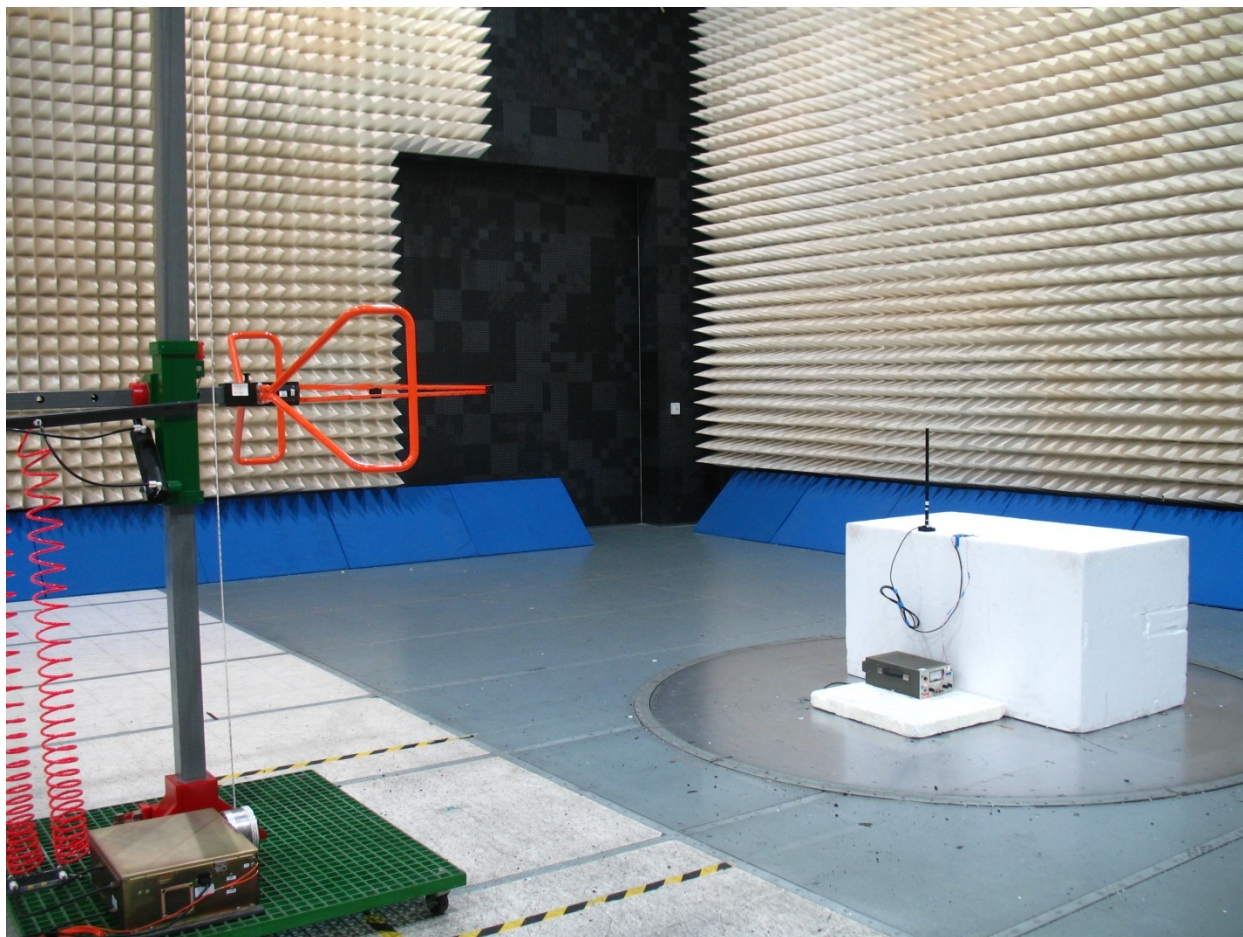
Radiated Spurious Emissions and unintentional radiated emissions, 30MHz-1GHz, L-Com model HG2408MGUR-RSP antenna
