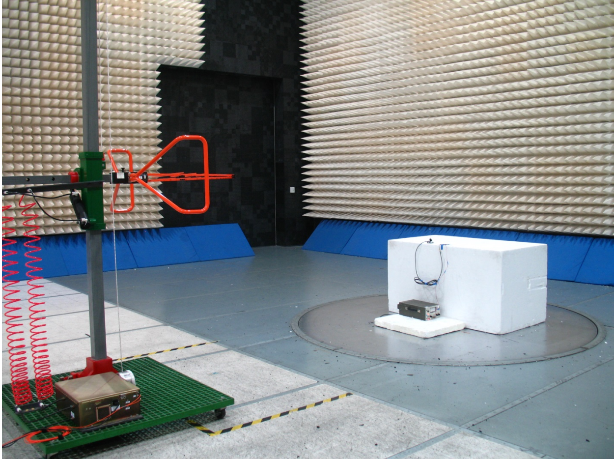
Radiated Spurious Emissions and unintentional radiated emissions, 30MHz-1GHz, L-Com model HG2405MGU antenna
