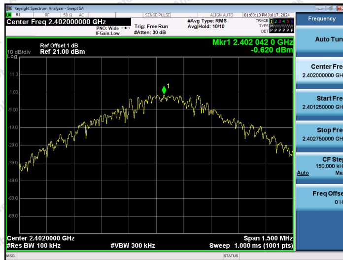
2.4G-Ant1-2402-0~Reference-PASS
