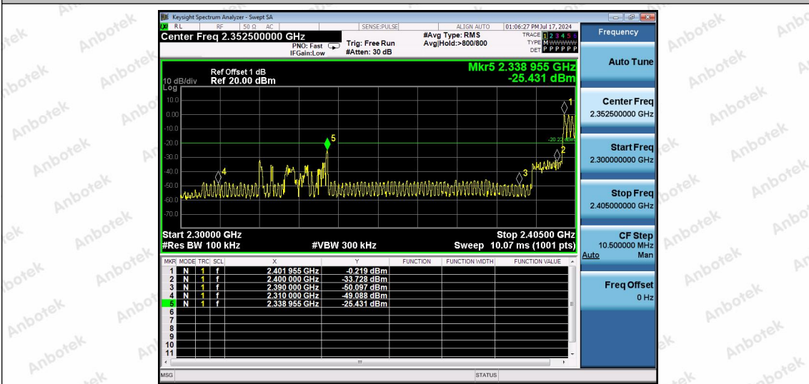
2.4G-Ant1-Hop_2402-PASS
