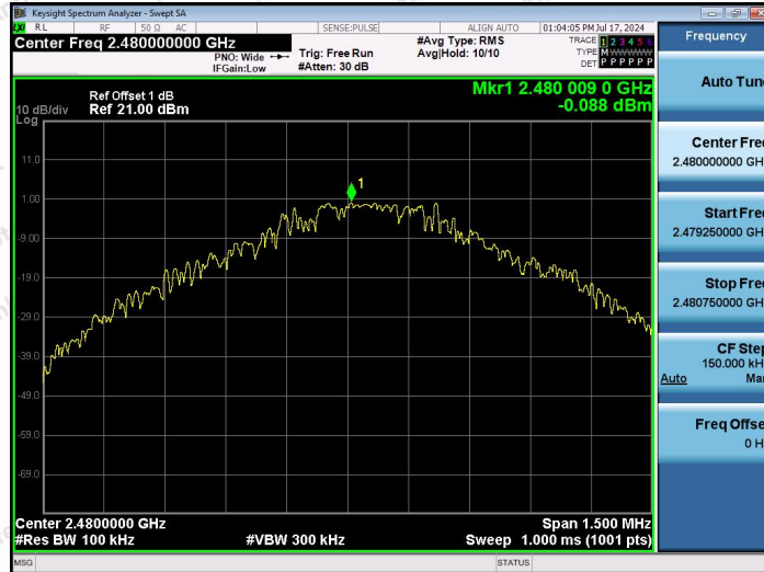
2.4G-Ant1-2480-0~Reference-PASS
