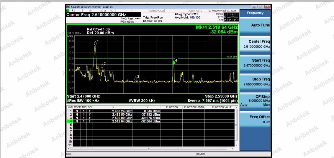
2.4G-Ant1-2480-PASS
