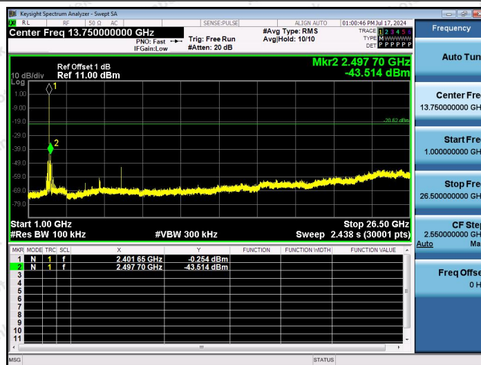
2.4G-Ant1-2402-1000~26500-PASS
