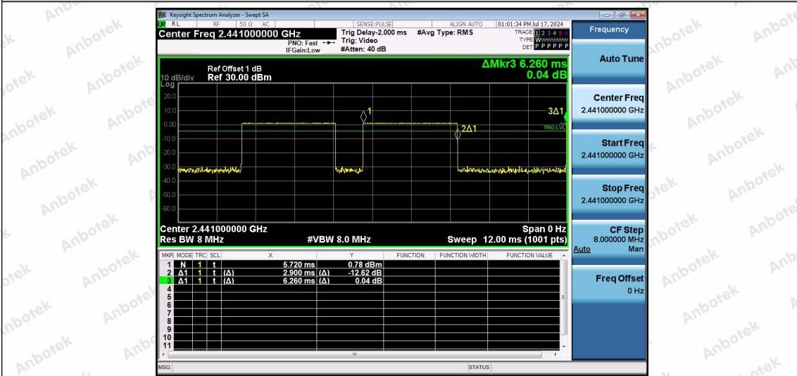
NTNV-2.4G-Ant1-2441
