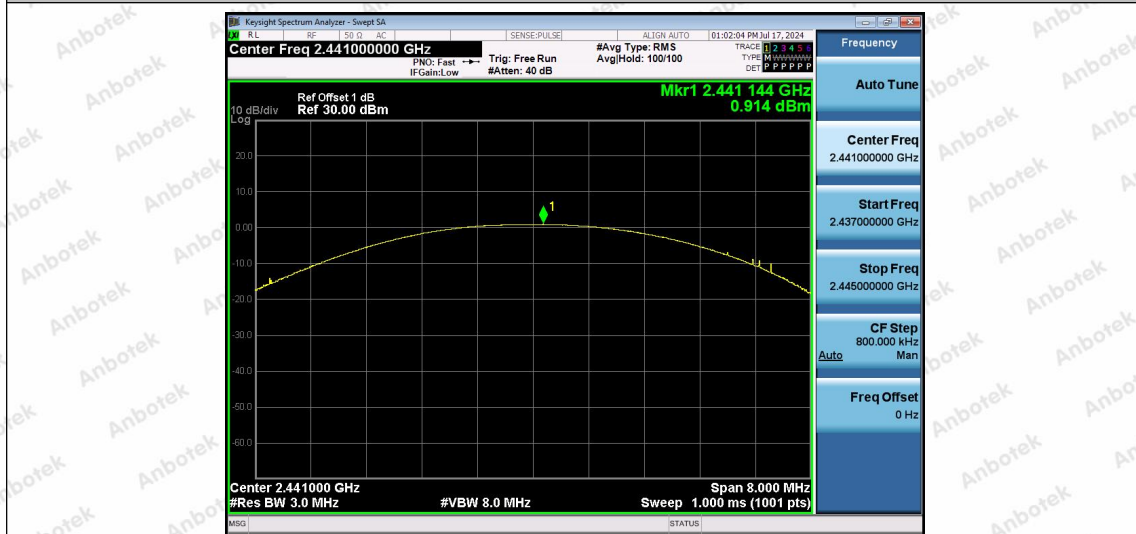
2.4G-Ant1-2441-PASS
