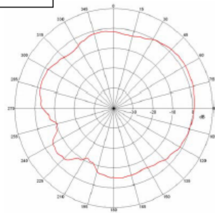
XZ-plane @2440MHz Total
