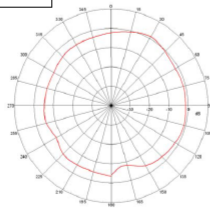
YZ-plane @2440MHz Total
