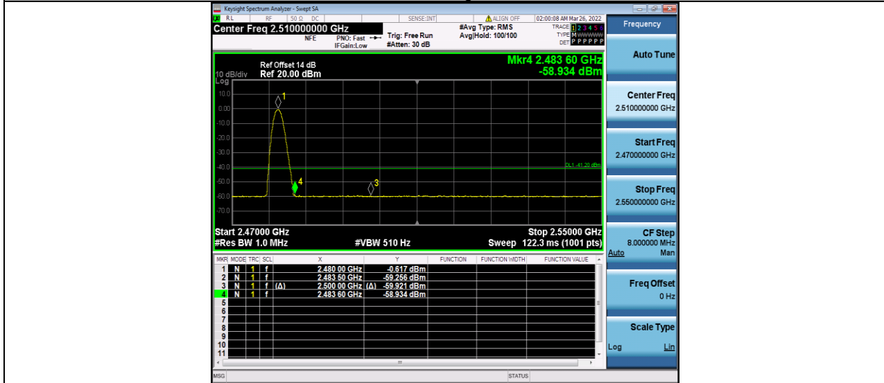
BLE_1M_Ant1_High_2480_Peak
