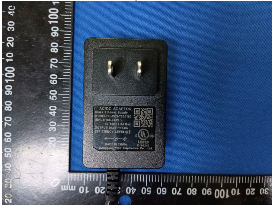
Adapter-1
