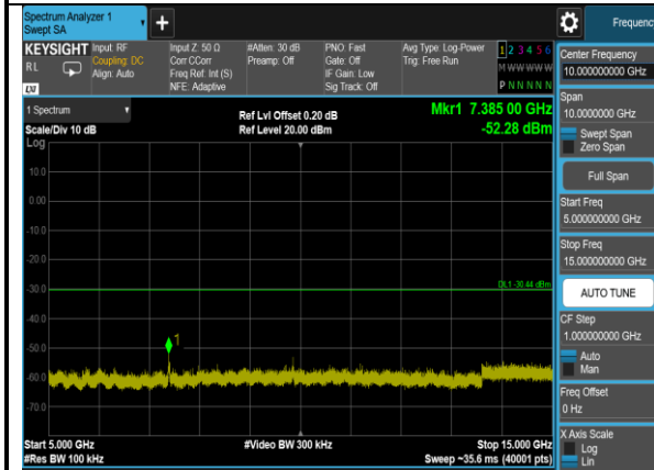
802.11n(HT20),2412MHz,Ant0,Plot 1,Reference Level
