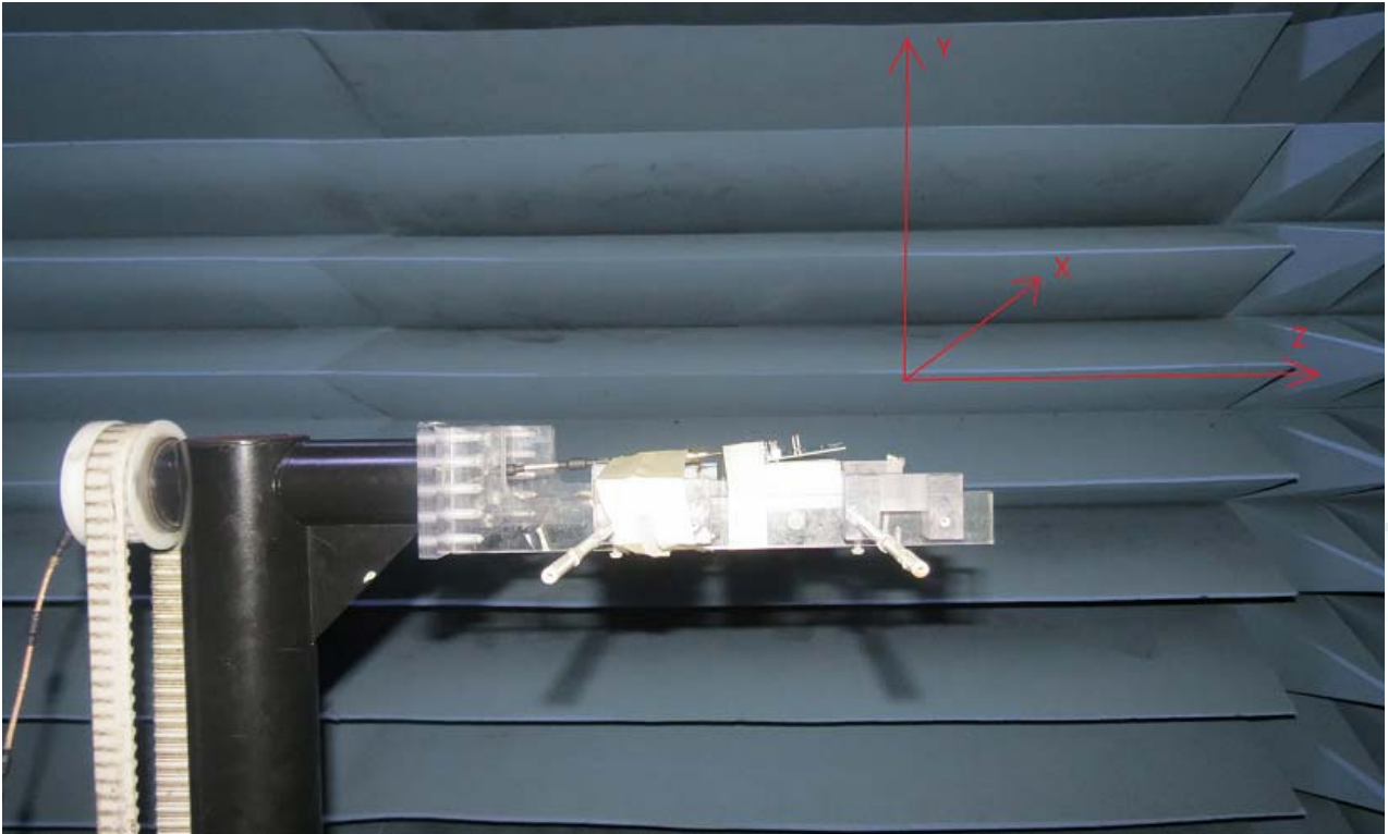
2.4G 3D Gain Picture 2 Test Setup *****END*****
