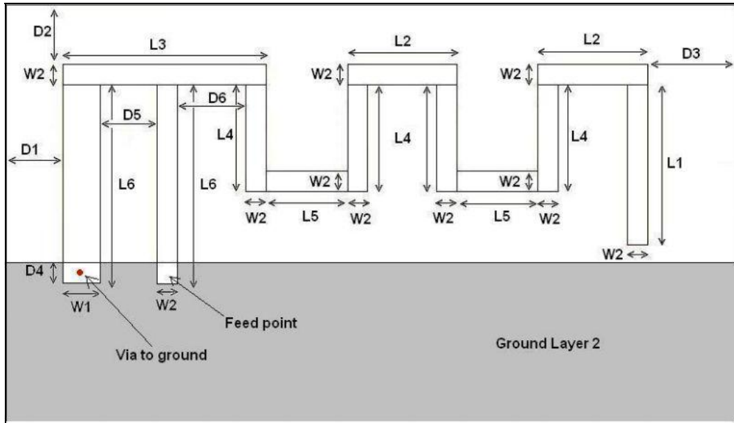
Figure 2: Antenna Dimensions
