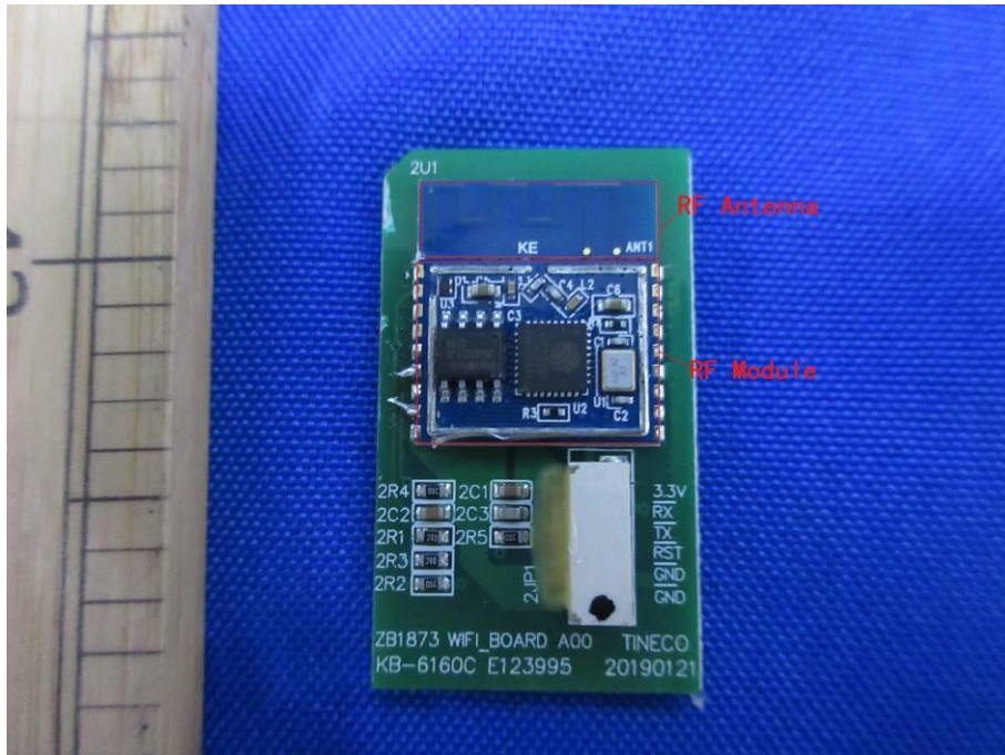
View of RF Module and Antenna location-2
