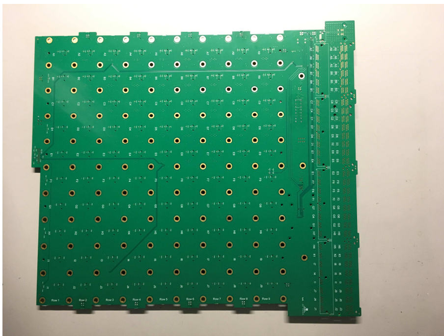
Nest Rack charging board - Carrier Bottom (used once per shelf)
