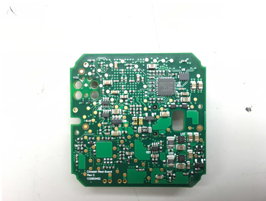
Nest Rack charging board - Nest Bottom (used 90 times per shelf)
