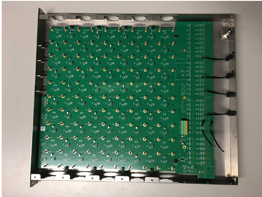
Nest Rack charging board - Carrier Top (used once per shelf)
