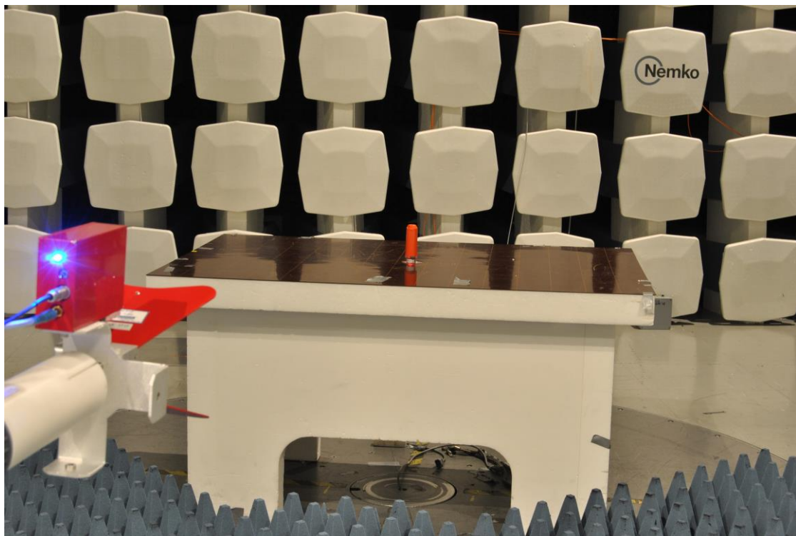
Radiated Emissions 1000 – 6000 MHz
