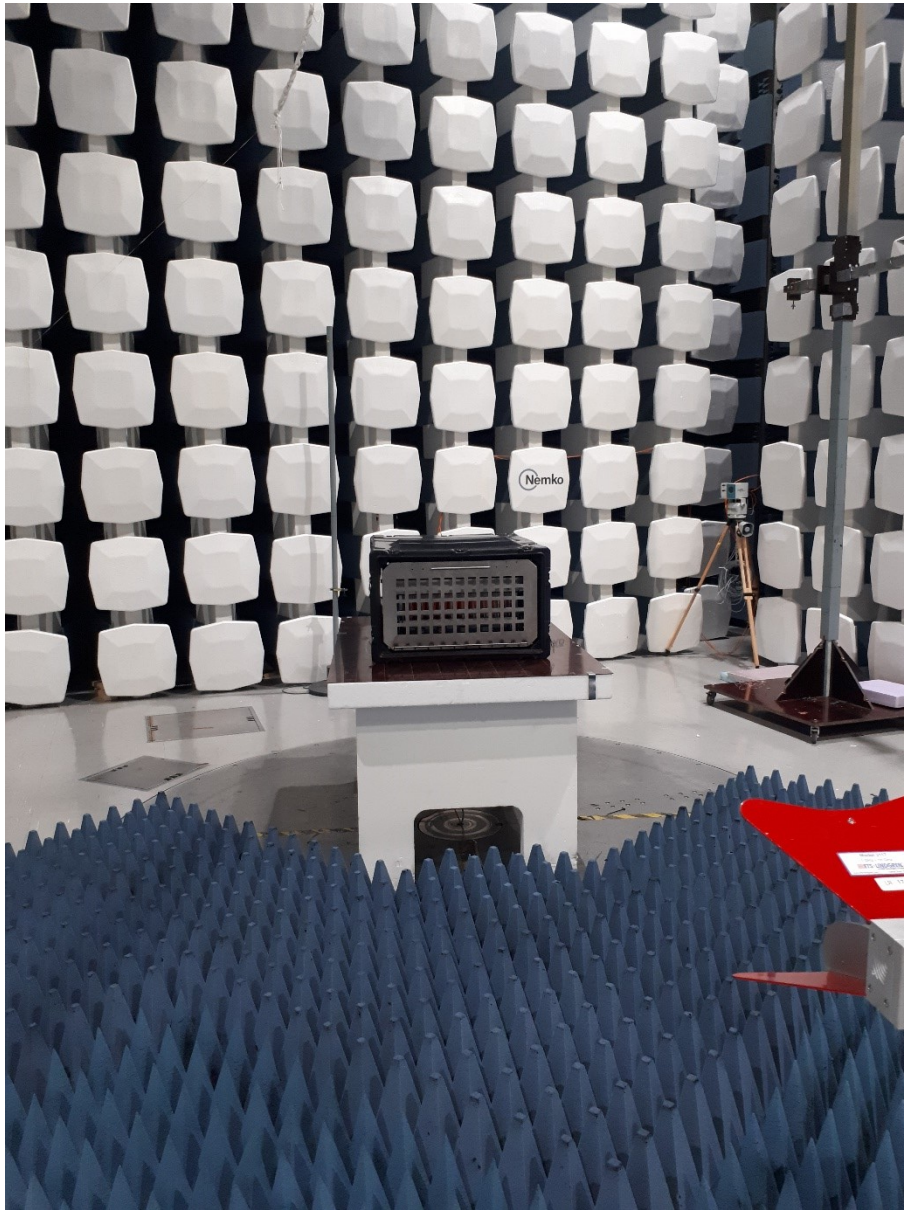
Radiated Emissions, 1000 – 6000 MHz
