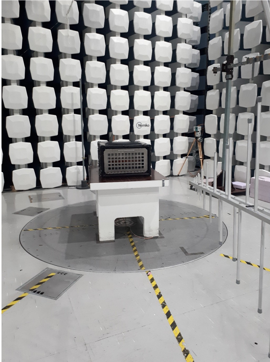
Radiated Emissions, 0.009 – 1000 MHz
