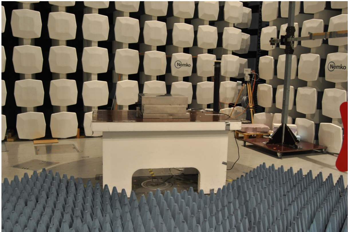
Radiated Emissions 1000 – 6000 MHz
