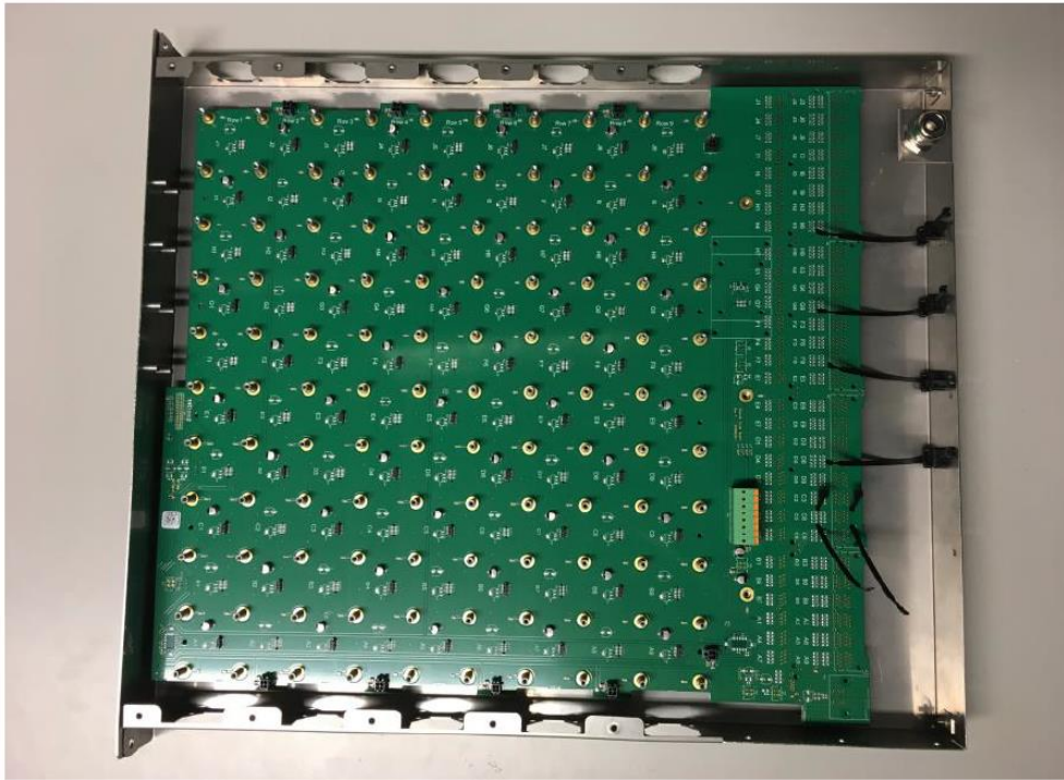
Figure 1: Initialisation Device Charger - Carrier Top
