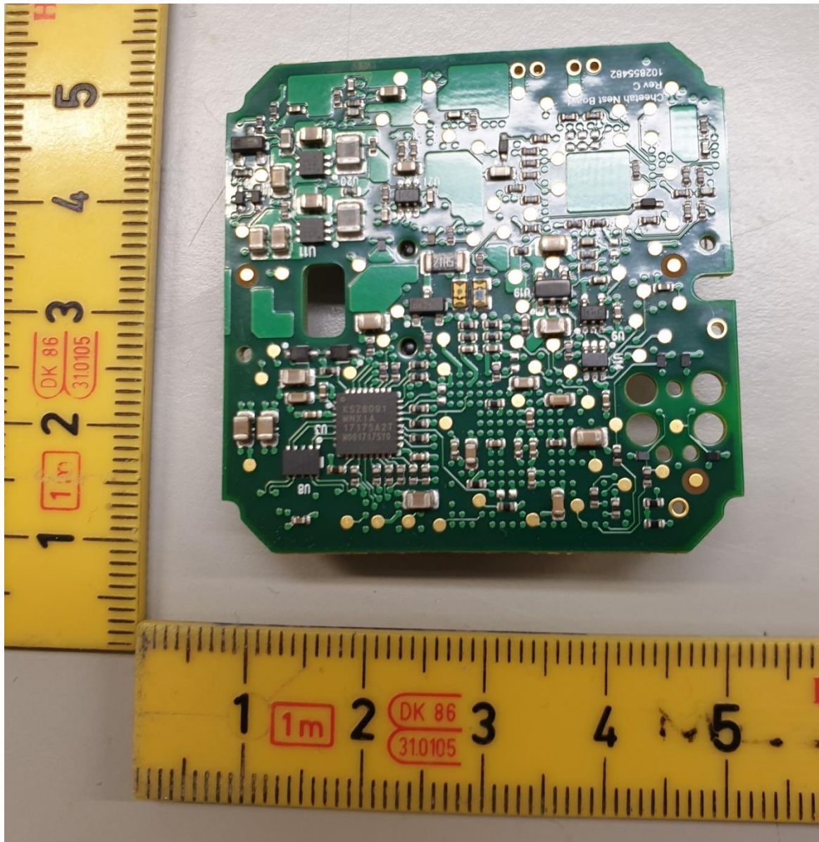
Figure 4: Nest Board bottom
