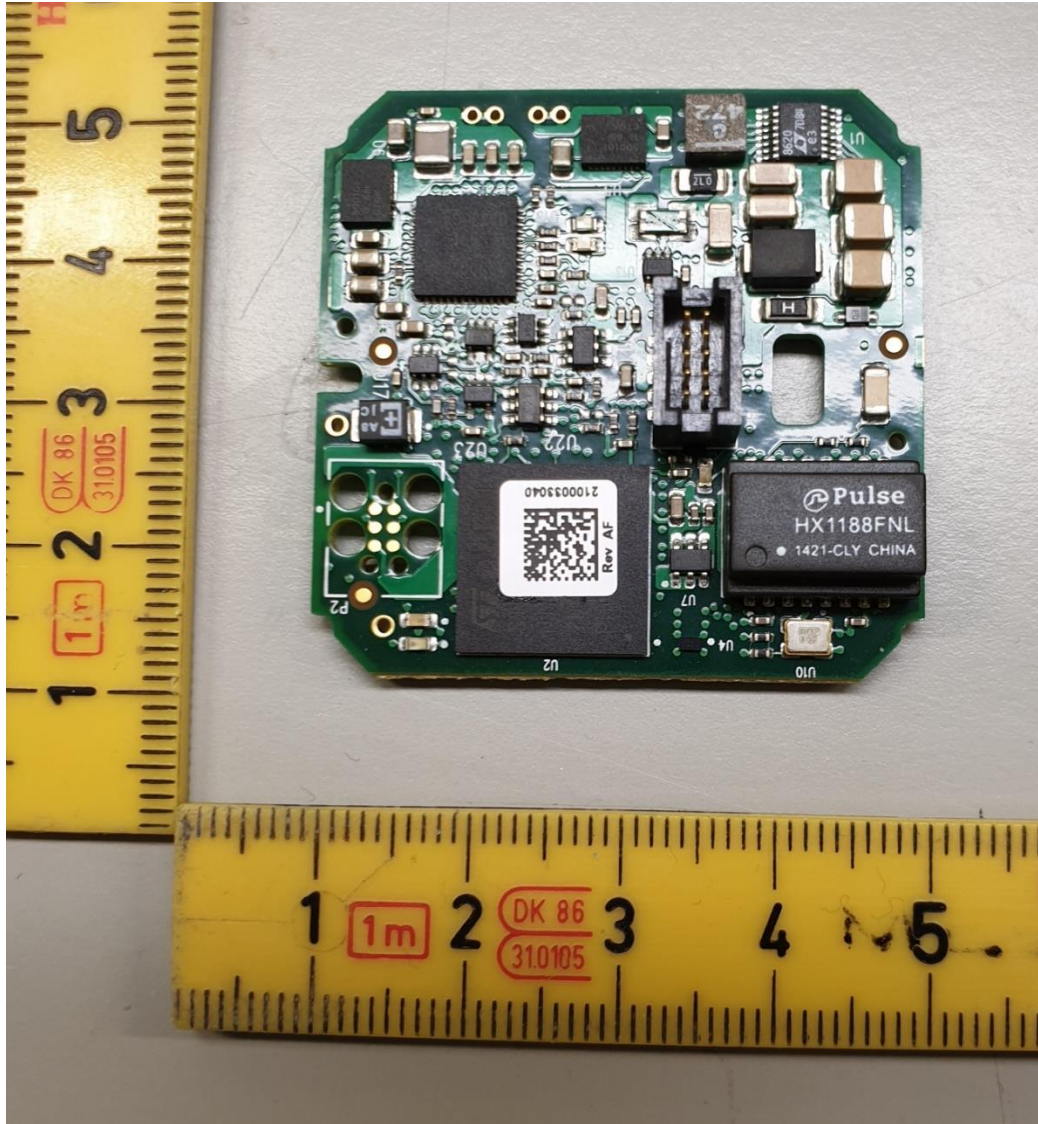
Figure 3: Nest Board top (used 45 times)
