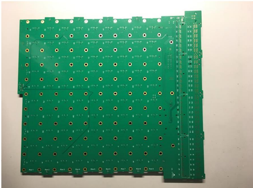
Figure 2: Initialisation Device Charger - Carrier Bottom
