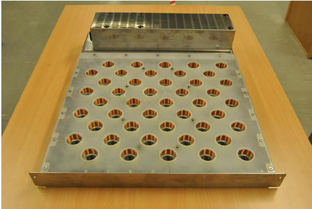
Init Device Charger - under the lid is the 45 charging loops
