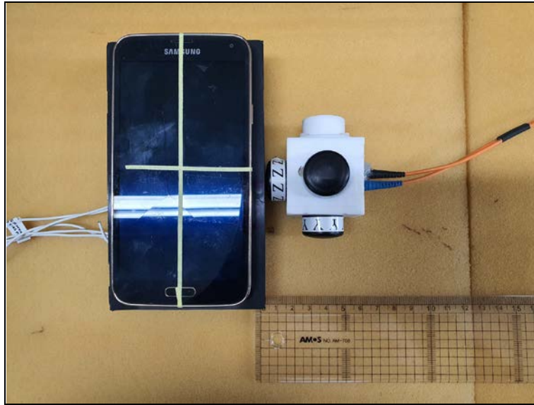
Photo of MPE Test Set up at 4 cm distance (E-field)
