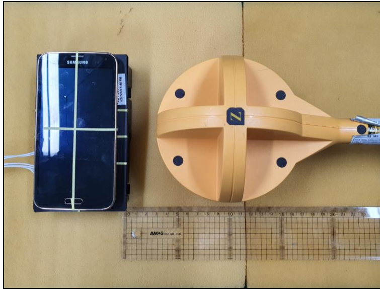
Photo of MPE Test Set up at 8 cm distance (H-field)
