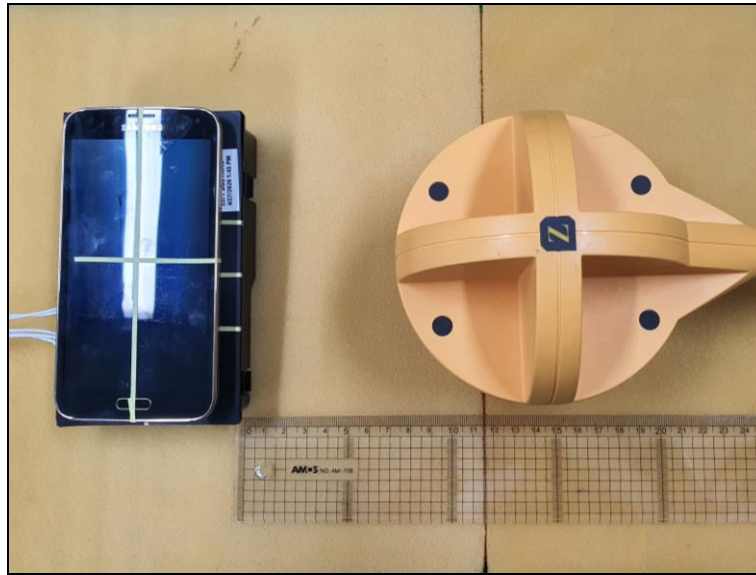
Photo of MPE Test Set up at 13 cm distance (H-field)
