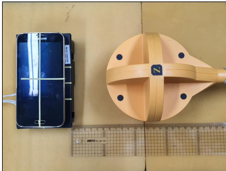
Photo of MPE Test Set up at 13 cm distance (H-field)
