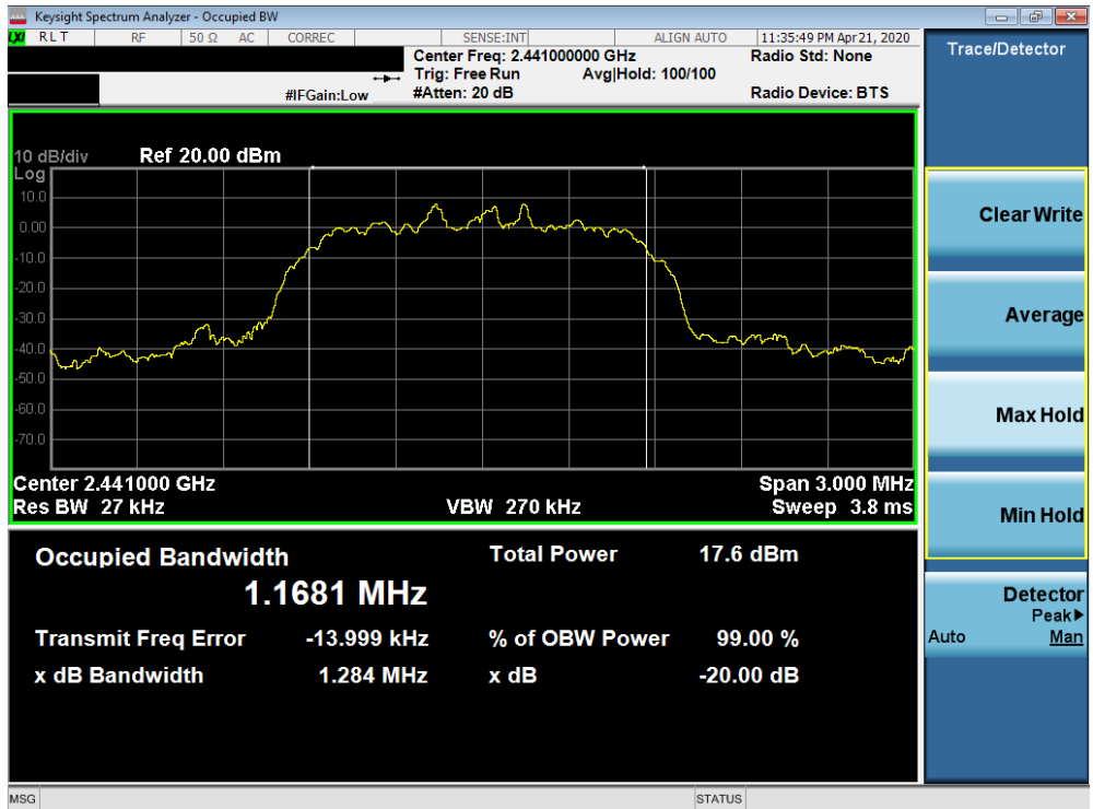
Plot 7-5. 20dB Bandwidth Plot (Bluetooth, 2Mbps – Ch. 39)
