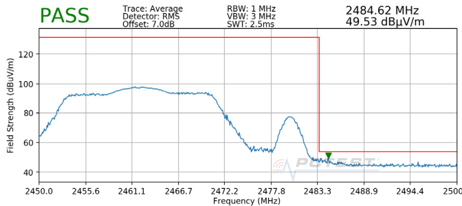
Plot 7-55. Radiated Restricted Upper Band Edge Measurement (Average)
