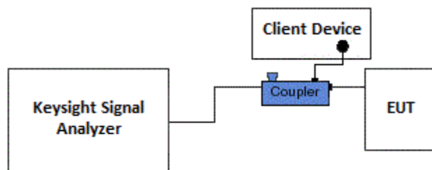
Figure 7-5. Test Instrument & Measurement Setup
