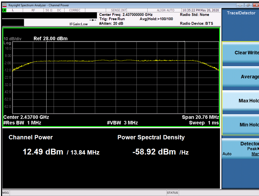
Plot 7-26. Peak Conducted Output Power Plot (802.11n (2.4GHz) – Ch. 6)
