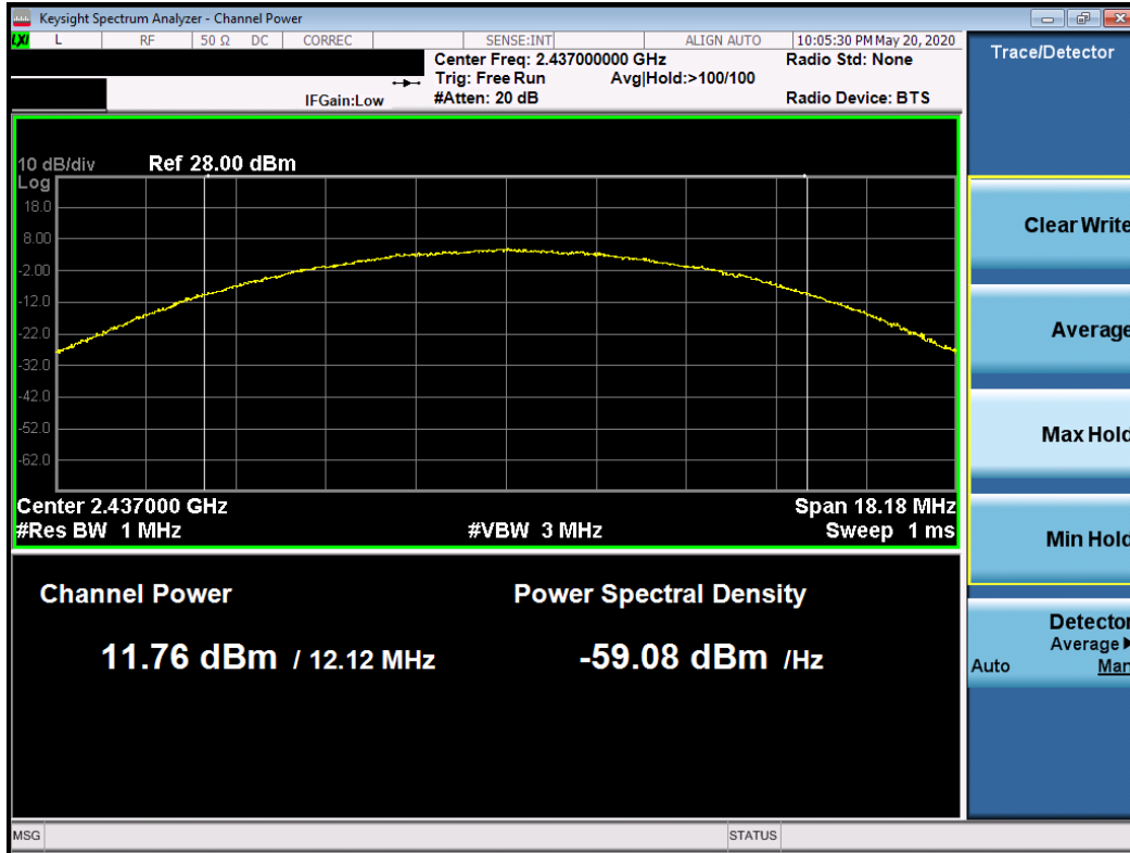
Plot 7-11. Average Conducted Output Power Plot (802.11b – Ch. 6)
