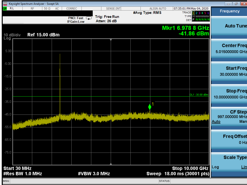
Plot 7-45. Conducted Spurious Plot (802.11b – Ch. 6)
