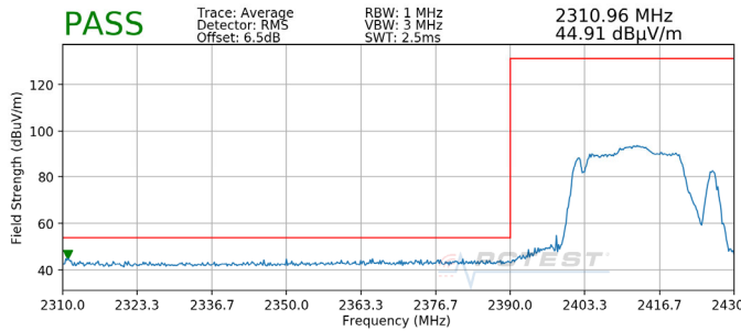
Plot 7-53. Radiated Restricted Lower Band Edge Measurement (Average)
