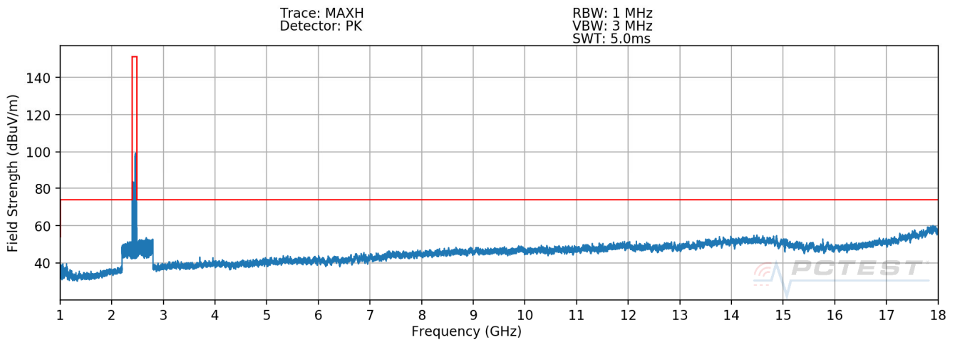
Plot 7-51. Radiated Spurious Plot above 1GHz (802.11b – Ch. 11)
