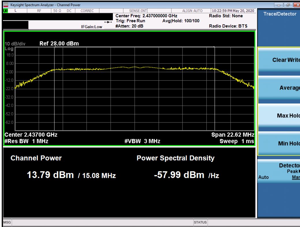
Plot 7-23. Peak Conducted Output Power Plot (802.11g – Ch. 6)
