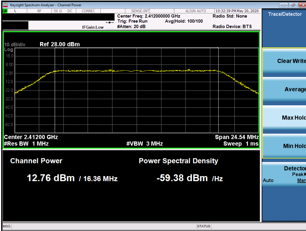
Plot 7-25. Peak Conducted Output Power Plot (802.11n (2.4GHz) – Ch. 1)
