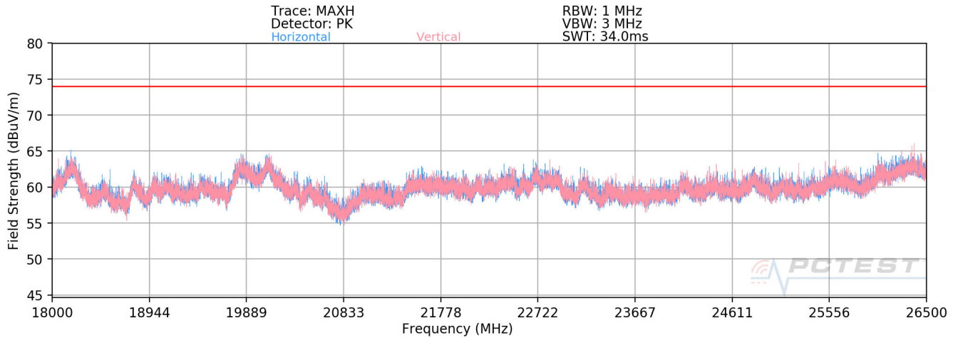
Plot 7-52. Radiated Spurious Plot above 18GHz ANT1
