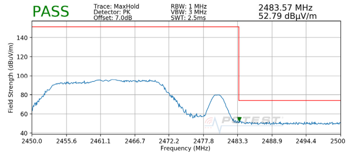
Plot 7-56. Radiated Restricted Upper Band Edge Measurement (Peak)
