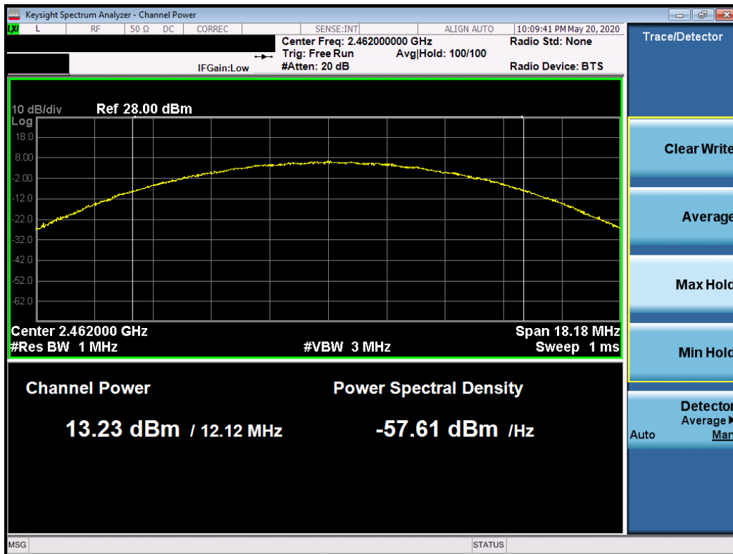
Plot 7-12. Average Conducted Output Power Plot (802.11b – Ch. 11)
