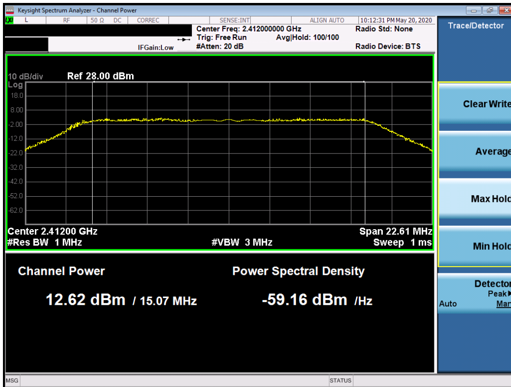
Plot 7-22. Peak Conducted Output Power Plot (802.11g – Ch. 1)
