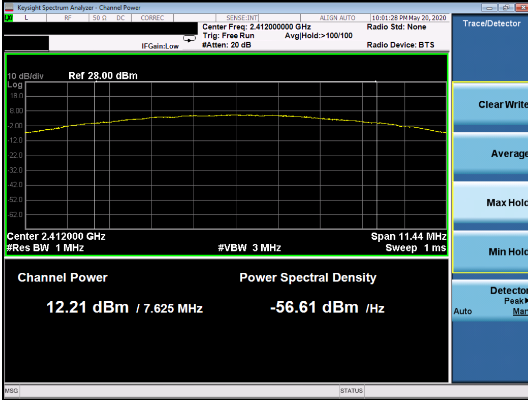
Plot 7-19. Peak Conducted Output Power Plot (802.11b – Ch. 1)
