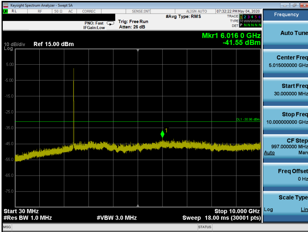
Plot 7-43. Conducted Spurious Plot (802.11b – Ch. 1)
