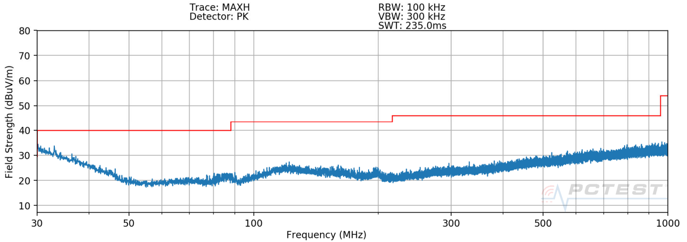
Plot 7-57. Radiated Spurious Plot below 1GHz ANT1
