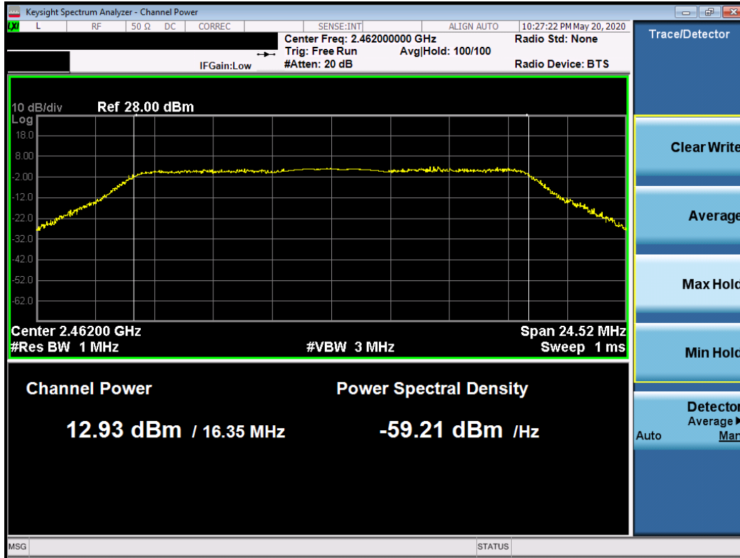
Plot 7-15. Average Conducted Output Power Plot (802.11g – Ch. 11)
