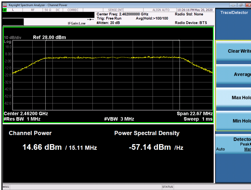
Plot 7-24. Peak Conducted Output Power Plot (802.11g – Ch. 11)
