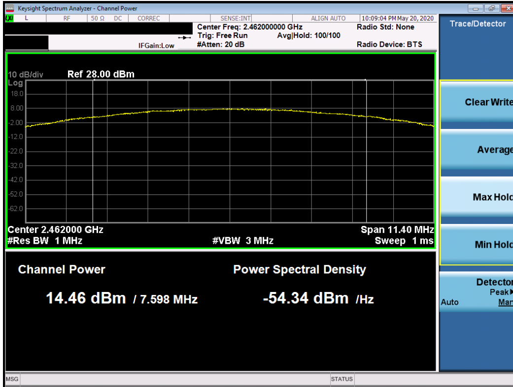
Plot 7-21. Peak Conducted Output Power Plot (802.11b – Ch. 11)
