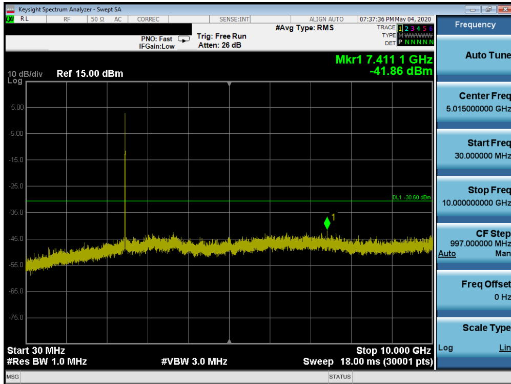
Plot 7-47. Conducted Spurious Plot (802.11b – Ch. 11)
