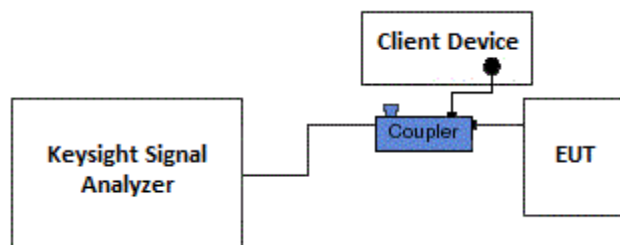
Figure 7-3. Test Instrument & Measurement Setup
