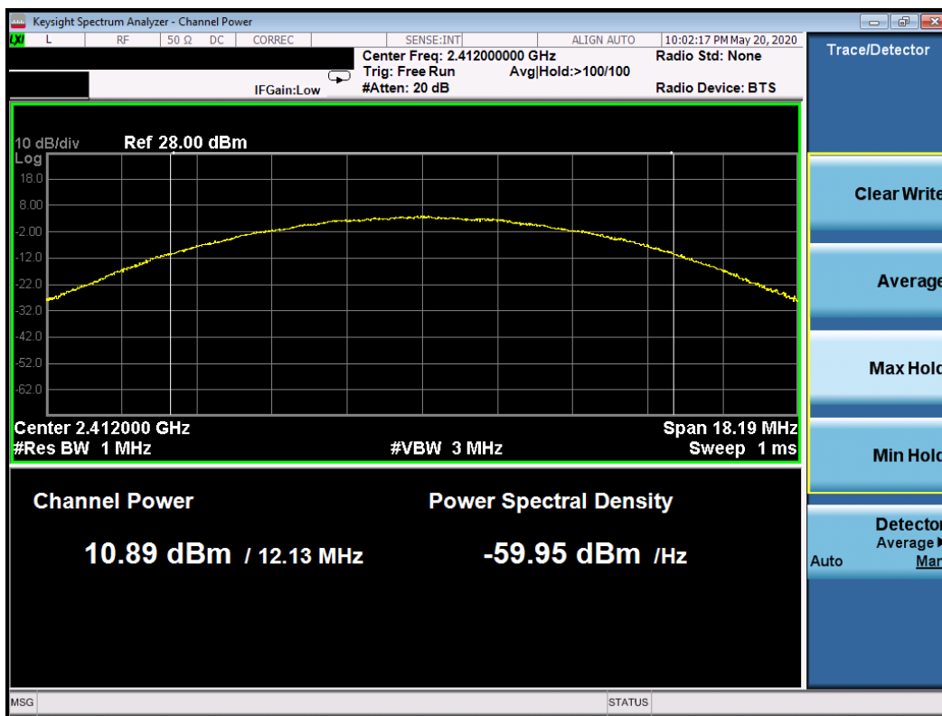
Plot 7-10. Average Conducted Output Power Plot (802.11b – Ch. 1)
