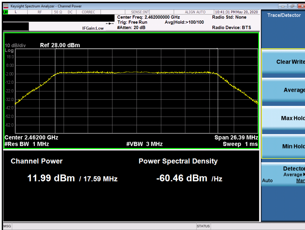
Plot 7-18. Average Conducted Output Power Plot (802.11n (2.4GHz) – Ch. 11)
