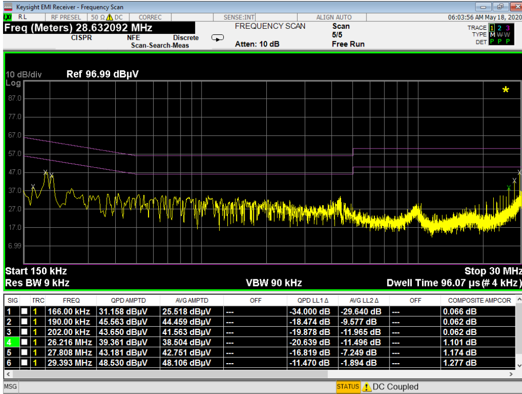
Plot 7-58. Line Conducted Plot with 802.11b (L1)
