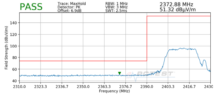
Plot 7-54. Radiated Restricted Lower Band Edge Measurement (Peak)
