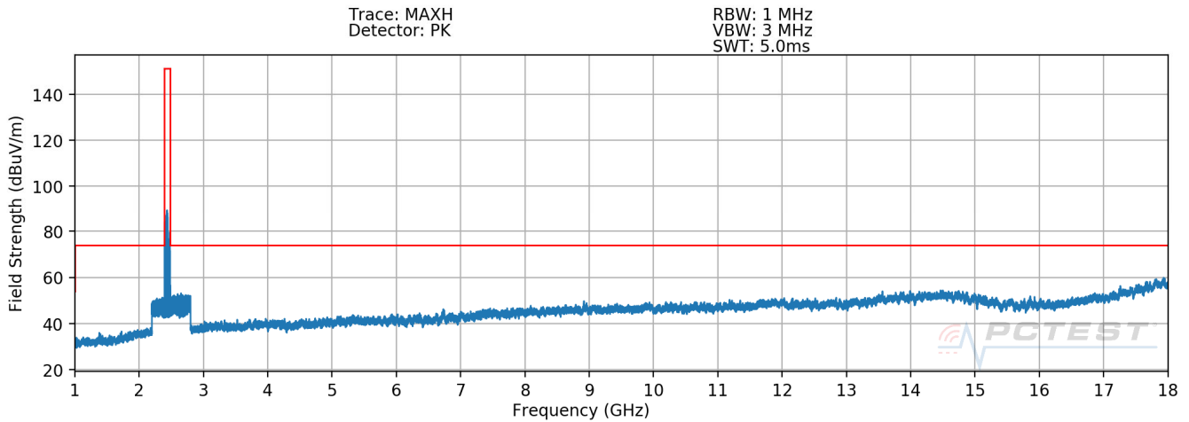
Plot 7-50. Radiated Spurious Plot above 1GHz (802.11b – Ch. 6)
