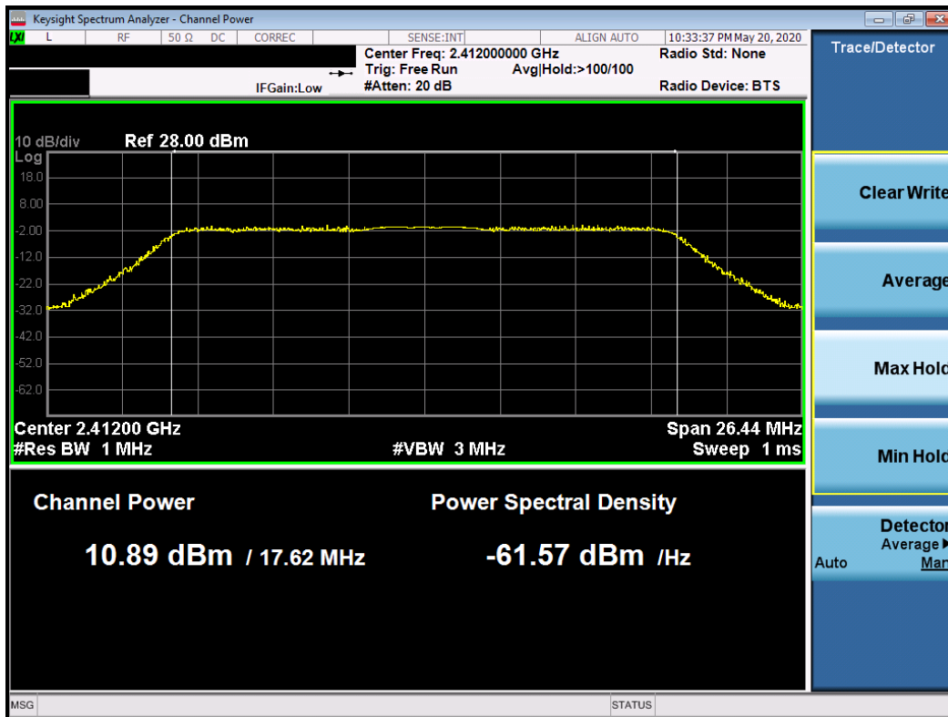
Plot 7-16. Average Conducted Output Power Plot (802.11n (2.4GHz) – Ch. 1)
