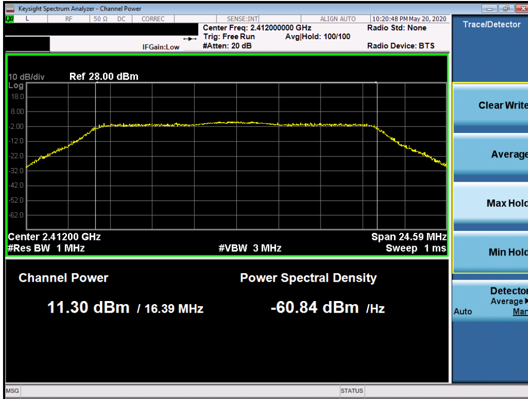
Plot 7-13. Average Conducted Output Power Plot (802.11g – Ch. 1)
