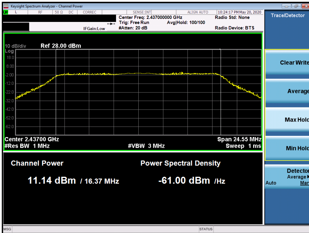
Plot 7-14. Average Conducted Output Power Plot (802.11g – Ch. 6)
