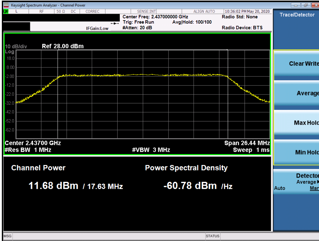
Plot 7-17. Average Conducted Output Power Plot (802.11n (2.4GHz) – Ch. 6)
