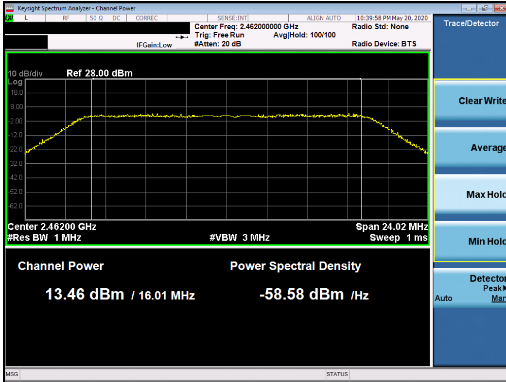
Plot 7-27. Peak Conducted Output Power Plot (802.11n (2.4GHz) – Ch. 11)
