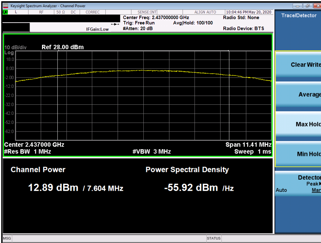
Plot 7-20. Peak Conducted Output Power Plot (802.11b – Ch. 6)
