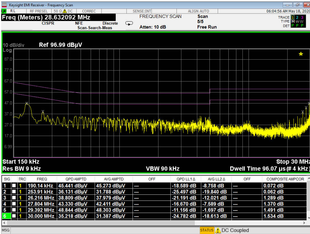
Plot 7-59. Line Conducted Plot with 802.11b (N)
