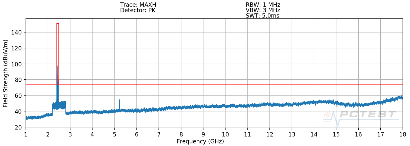
Plot 7-49. Radiated Spurious Plot above 1GHz (802.11b – Ch. 1)
