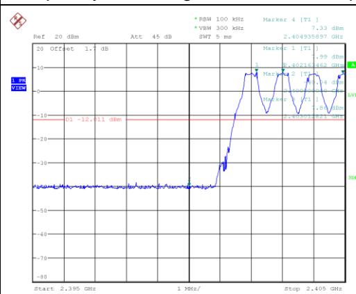
Frequency Band Edge: GFSK, Ch0, Hopping ON
