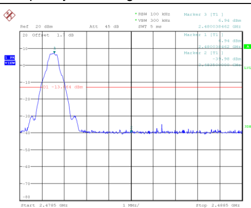
Frequency Band Edge: GFSK, Ch78, Hopping OFF
