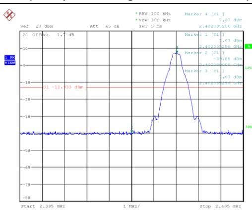
Frequency Band Edge: GFSK, Ch0, Hopping OFF
