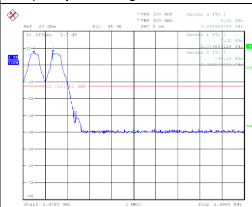
Frequency Band Edge: GFSK, Ch78, Hopping ON
