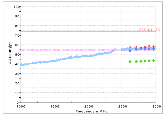
Bandedge (Low): 8DPSK, low channel
