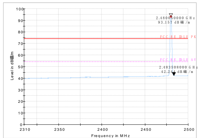
Bandedge (High): \pi/4 DQPSK, high channel
