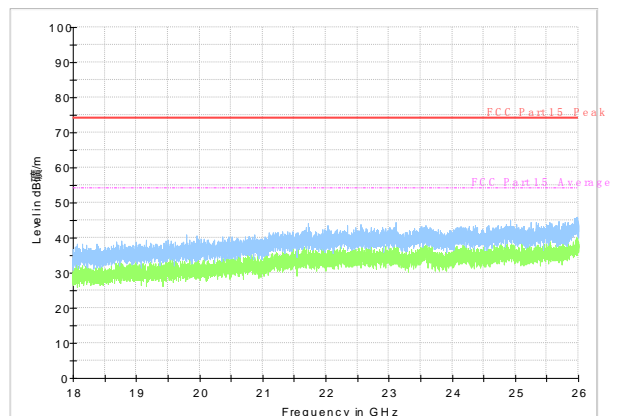
ALL Channel 18GHz~26GHz
