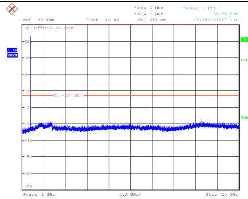
Channel 1512: 1GHz~20GHz
