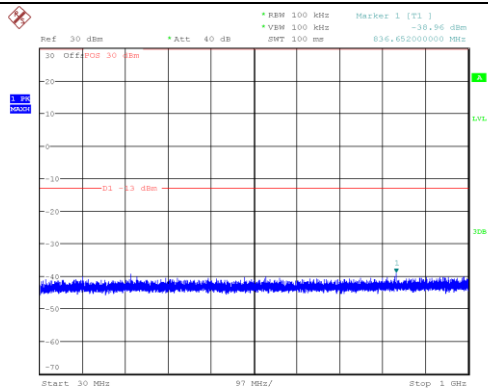
Channel 1512: 30MHz~1GHz
