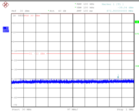
Channel 9400: 30MHz~1GHz
