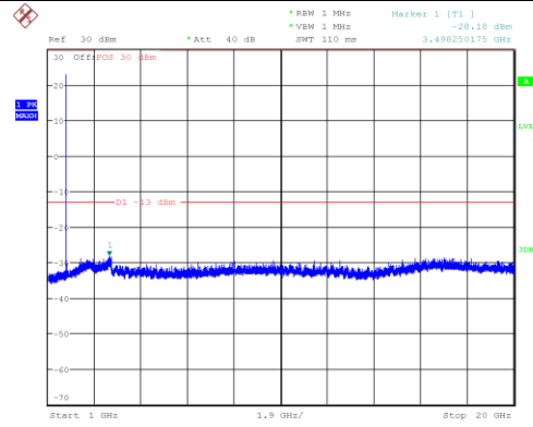
Channel 1312: 1GHz~20GHz
