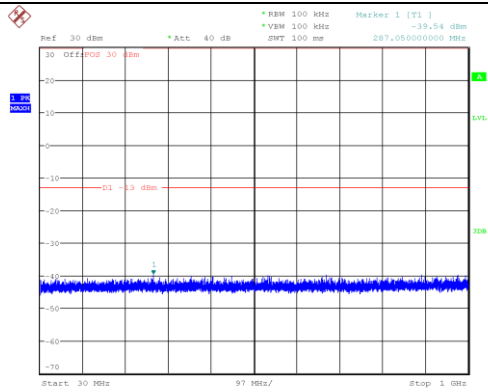
Channel 1450: 30MHz~1GHz
