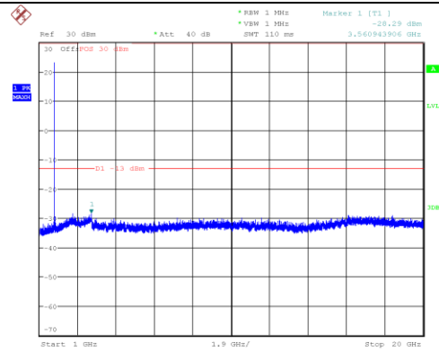
Channel 1450: 1GHz~20GHz
