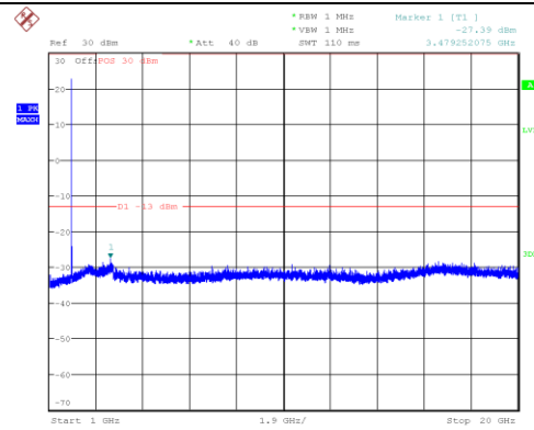
Channel 9538: 1GHz~20GHz
