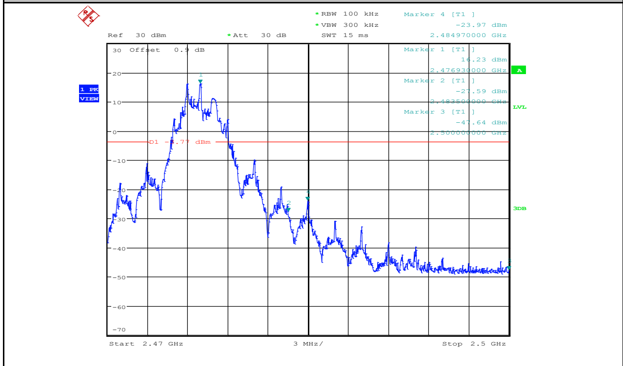
Band-edge for RF Conducted Emissions_2.4G_2477_Hopping Off
