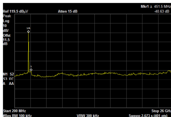
Spurious Conducted Emissions, N mode, 20MHz, High 2462
