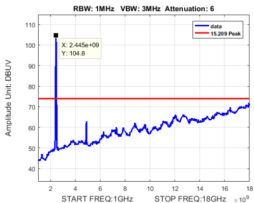
Radiated Spurious Emissions, N mode, 20MHz, Mid 2437, Peak
