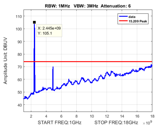
Radiated Spurious Emissions, B mode, 20MHz, Mid 2437, Peak
