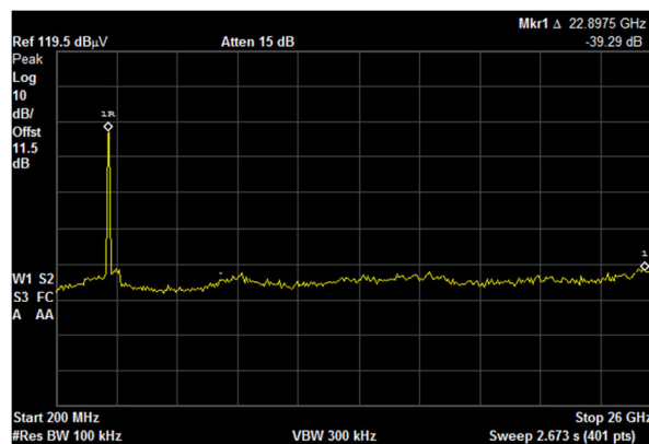
Spurious Conducted Emissions, N mode, 40MHz, Low 2422
