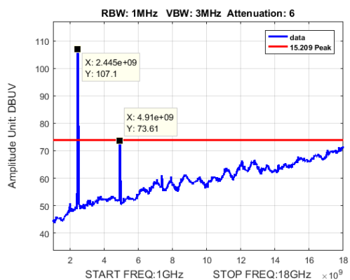
Radiated Spurious Emissions, B mode, 20MHz, High 2462, Peak
