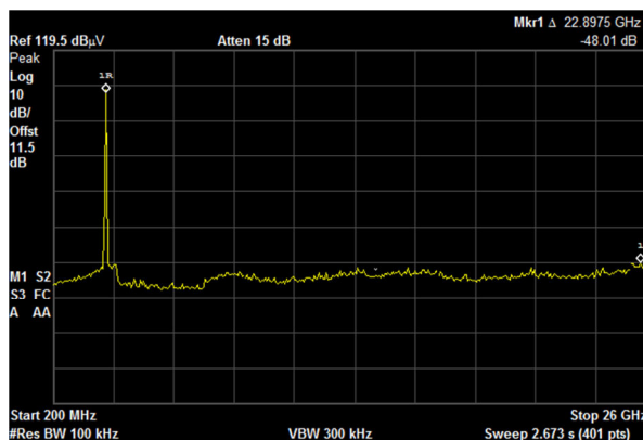
Spurious Conducted Emissions, N mode, 20MHz, Mid 2437
