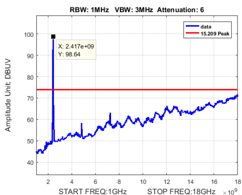
Radiated Spurious Emissions, B mode, 20MHz, Low 2412, Peak
