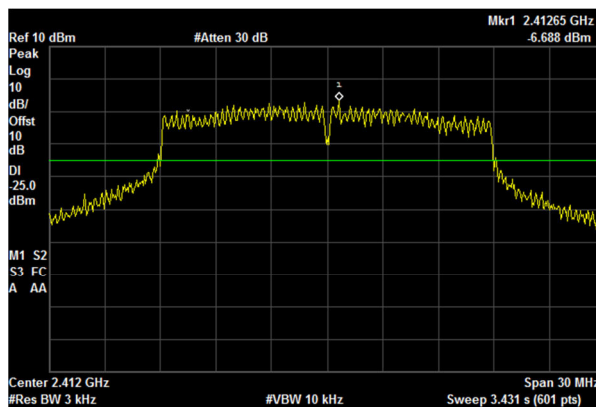
Peak Spectral Density, N mode, 20MHz, Low 2412
