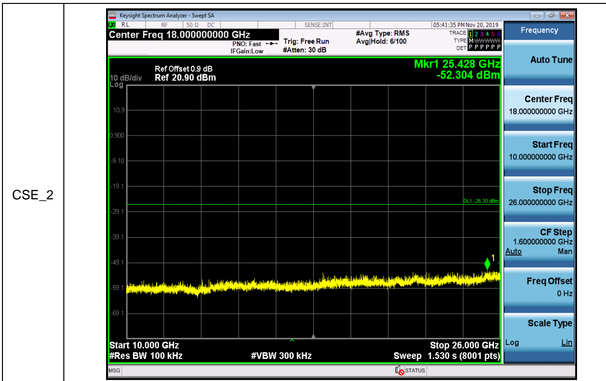
RF Conducted Spurious Emissions_11N40ISO_2422_Ant1
