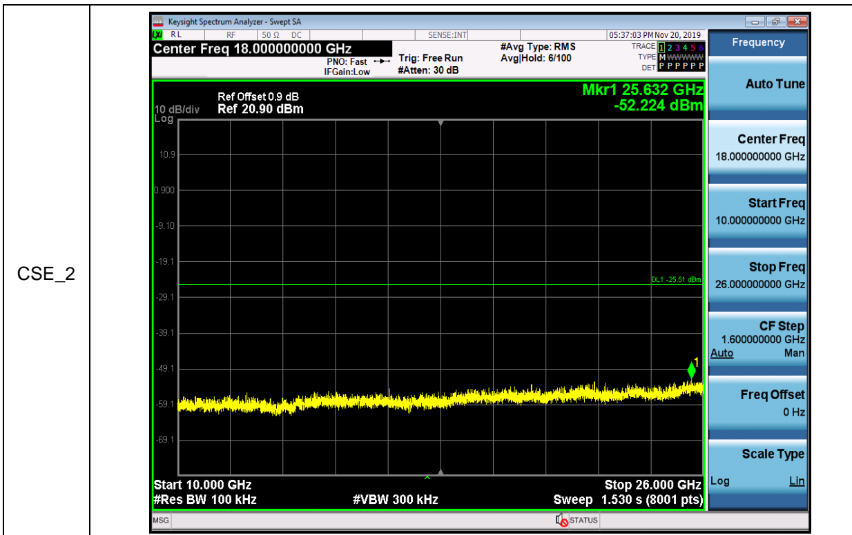
RF Conducted Spurious Emissions_11N20SISO_2442_Ant1
