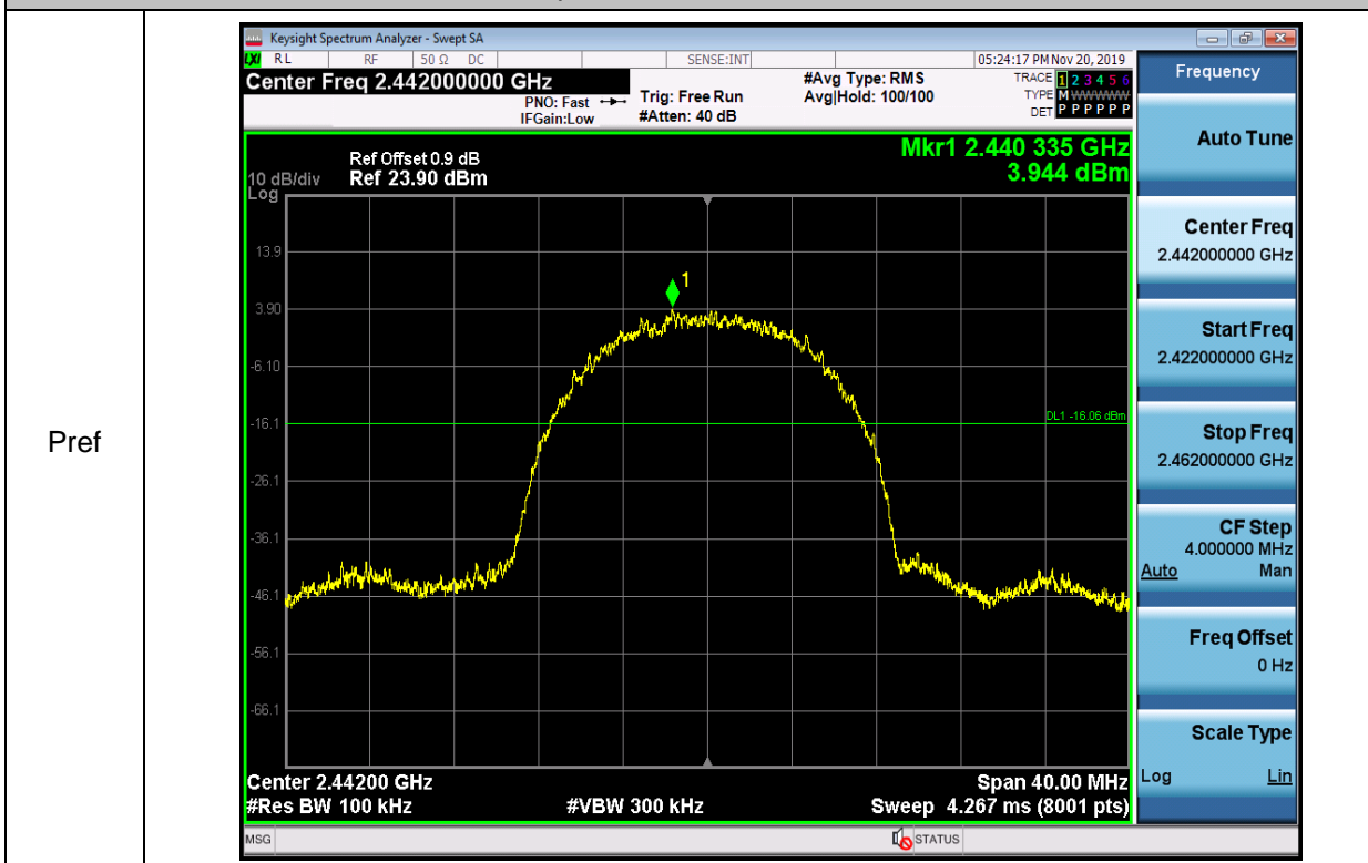
RF Conducted Spurious Emissions_11B_2442_Ant1
