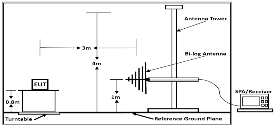
Below 1GHz
